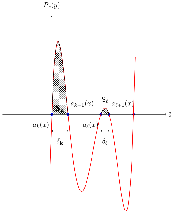
Figure 1.41: For any k \neq l , \delta_k \succ_+ \delta_\ell implies S_k \succ_+ S_\ell .
