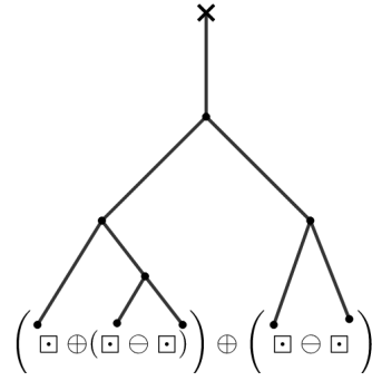
Figure 4.14: A binary separating tree s_1 of \sigma .
