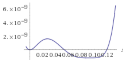
Figure 1.53: The graph of Q_x(y) for x > 0 small enough: the snake associated to Q_x(y) is \sigma .
