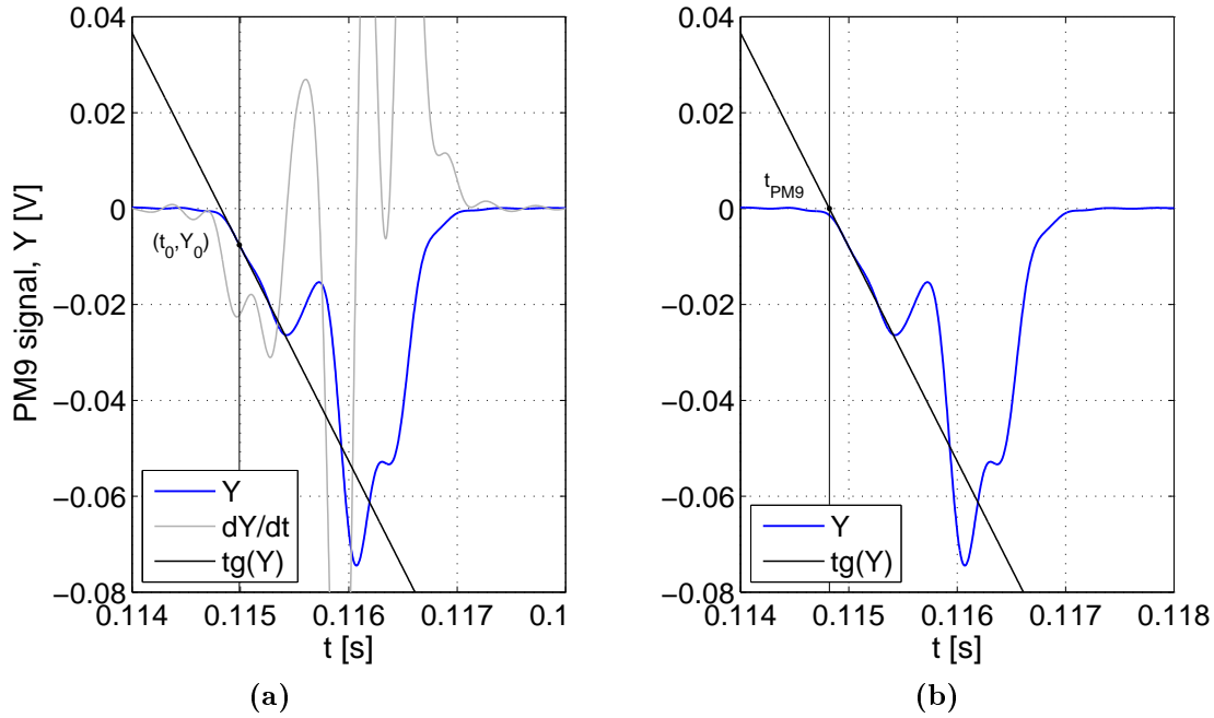
Figure 8.4: Graphic representation of the method used to evaluate the flame time-of-arrival for PMT9. f_c = 3200 Hz.
