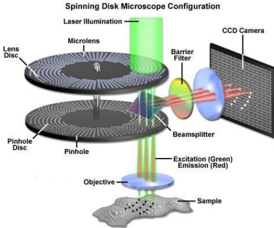
Figure 19: Spinning Disk Confocal Microscope configuration
