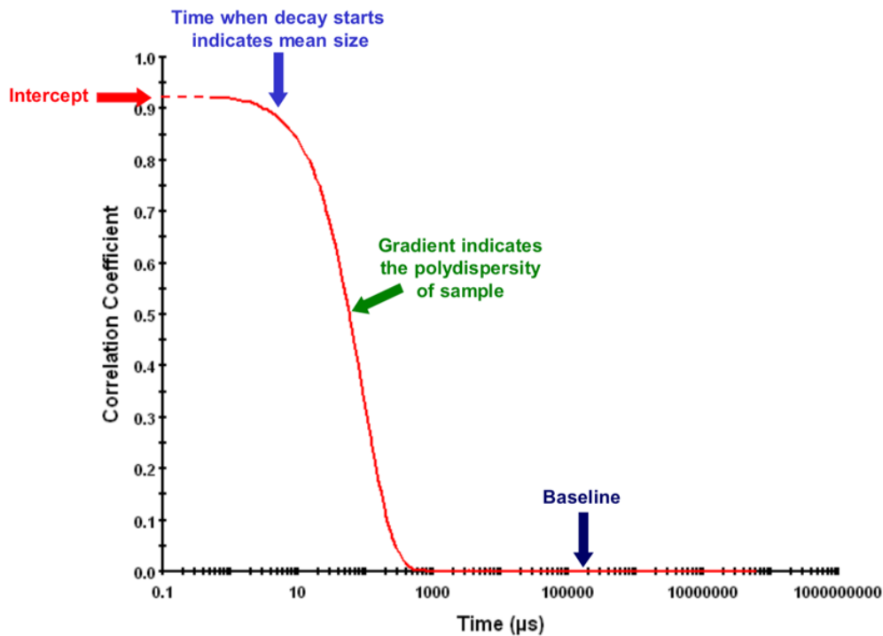
Figure B-2: Auto-correlation function description. From Malvern technical support datasheet
