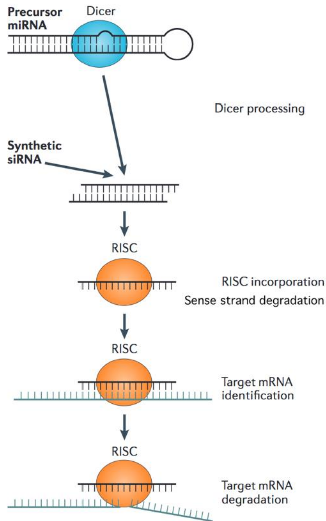
Figure 3.3-2: Gene silencing at post-transcriptional level using siRNA. dsRNA is first cleaved by Dicer to produce siRNA. In case of synthetic siRNA, this step is bypassed. siRNA then assembles with RISC. The sense strand of siRNA is degraded, and the antisense strand is used to guide RISC to the targeted mRNA and cleave it. siRNA and RISC are recycled to process other cleavage cycles. Adapted from Ref. [230]
