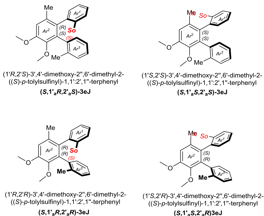
figureVII-38 : diastereomers of ( S,S )-3eM
