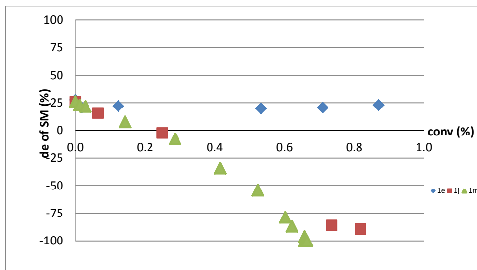
Figure V-17 : Variation of the diastereomeric excess of 1e , 1j and 1m as a function of conversion
