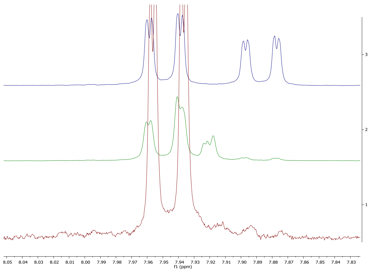
Figure VII-49 : top spectra : Step 3; middle spectra : Step 2; bottom spectra crude reaction mixture
