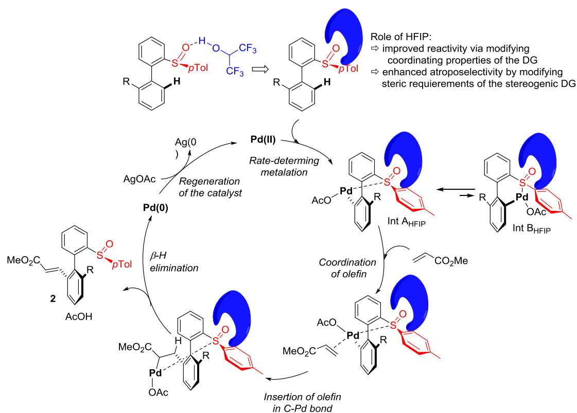
Figure IV-21 : Proposed catalytic cycle.
