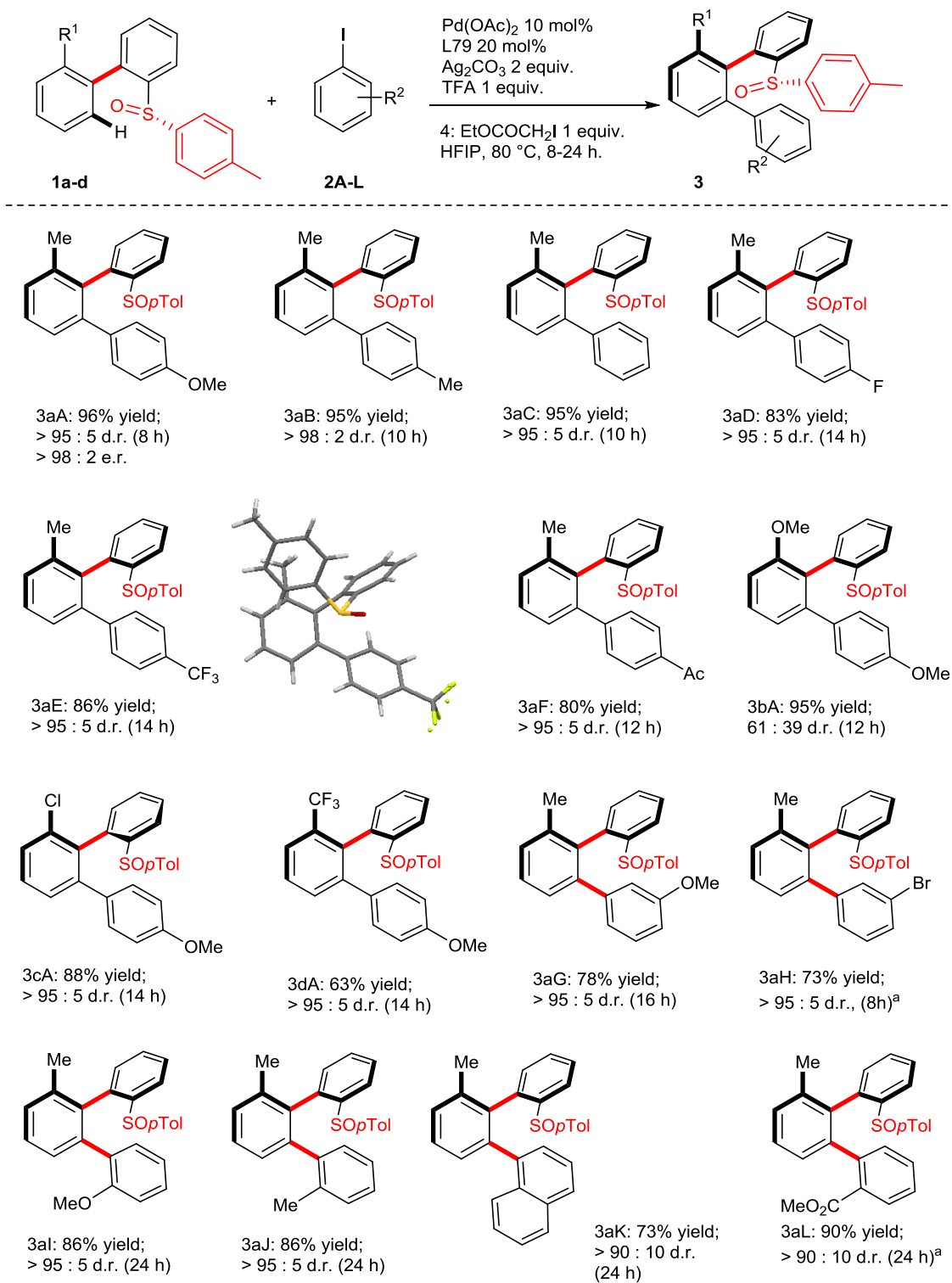
Figure VII-23 : Scope of direct arylation of biaryl sulfoxides 1a-1d.
