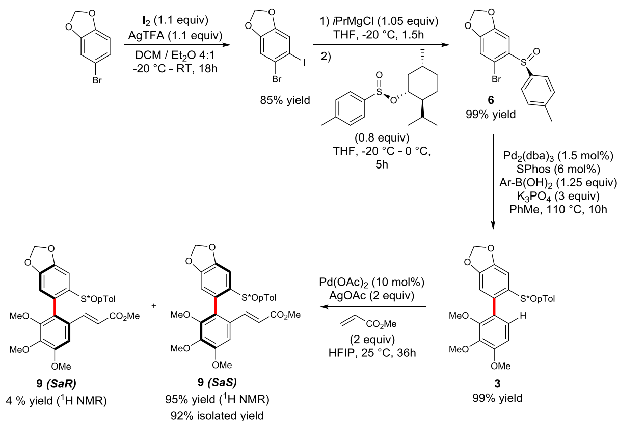
Figure VI-16 : synthesis of 9 with controlled axial chirality
