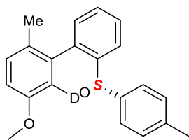
(S)-5-methoxy-2-methyl-2'-(p-tolylsulfinyl)-1,1'-biphenyl-6-d Chemical Formula: C 21 H 19 DO 2 S Molecular Weight: 337,4551
