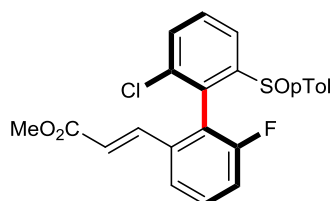
methyl ( E )-3-(( aR )-2'-chloro-6-fluoro-6'-(( S )- p -tolylsulfinyl)-[1,1'-biphenyl]-2-yl)acrylate Chemical Formula: C 23 H 18 ClFO 3 S Molecular Weight: 428,9024
