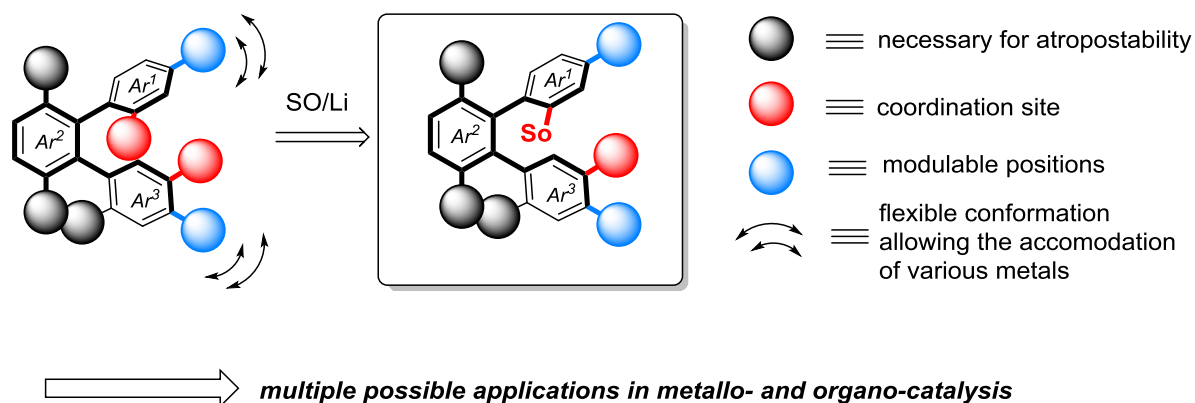
Figure VII-13 : stereogenic multi-functional bidentate scaffold
