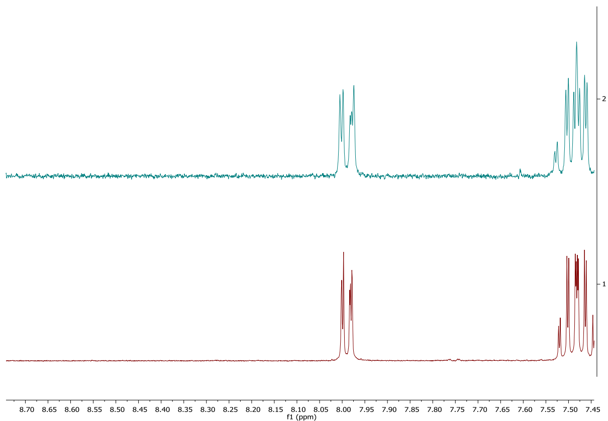
Figure VII-42 : Study of the thermal stability of \text{Ar}^1\text{-Ar}^2 axis of 3aA
