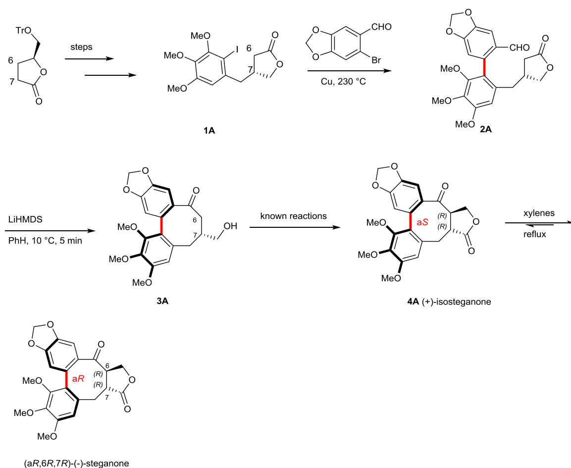
Figure VI-5 : first asymmetric synthesis
