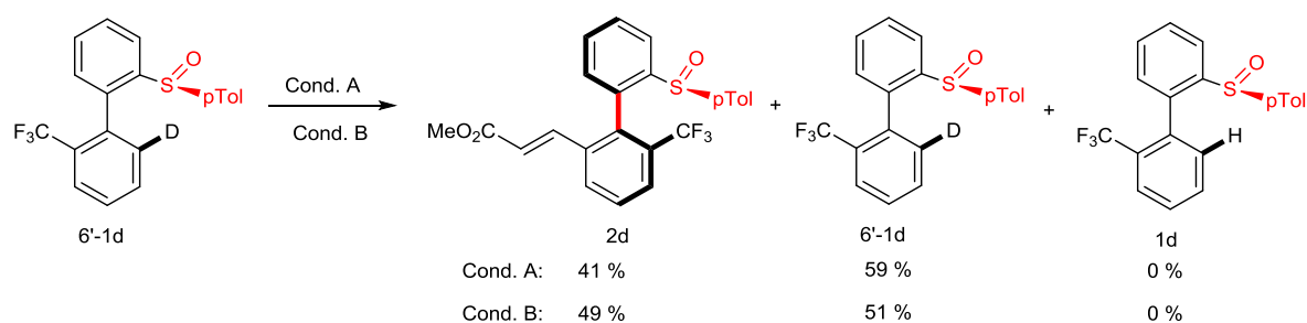
Figure IV-19 : reversibility study.
