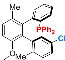
((1'R,2'S)-5''-chloro-3'-methoxy-2'',6'-dimethyl-[1,1':2',1''-terphenyl]-2-yl)diphenylphosphane C 33 H 28 ClOP 507,0098
