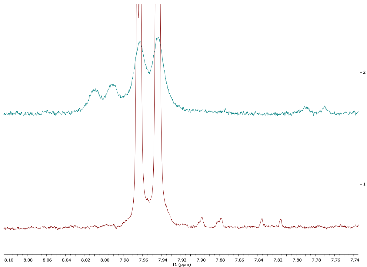
Figure VII-55 :thermal epimerization of 3fU; Top spectra : thermal epimerization ; Bottom spectra : crude reaction mixture
