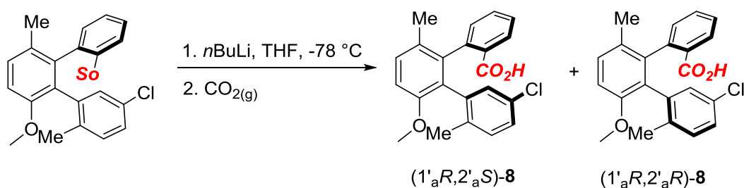
FigureVII-60 : functionalization of epimerized 3fP
