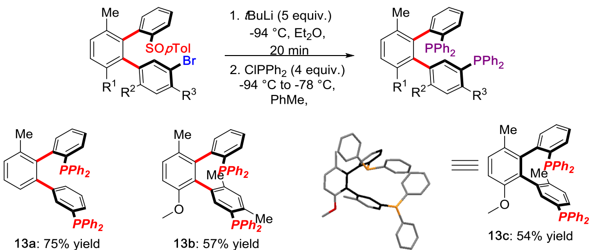
Figure VII-30 : Post-functionalization of terphenyl scaffolds.
