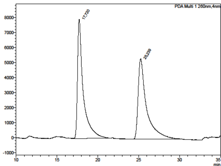
<PDA Chromatogram>
