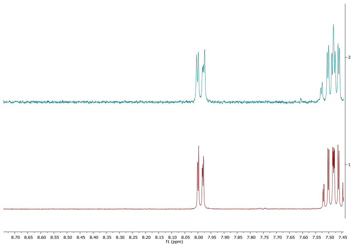
Figure VII-42 : Study of the thermal stability of Ar 1 -Ar 2 axis of 3aA
