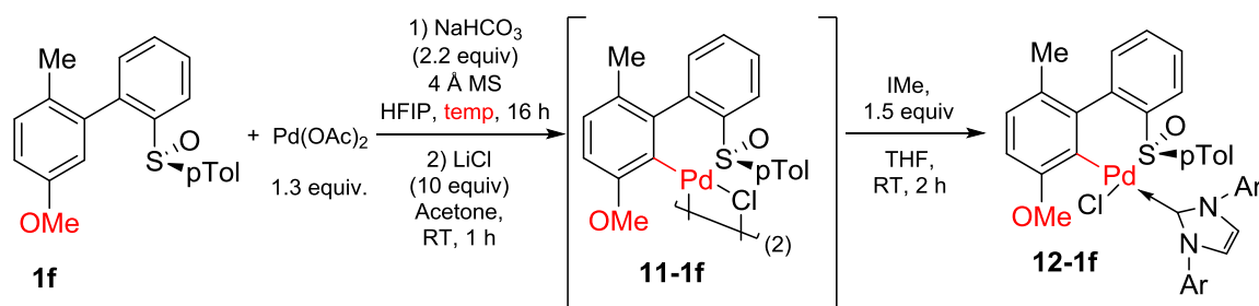
figureVII-77: attempt of isolation of 1f palladacycle in standard conditions
