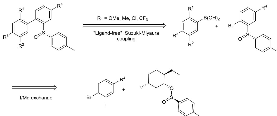
Figure VIII-1 : retrosynthetic scheme
