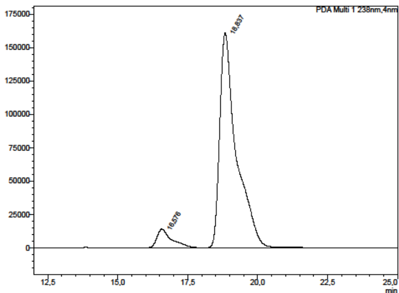
<PDA Chromatogram>
