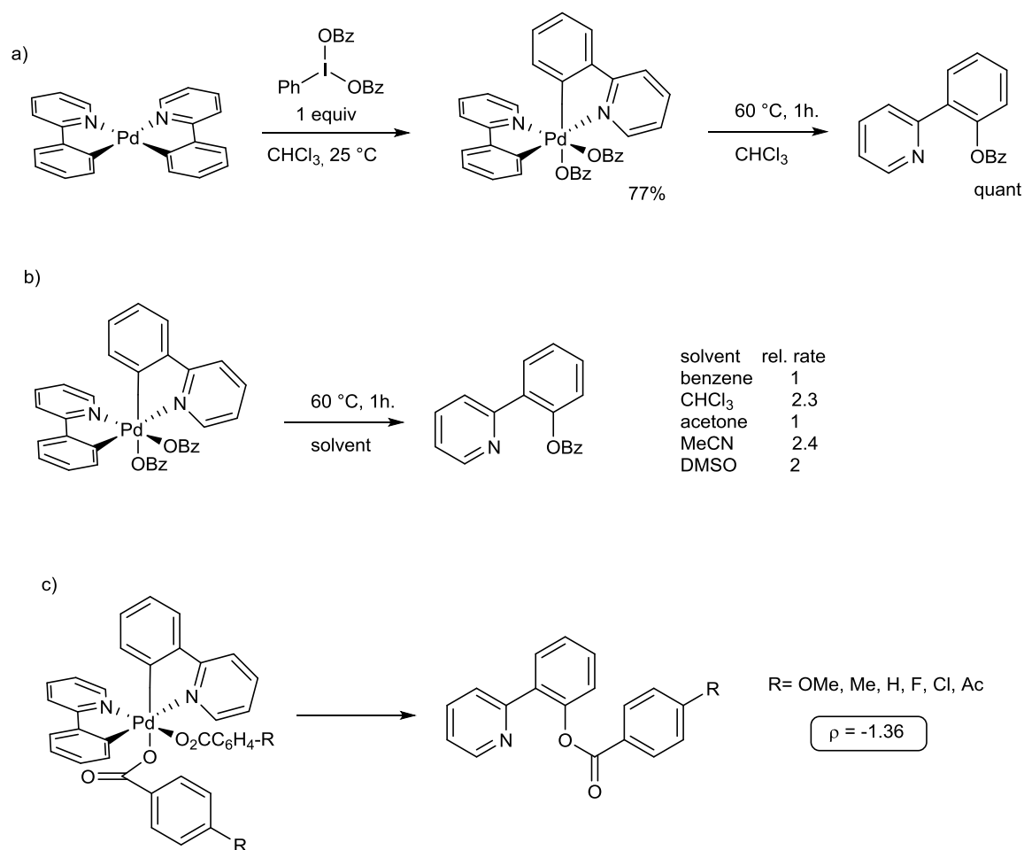
Figure V-12 : reductive elimination from Pd IV complexes
