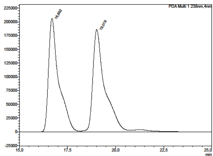
<PDA Chromatogram>
