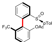
( R )-2'-(( S )- p -tolylsulfinyl)-6-(trifluoromethyl)-[1,1'-biphenyl]-2-yl acetate Chemical Formula: C 22 H 17 F 3 O 3 S Molecular Weight: 418,4302
