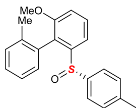
2-methoxy-2'-methyl-6-((S)-p-tolylsulfinyl)-1,1'-biphenyl
