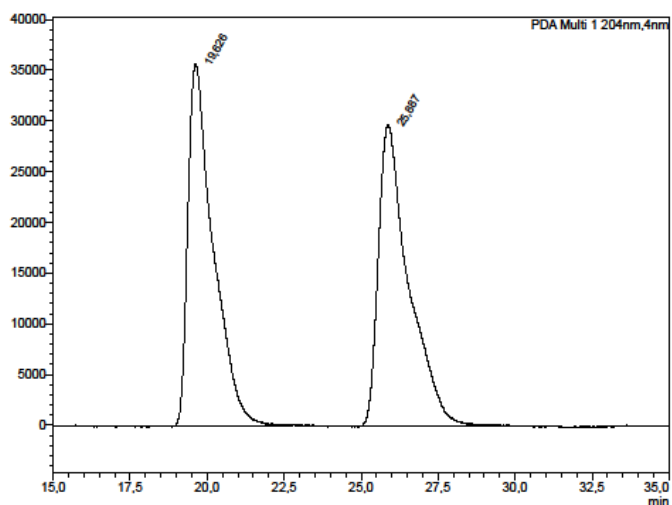
<PDA Chromatogram>
