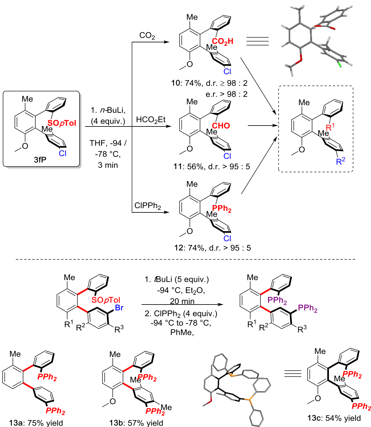
Figure VII-30 : Post-functionalization of terphenyl scaffolds.
