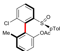
( S )-2'-chloro-6-methyl-6'-(( S )- p -tolylsulfinyl)-[1,1'-biphenyl]-2-yl acetate Chemical Formula: C 22 H 16 ClO 3 S Molecular Weight: 398,9010
