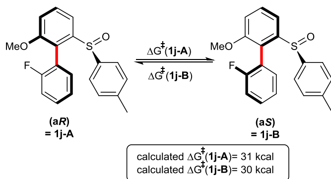
Figure V-23 : 1j rotation barrier
