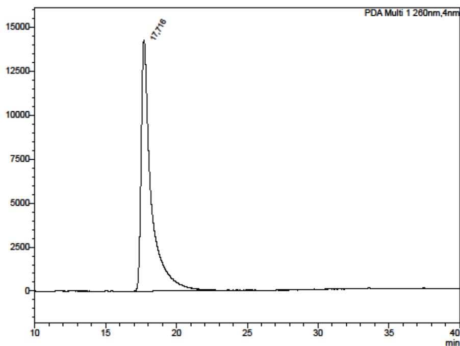
<PDA Chromatogram>
