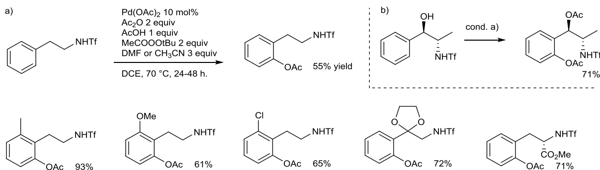
Figure V-6 : other DG for the acetoxylation reaction
