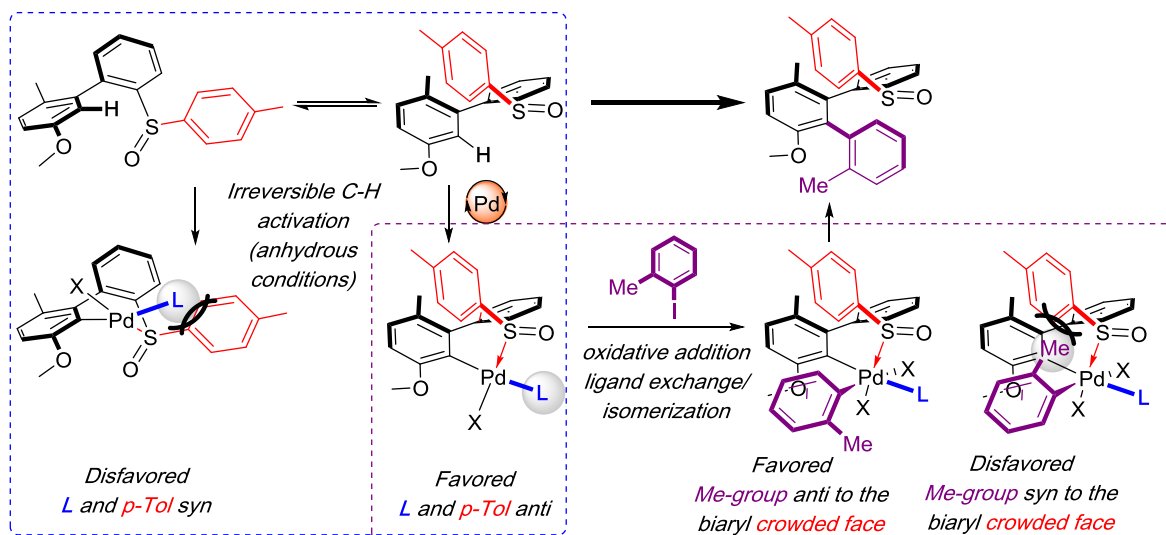
Figure VII-28 : stereinduction model
