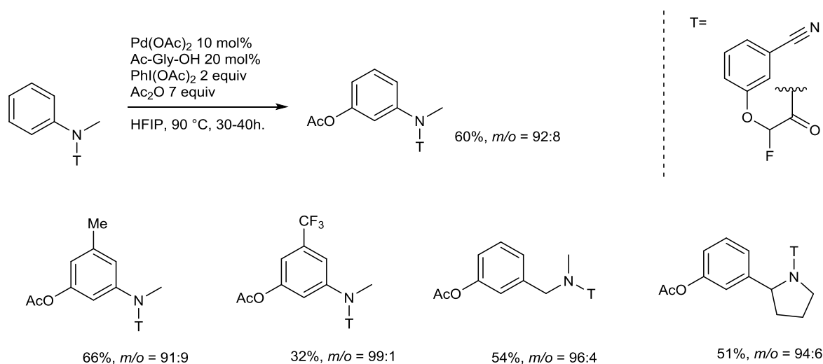
Figure V-7 meta-selective acetoxylation
