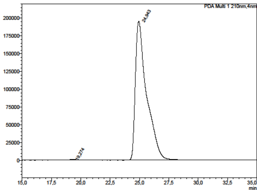
<PDA Chromatogram>
