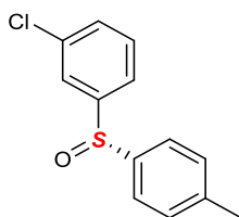
(S)-1-chloro-3-(p-tolylsulfinyl)benzene Chemical Formula: C 13 H 11 ClOS Molecular Weight: 250.7400
