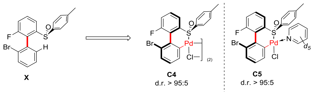
Figure V-25 : literature precedent of biphenylsulfoxide palladacycles
