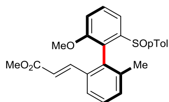
methyl ( E )-3-(( aR )-2'-methoxy-6-methyl-6'-(( S )- p -tolylsulfinyl)-[1,1'-biphenyl]-2-yl)acrylate Chemical Formula: C 25 H 24 O 4 S Molecular Weight: 420,5230
