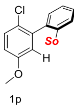
Figure VII-31 : scope limitations
