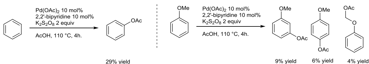
Figure V-3 : early examples of palladium-catalyzed acetoxylation
