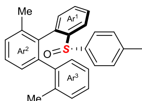
( R )-2,3'-dimethyl-2''-(( S )- p -tolylsulfinyl)-1,1':2',1''-terphenyl Chemical Formula: C 27 H 24 OS Molecular Weight: 396,5480
