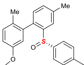
(S)-5'-methoxy-2',4-dimethyl-2-(p-tolylsulfinyl)-1,1'-biphenyl Chemical Formula: C 22 H 22 O 2 S Molecular Weight: 350,4760
