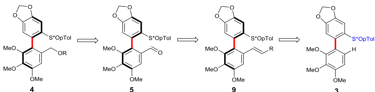
Figure VI-15 : atroposelective Fujiwara-Moritani retrosynthetic scheme
