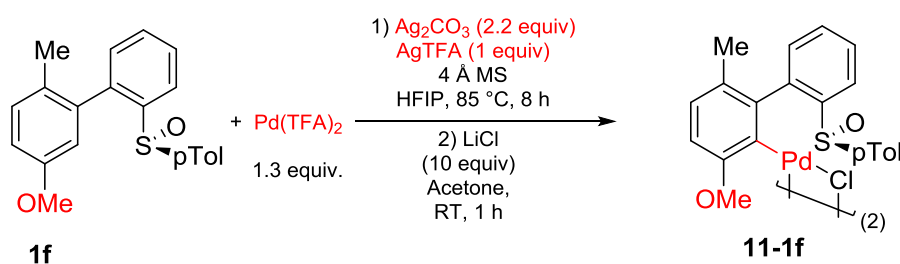
Figure VII-78 : attempt of isolation of 1f palladacycle in reaction conditions
