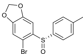
(S)-5-bromo-6-(p-tolylsulfinyl)benzo[d][1,3]dioxole Chemical Formula: C 14 H 11 BrO 3 S Molecular Weight: 339,2030
