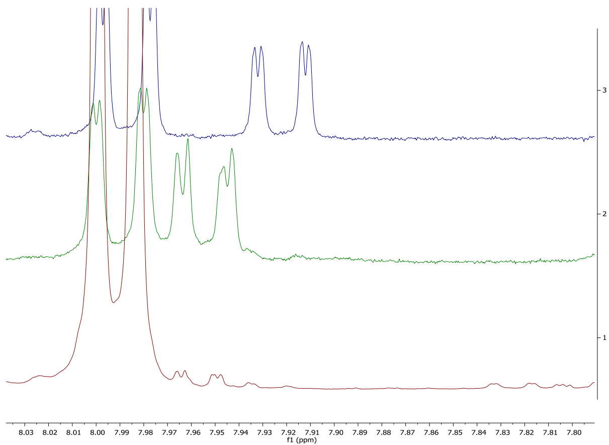
Figure VII-53 : identification of 3fN diastereomers; Top spectra : epi red/ox ; middle spectra thermal epi ; bottom spectra crude ^1\text{H} NMR
