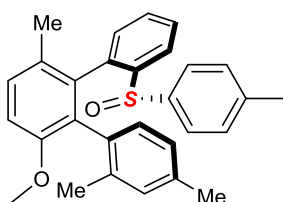
(1' S ,2' R )-6'-methoxy-2,3',4-trimethyl-2''-(( S )- p -tolylsulfinyl)-1,1':2',1''-terphenyl Chemical Formula: C 29 H 28 O 2 S Molecular Weight: 440,6010
