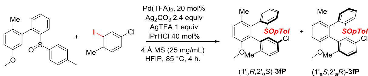
FigureVII-62: arylation of racemic 3fO
