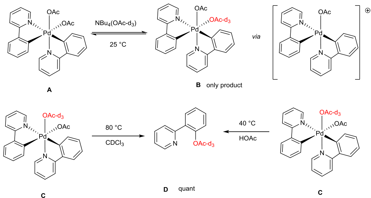
Figure V-13 : dissociative mechanism evidence
