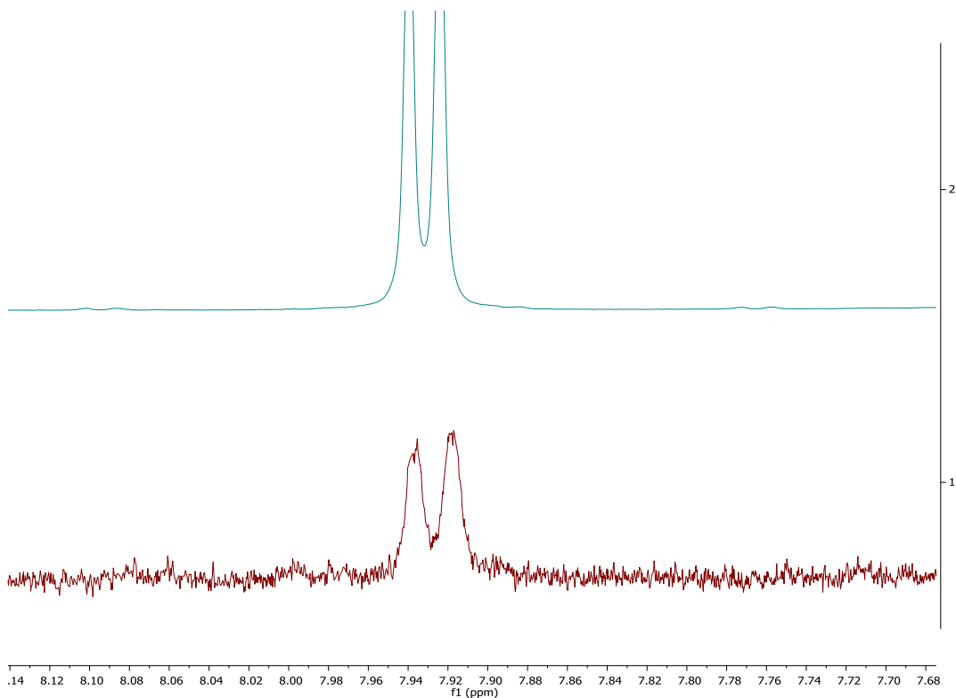
Figure VII-41 : Study of the thermal stability of Ar 1 -Ar 2 axis of 3al
