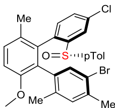
(1'S,2'R)-5-bromo-4''-chloro-6'-methoxy-2,3',4-trimethyl-2''-((S)-p-tolylsulfinyl)-1,1':2',1''-terphenyl Chemical Formula: C 29 H 26 BrClO 2 S Molecular Weight: 553,9390
