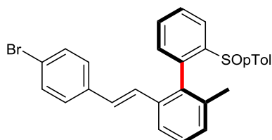
(aR)-2-((E)-4-bromostyryl)-6-methyl-2'-((S)-p-tolylsulfinyl)-1,1'-biphenyl Chemical Formula: C 28 H 23 BrOS Molecular Weight: 487,4550
