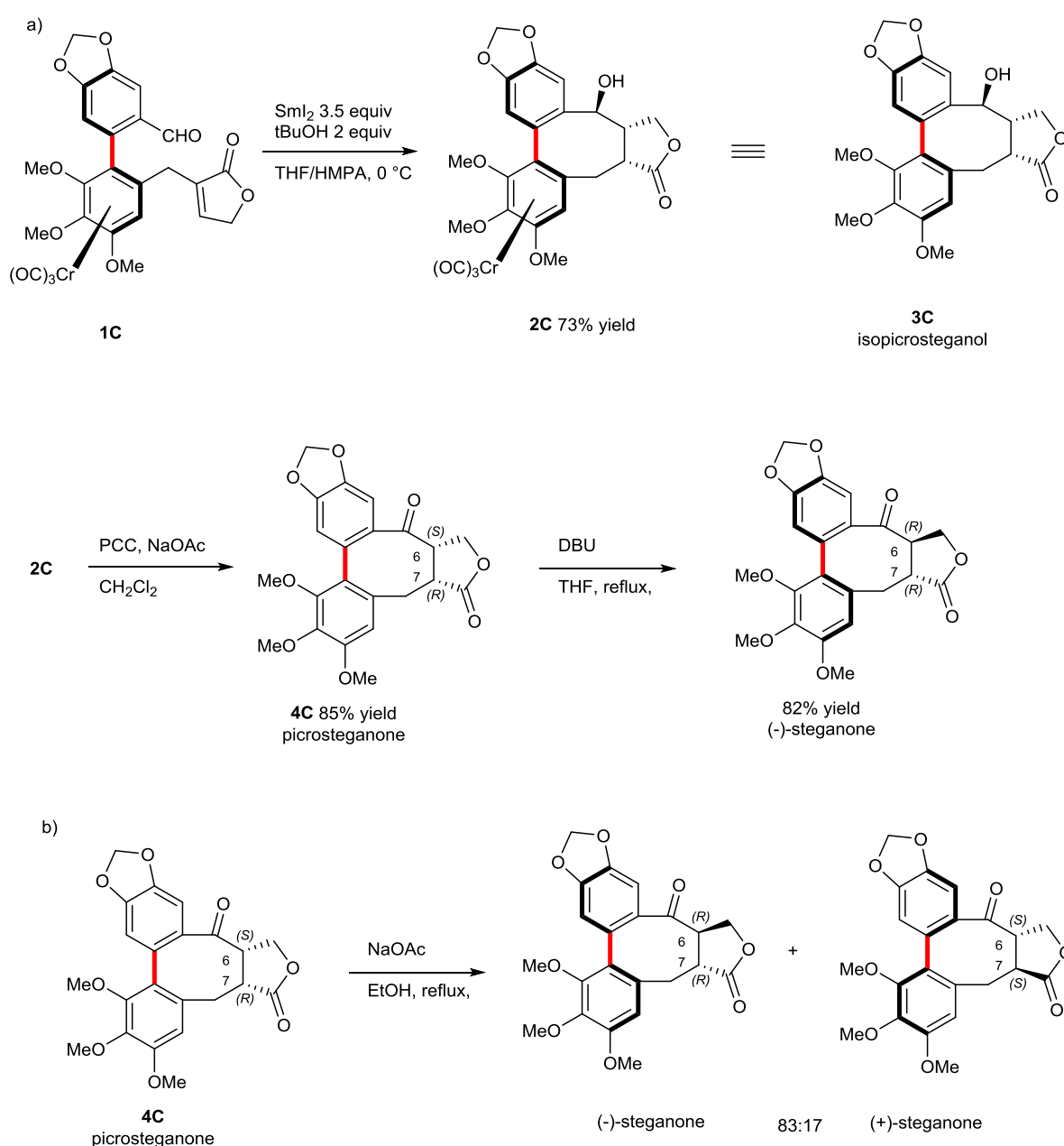
Figure VI-7 : total synthesis and studies on isomerization
