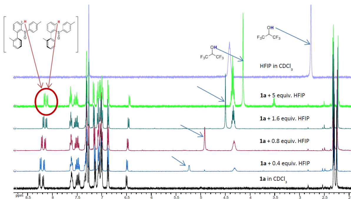
Figure IV-16 : 1 H NMR titration of 1a by HFIP in CDCl 3
