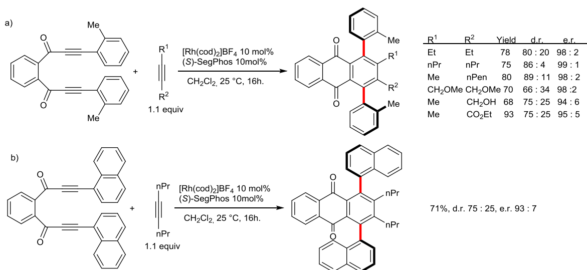
Figure VII-16 : rhodium catalyzed para -teraryl formation
