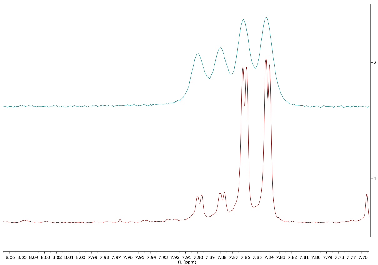
Figure VII-58 thermal epimerization of 3gV. Top spectra : thermal epimerization ; Bottom spectra : crude reaction mixture
