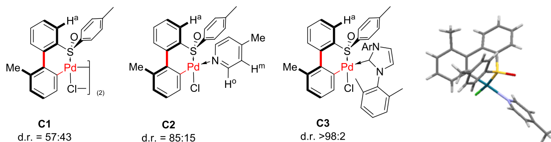
Figure V-20 : isolated palladacycles ; C2 X-ray crystal structure
