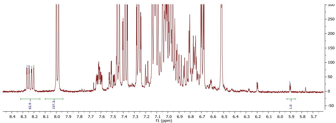
Figure VII-73 : reversibility of 1f arylation in anhydrous conditions
