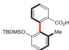
( R )-2'-(( tert -butyldimethylsilyloxy)-6'-methyl-[1,1'-biphenyl]-2-carboxylic acid Chemical Formula: \text{C}_{20}\text{H}_{26}\text{O}_3\text{Si} Molecular Weight: 342,5100
