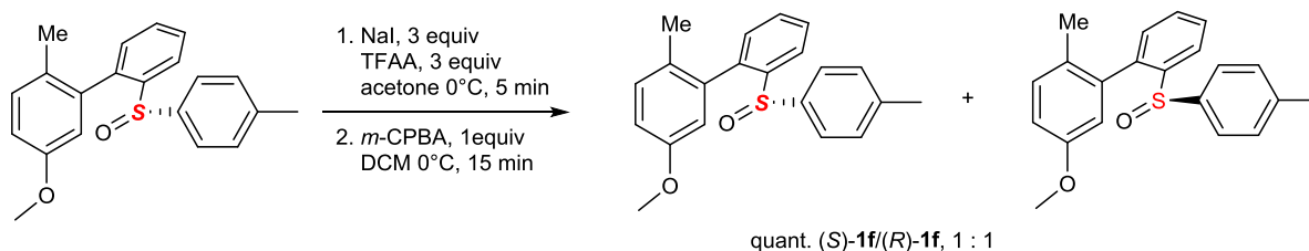
FigureVII-45 : preparation of racemic 1f
