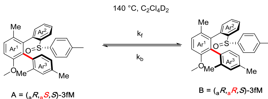
Figure VII-67 : calculation of the rate of epimerization and the rotational barrier
