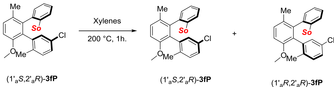
FigureVII-59 : thermal epimerization of 3fP
