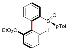
ethyl ( R )-6-iodo-2'-(( S )- p -tolylsulfinyl)-[1,1'-biphenyl]-2-carboxylate Chemical Formula: C 22 H 19 O 3 S Molecular Weight: 490,3555
