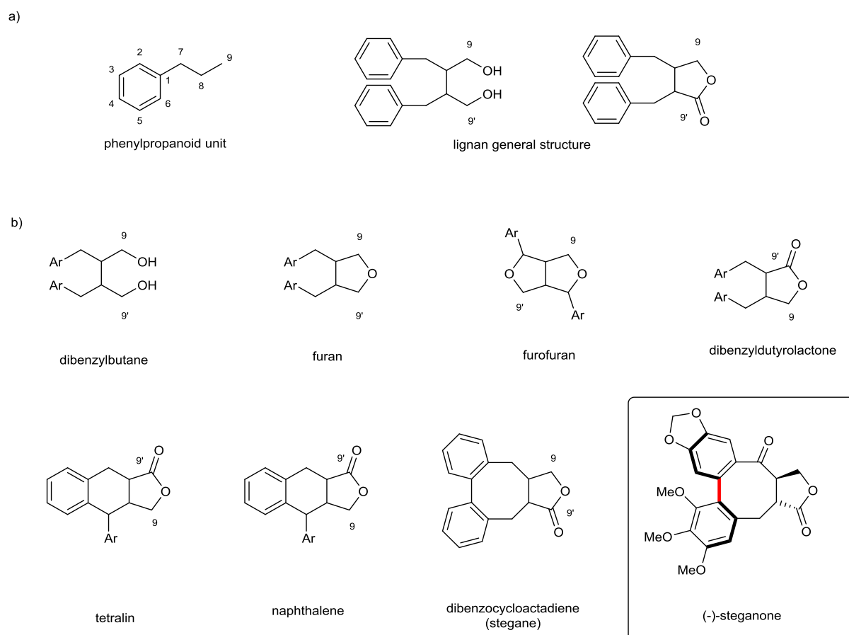
Figure VI-1 : lignans natural products
