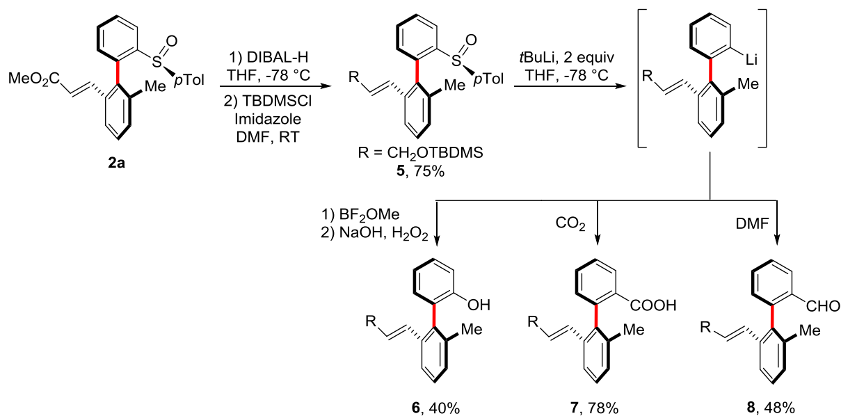
Figure IV-22 : Examples of transformation of sulfoxide DG
