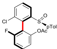
( R )-2'-chloro-6-fluoro-6'-(( S )- p -tolylsulfinyl)-[1,1'-biphenyl]-2-yl acetate Chemical Formula: C 21 H 16 ClFO 3 S Molecular Weight: 402,8644
