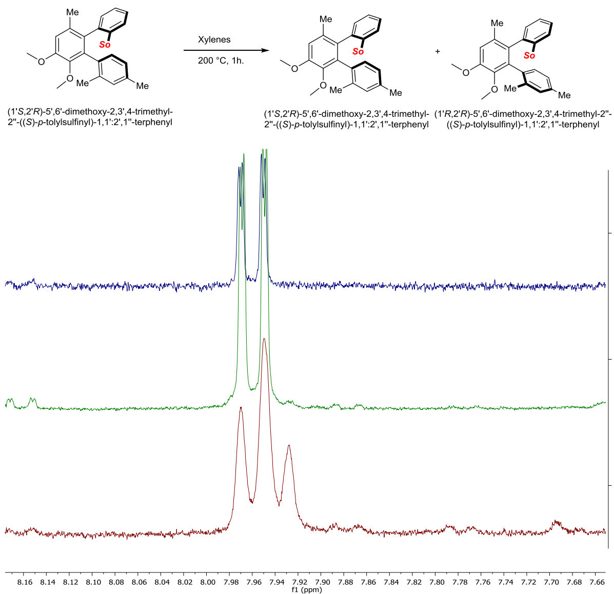
Figure VII-50 : thermal epimerization of 3eM : Top isolated product; middle crude mixture ; bottom crude mixture after thermal epimerization
