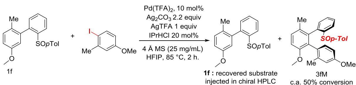
FigureVII-46: arylation of racemic 1f
