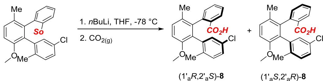
FigureVII-63 : functionalization of epimerized 3fO
