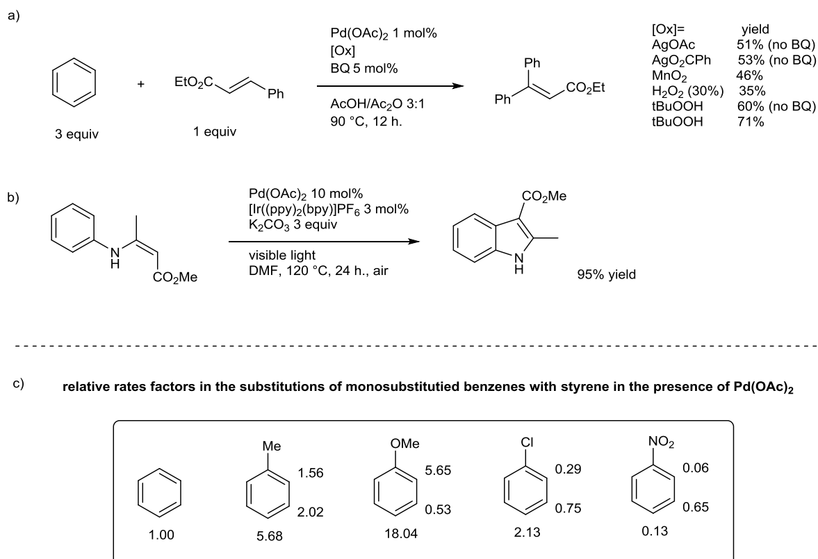
Figure IV-3 : scope of oxidants and regioselectivity of the Fujiwara-Moritani reaction
