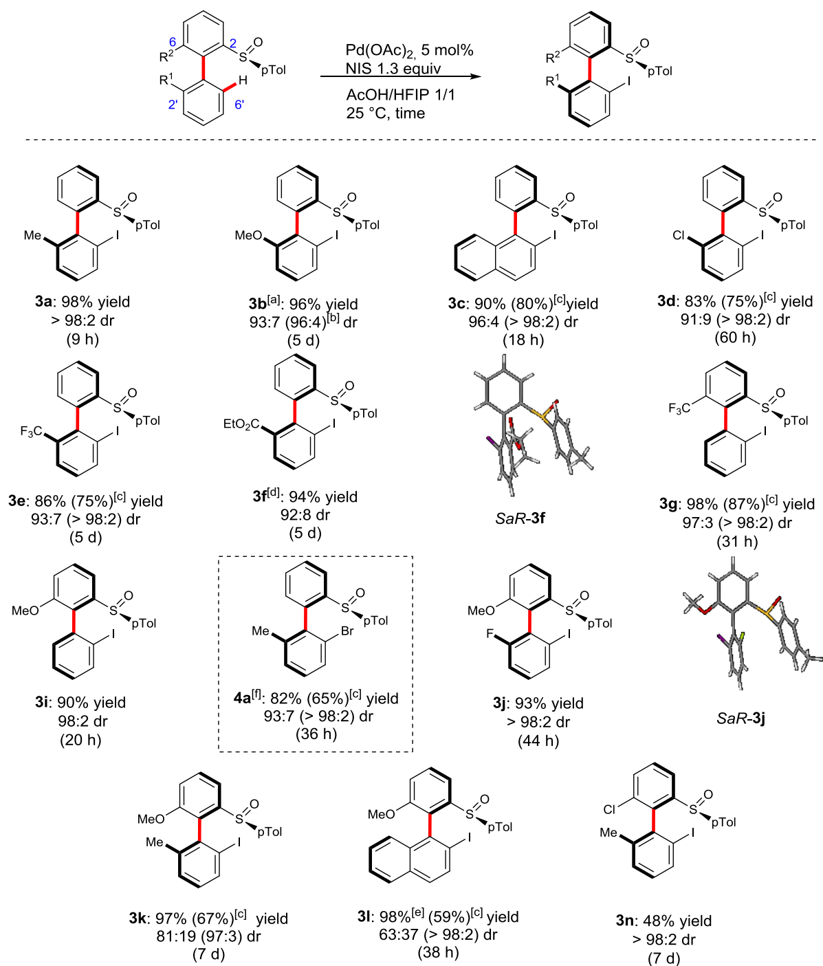
Figure V-30 : Substrate scope for asymmetric iodination occurring via KR/DKR
