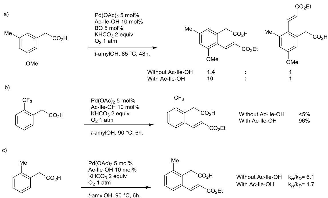
Figure IV-7 : use of MPAAs
