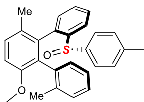
(1' R ,2' S )-3'-methoxy-2'',6'-dimethyl-2-(( S )- p -tolylsulfinyl)-1,1':2',1''-terphenyl Chemical Formula: C 28 H 26 O 2 S Molecular Weight: 426,5740
