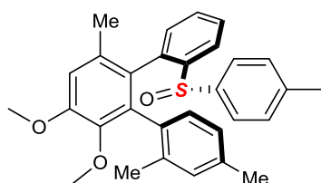
(1' S ,2' R )-5',6'-dimethoxy-2,3',4'-trimethyl-2''-(( S )- p -tolylsulfinyl)-1,1':2',1''-terphenyl Chemical Formula: C 30 H 30 O 3 S Molecular Weight: 470,6270
