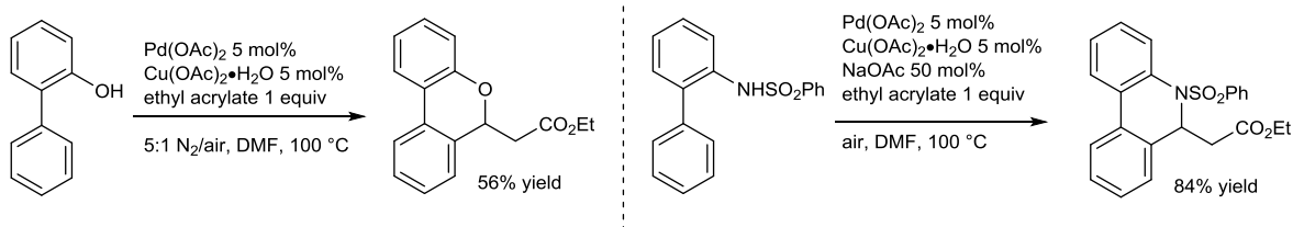
Figure IV-9 : F-M reactions on biaryls
