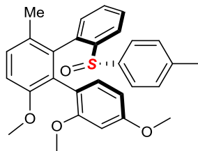
(1' S ,2' R )-2,4,6'-trimethoxy-3'-methyl-2''-((S)-p-tolylsulfinyl)-1,1':2',1''-terphenyl Chemical Formula: C 29 H 28 O 4 S Molecular Weight: 472.5990
