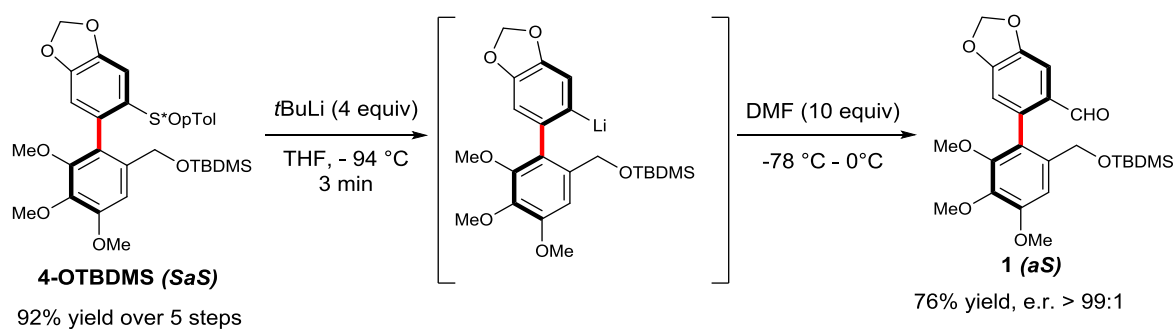
Figure VI-19 : synthesis of 1
