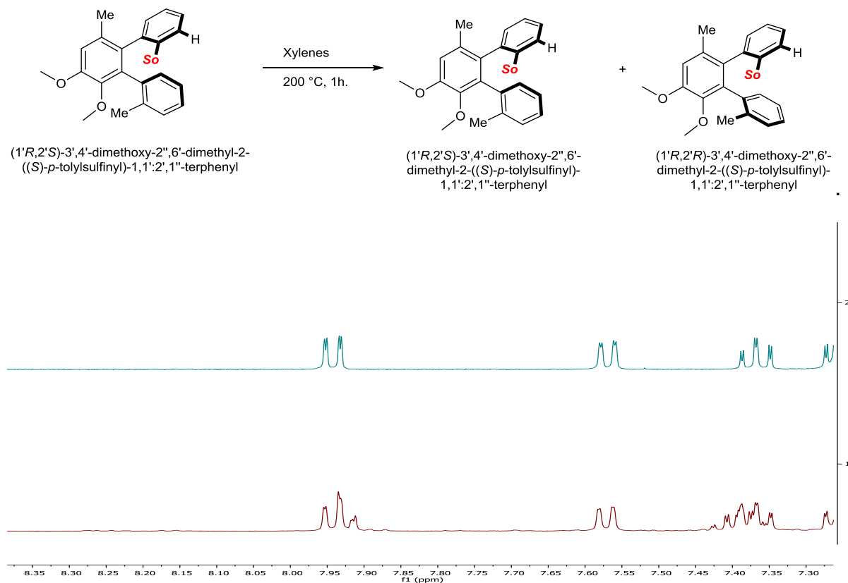
Figure VII-43 : Thermal epimerization of Ar 2 -Ar 3 axis of 3eJ
