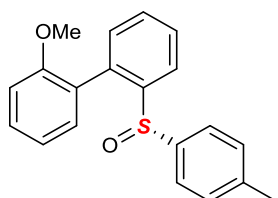
( S )-2-methoxy-2'-( p -tolylsulfinyl)-1,1'-biphenyl Chemical Formula: \text{C}_{20}\text{H}_{18}\text{O}_2\text{S} Molecular Weight: 322,4220
