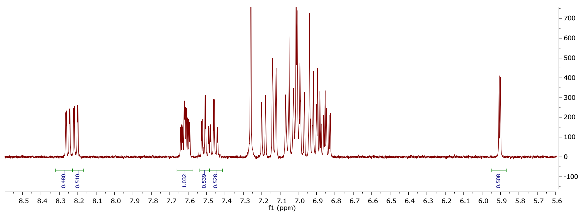
Figure VII-72 : identification of 1a characteristic signals
