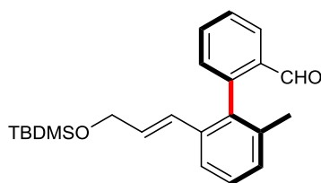
( R,E )-2'-(3-(( tert -butyldimethylsilyloxy)prop-1-en-1-yl)-6'-methyl-[1,1'-biphenyl]-2-carbaldehyde Chemical Formula: C_{23}H_{30}O_2Si Molecular Weight: 366,5760
