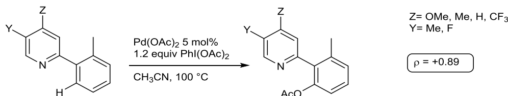
Figure V-10 : Hammett-plot experiment
