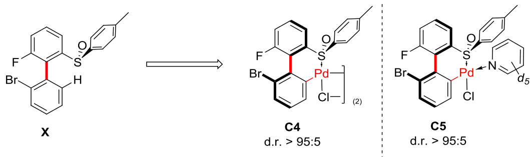
Figure V-25 : literature precedent of biphenylsulfoxyde palladacycles
