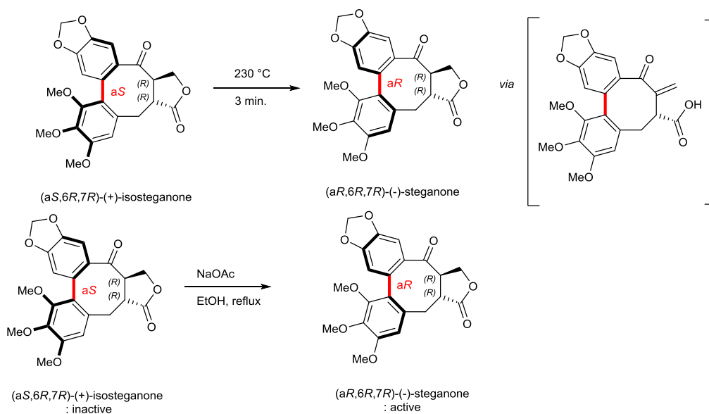
Figure VI-4 : steganone isomerization
