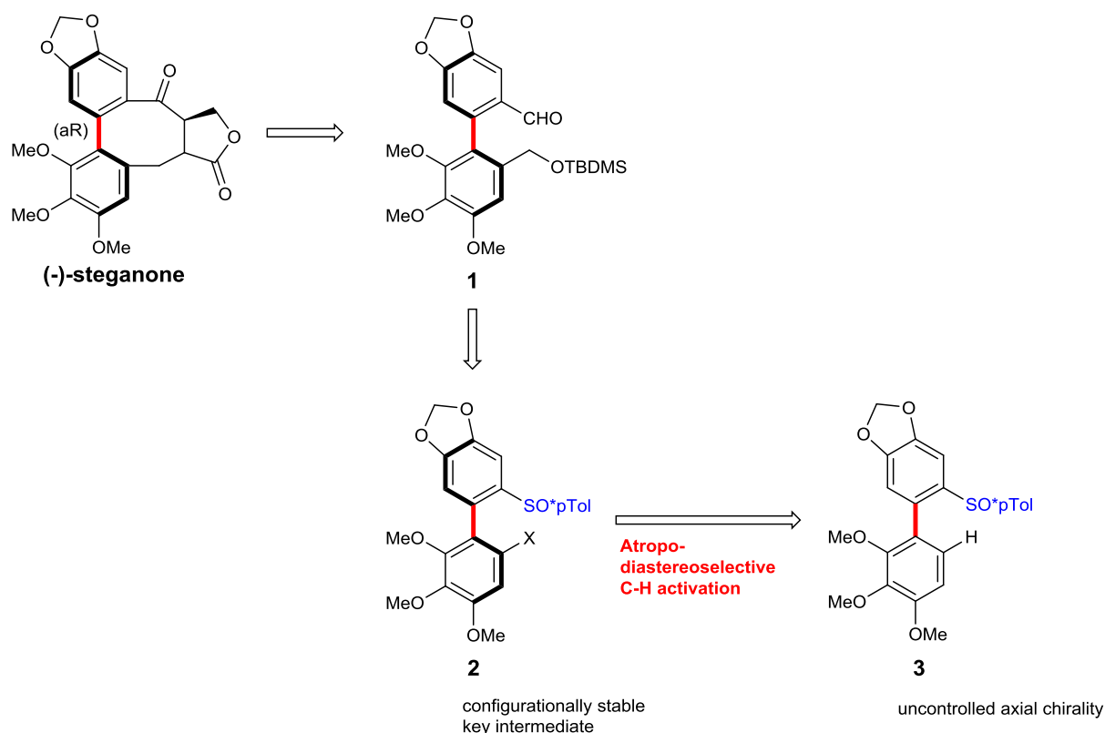
Figure VI-13 : retrosynthetic strategy
