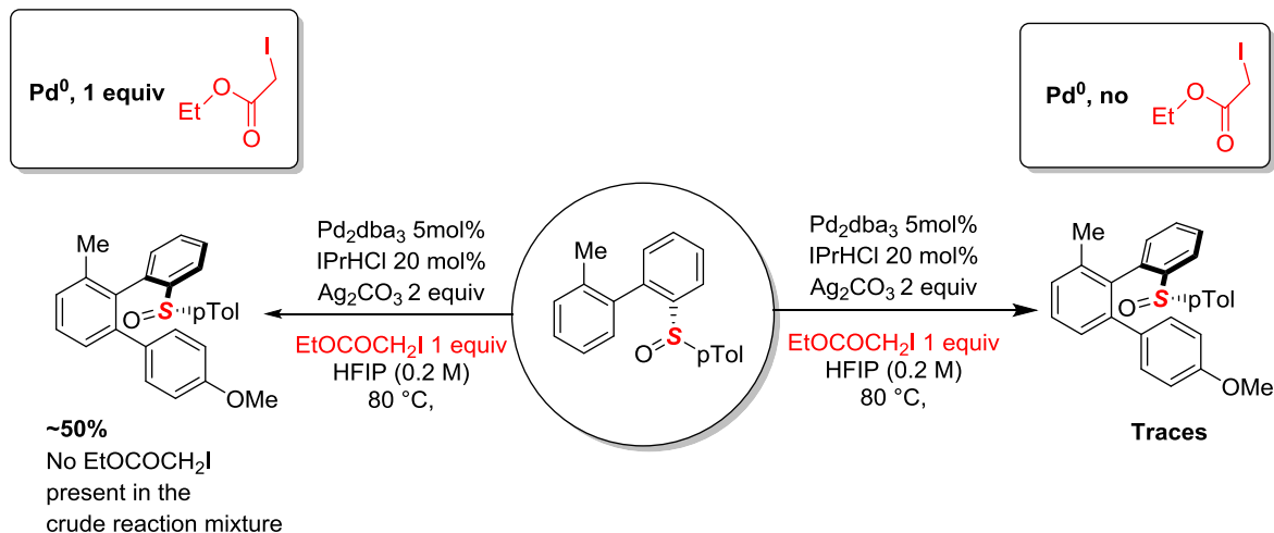
FigureVII-71 : experiments on the role of ethyl iodoacetate
