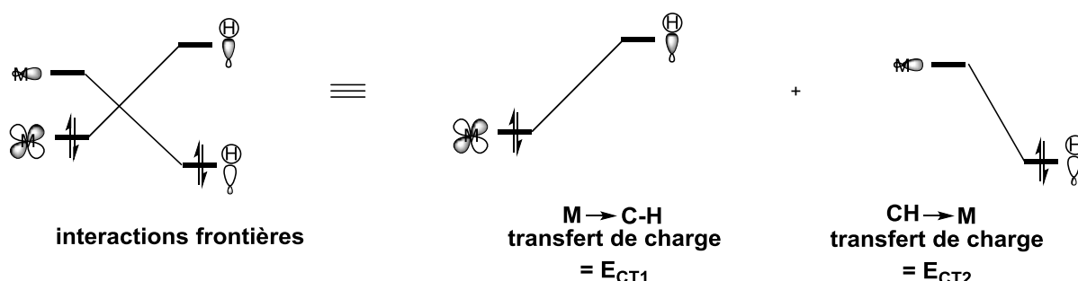
Figure III-4 : interactions frontalières
