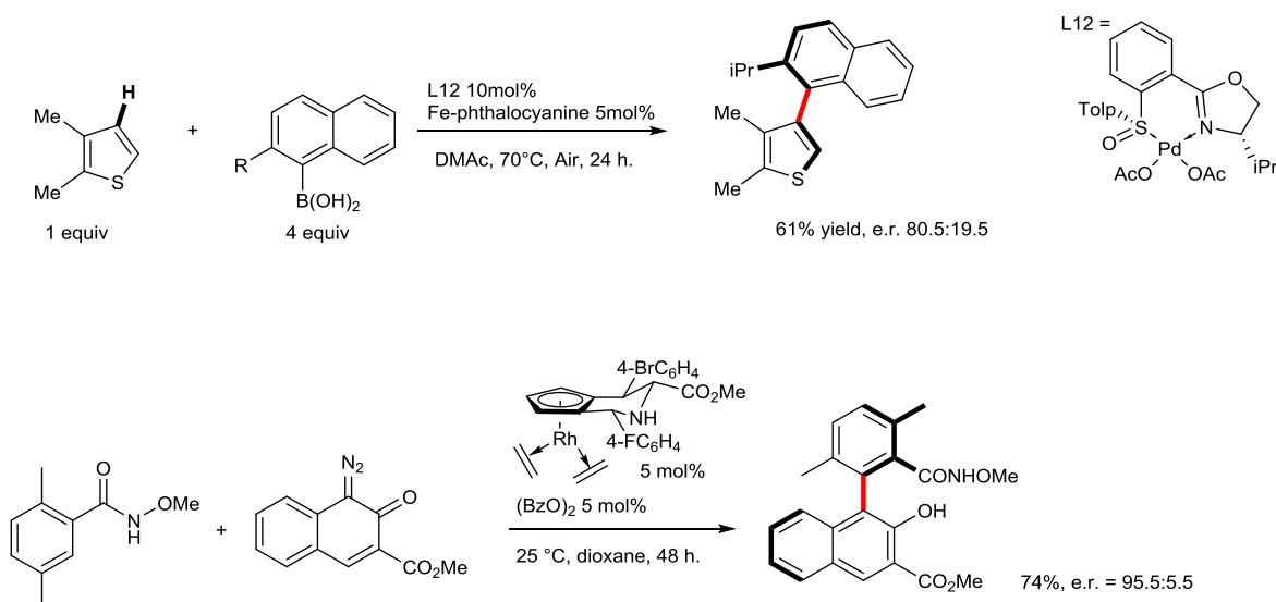
Figure VII-20 : atroposelective direct arylation
