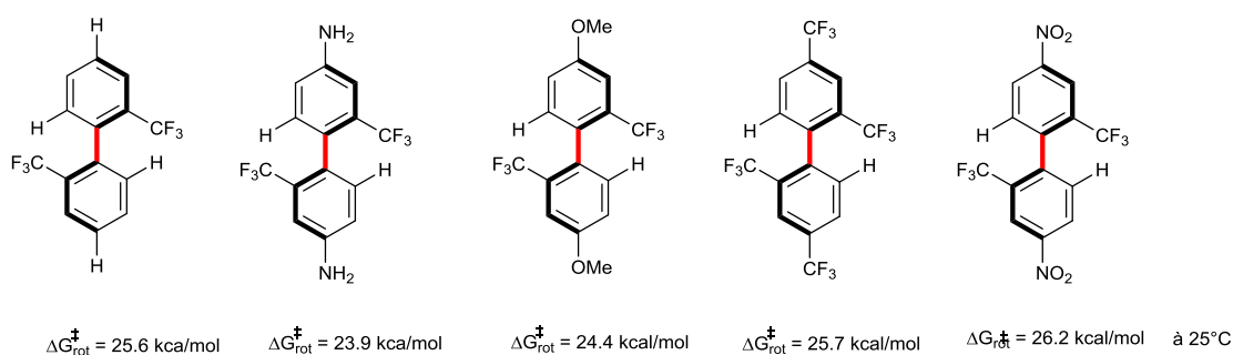
Figure III-20 : influence des substituents para
