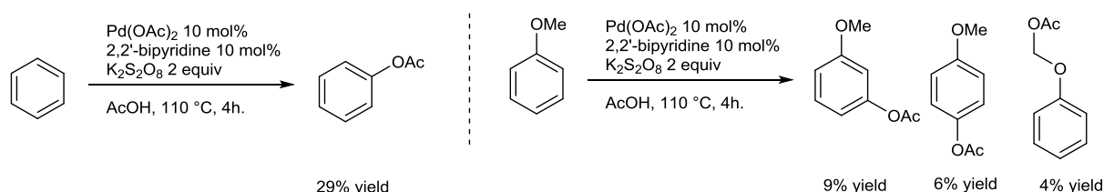
Figure V-3 : early examples of palladium-catalyzed acetoxylation
