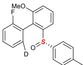
2'-fluoro-2-methoxy-6-((S)- p -tolylsulfinyl)-1,1'-biphenyl-6'- d Chemical Formula: C 20 H 16 DFO 2 S Molecular Weight: 341,4185
