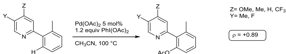
Figure V-10 : Hammett-plot experiment
