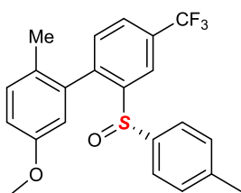
(S)-5'-methoxy-2'-methyl-2-(p-tolylsulfinyl)-4-(trifluoromethyl)-1,1'-biphenyl
