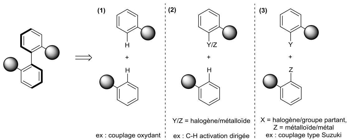
Figure III-24 : types de couplages Ar-Ar
