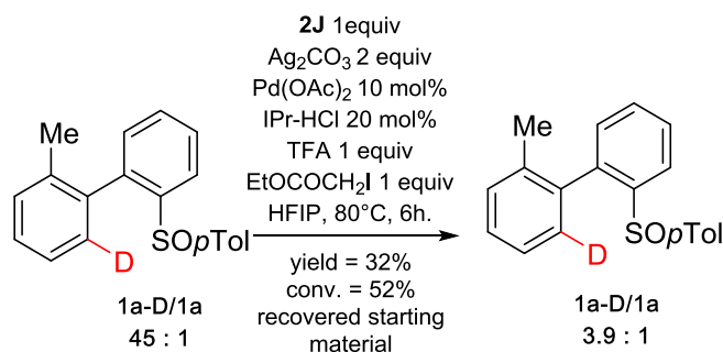
FigureVII-70 : reversibility of arylation of 1a in non-anhydrous conditions
