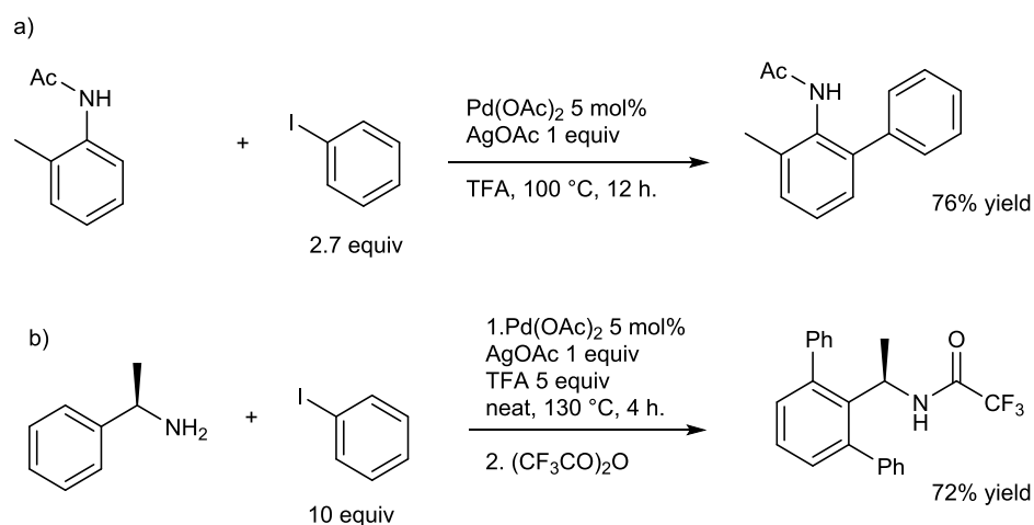
Figure VII-7 : early Pd II -Pd IV arylations
