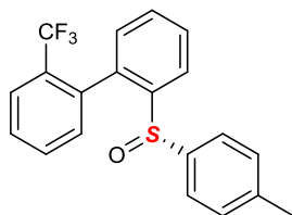
(S)-2-( p -tolylsulfinyl)-2'-(trifluoromethyl)-1,1'-biphenyl Chemical Formula: C 20 H 15 F 3 OS Molecular Weight: 360,3942
