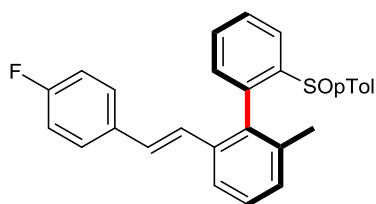
(aR)-2-((E)-4-fluorostyryl)-6-methyl-2'-((S)-p-tolylsulfinyl)-1,1'-biphenyl Chemical Formula: C 28 H 23 FOS Molecular Weight: 426,5494
