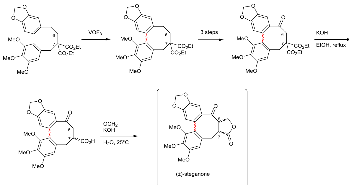
Figure VI-3 : first total synthesis of steganone
