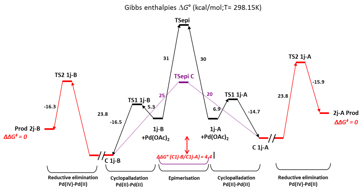
Figure V-24 : 1j reaction profile
