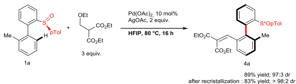
Figure IV-14 : synthesis of atropopure biaryl bearing a 1,1-disubstituted olefin moiety.
