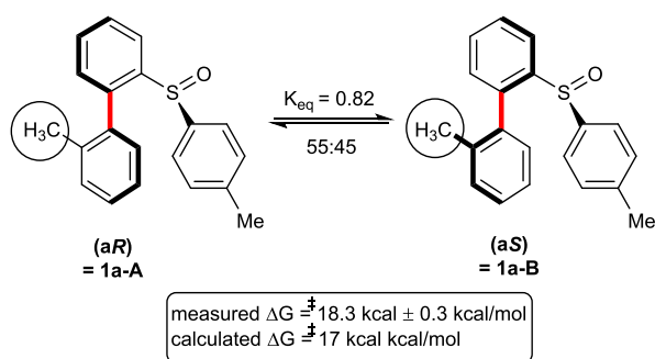
Figure V-19 : rotational barrier of substrate 1a
