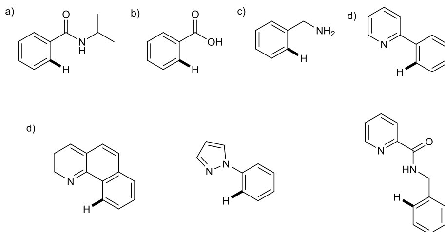
Figure VII-8 : directing groups in palladium catalyzed arylation
