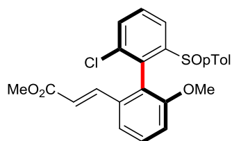
methyl (E)-3-((R)-2'-chloro-6-methoxy-6'-((S)-p-tolylsulfinyl)-[1,1'-biphenyl]-2-yl)acrylate Chemical Formula: C 24 H 21 ClO 4 S Molecular Weight: 440,9380
