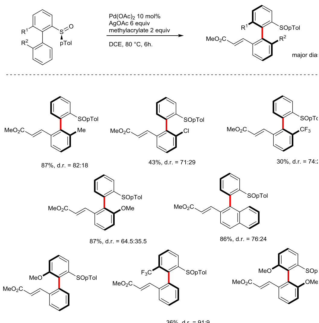
Figure IV-10 : seminal atroposelective F-M reaction
