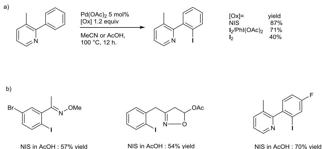
Figure V-27 : first example of directed Pd-catalyzed iodination
