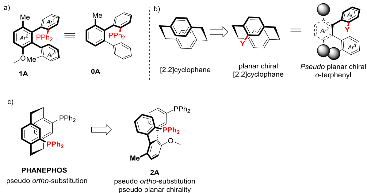
Figure VII-12 : o -terphenyls, cyclophane and pseudo planar chirality
