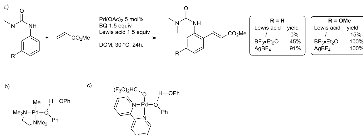
Figure IV-20 : lewis acid accelerated F-M reaction. Palladium complexes exhibiting H-bonding
