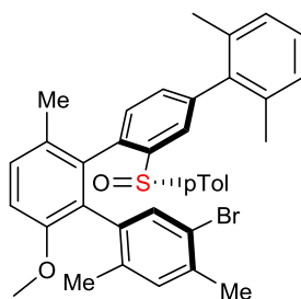
(1'S,2'R)-5-bromo-6'-methoxy-2,2'',3',4,6'''-pentamethyl-2''-((S)- p -tolylsulfinyl)-1,1':2',1'':4'',1'''-quaterphenyl Chemical Formula: C 37 H 35 BrO 2 S Molecular Weight: 623,6490
