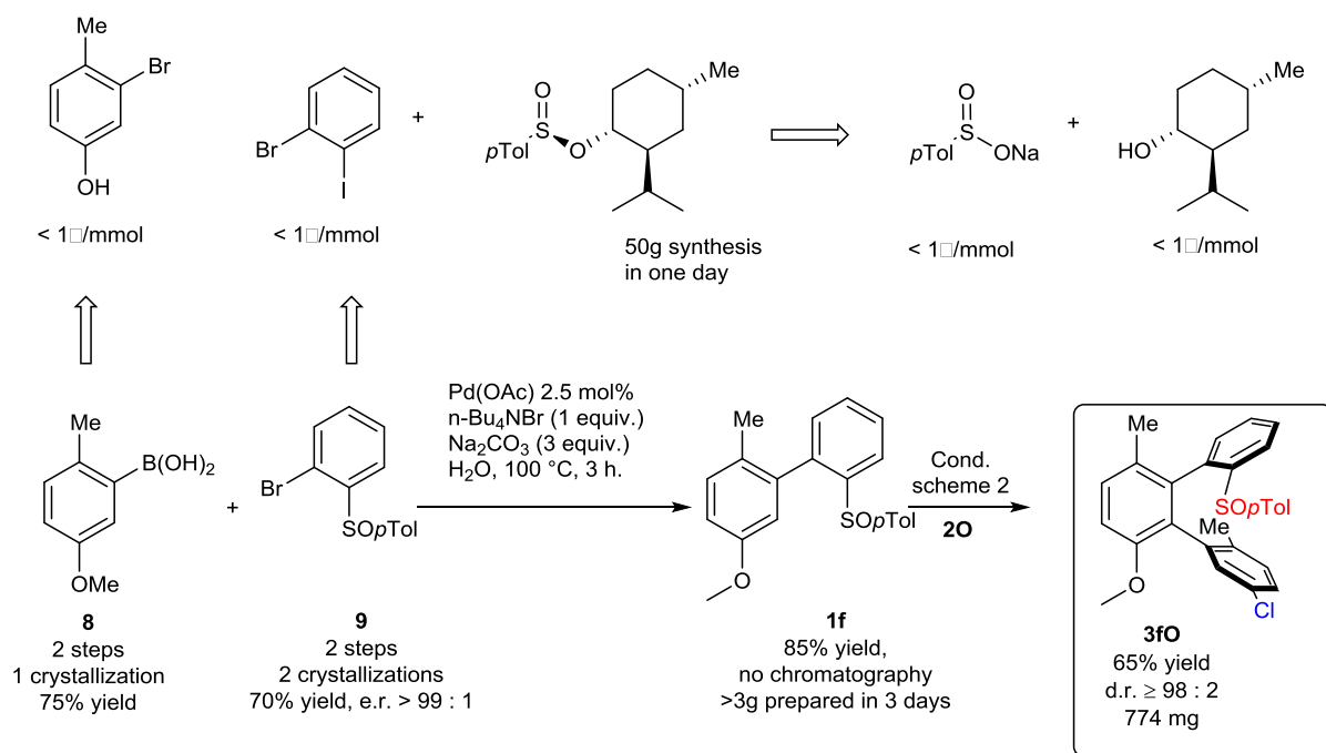
Figure VII-29 : large scale synthesis of 3fP
