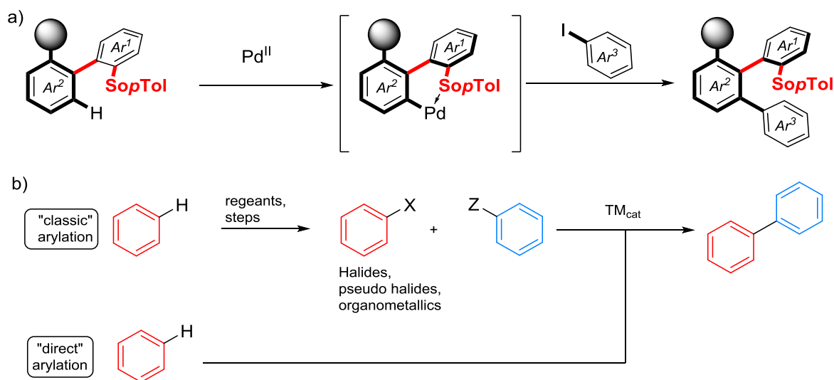
Figure VII-1: arylation of biphenyl sulfoxide and classic and direct arylation
