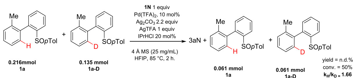
Figure VII-75 : KIE of arylation of 1a into 3aN
