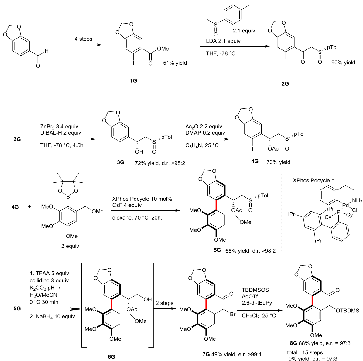
Figure VI-11 : formal synthesis through atropodiselective Suzuki coupling reaction
