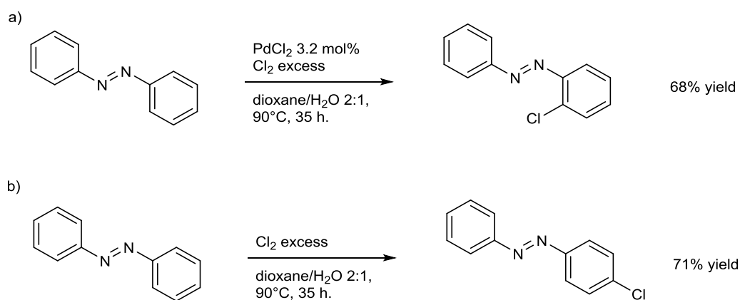
Figure V-26 : early examples of C-X Pd-catalyzed bond formation
