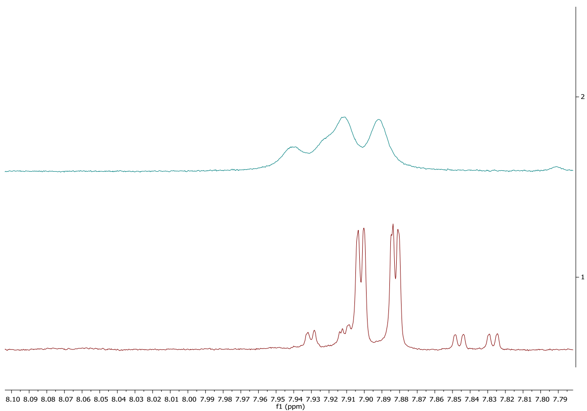
Figure VII-56 : thermal epimerization of 3fl. Top spectra : thermal epimerization ; Bottom spectra : crude reaction mixture
