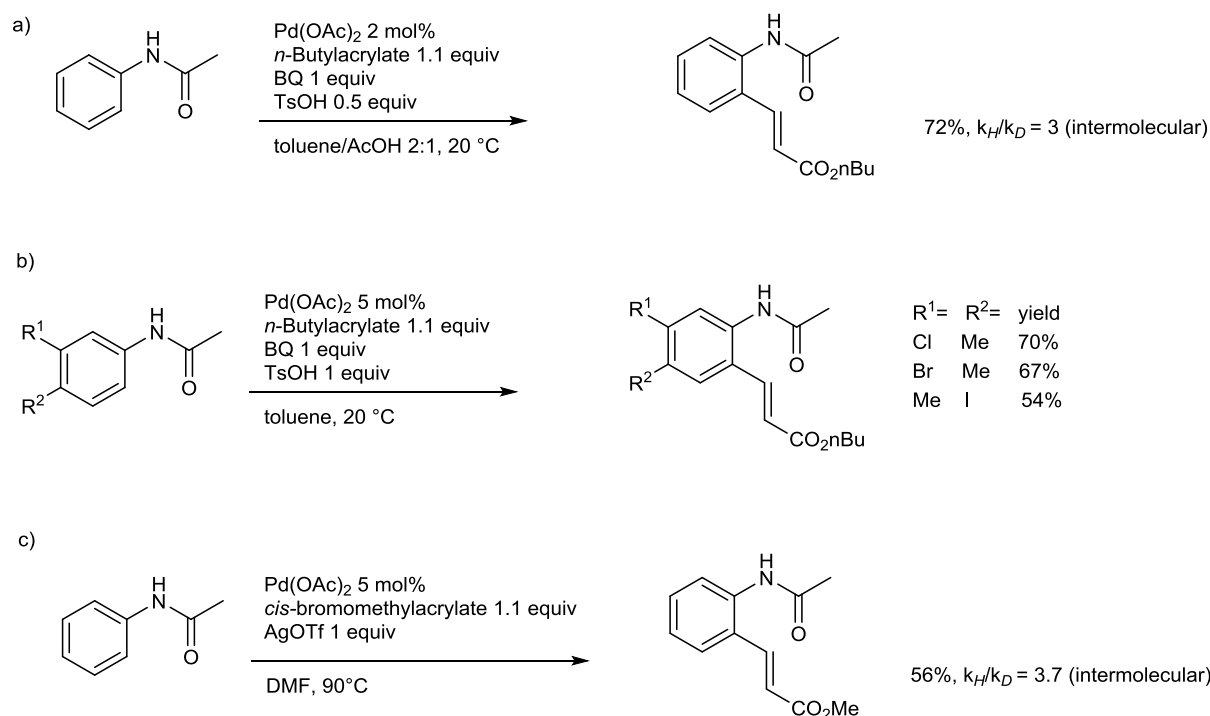
Figure IV-6 : example of directed Fujiwara-Moritani reaction
