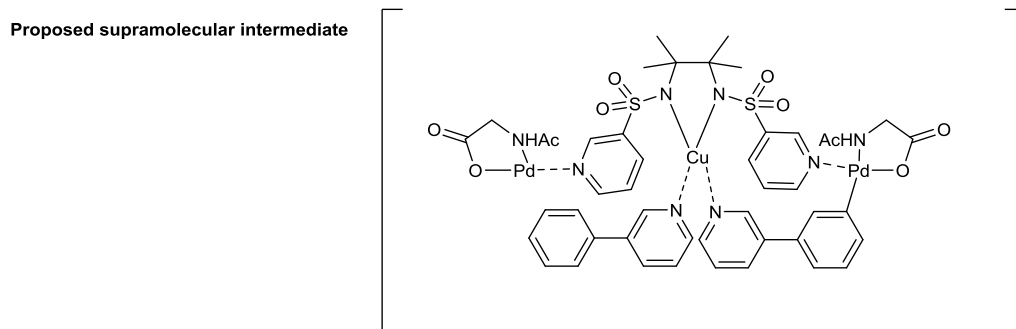
Figure IV-8 : meta selective F-M reactions
