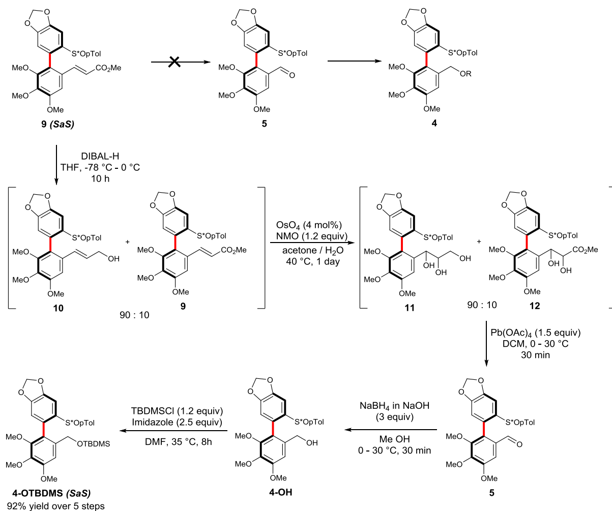
Figure VI-18 : synthesis of 4-OTBDMS
