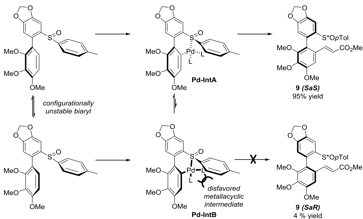
Figure VI-17 : stereoselectivity rationale
