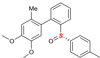
( S )-4,5-dimethoxy-2-methyl-2'-( p -tolylsulfinyl)-1,1'-biphenyl Chemical Formula: \text{C}_{22}\text{H}_{22}\text{O}_3\text{S} Molecular Weight: 366,4750
