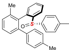
( R )-4'',6'-dimethyl-2-(( S )- p -tolylsulfinyl)-1,1':2',1''-terphenyl Chemical Formula: C 27 H 24 OS Molecular Weight: 396,5480
