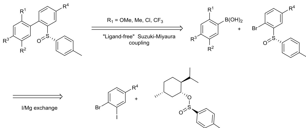
Figure VIII-1 : retrosynthetic scheme
