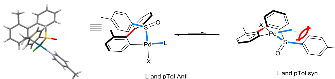
Figure V-21 : stereoselectivity model for the palladacycle intermediate
