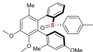
(1'S,2'R)-4,5',6'-trimethoxy-2,3'-dimethyl-2''-((S)-p-tolylsulfinyl)-1,1':2',1''-terphenyl Chemical Formula: C 30 H 30 O 4 S Molecular Weight: 486,6260
