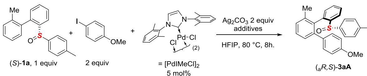
FigureVII-69 : experiments with well-defined Pd-NHC pre-catalysts
