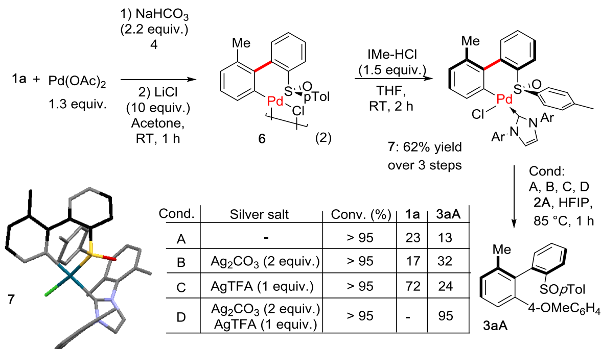
Figure VII-27 : Synthesis and reactivity of palladacyclic intermediate
