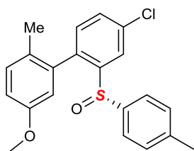
(S)-4-chloro-5'-methoxy-2'-methyl-2-(p-tolylsulfinyl)-1,1'-biphenyl
