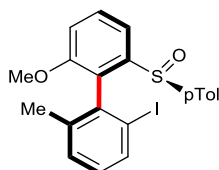
( R )-2-iodo-2'-methoxy-6-methyl-6'-(( S )- p -tolylsulfinyl)-1,1'-biphenyl Chemical Formula: \text{C}_{21}\text{H}_{19}\text{IO}_2\text{S} Molecular Weight: 462,3455
