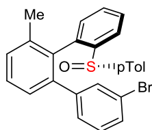
( R )-3''-bromo-6'-methyl-2-(( S )- p -tolylsulfinyl)-1,1':2',1''-terphenyl Chemical Formula: C 26 H 21 BrOS Molecular Weight: 461,4170
