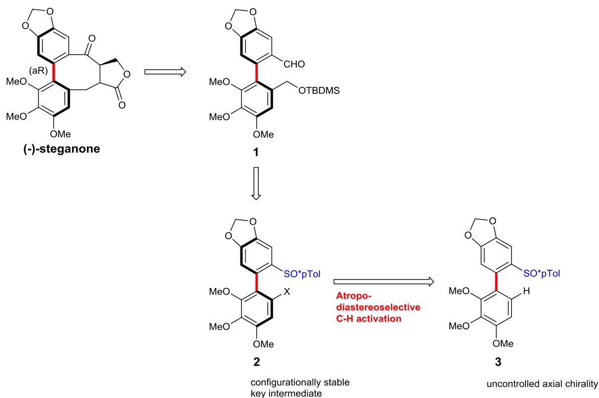
Figure VI-13 : retrosynthetic strategy
