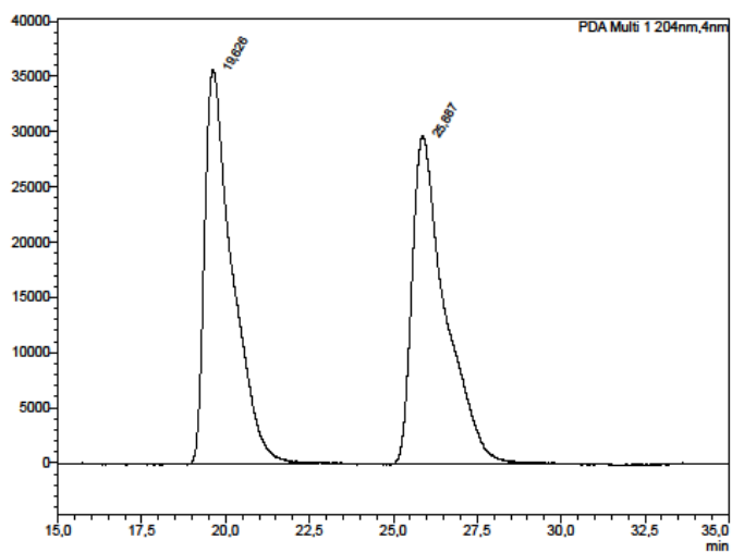
<PDA Chromatogram>
