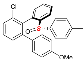
( S )-6'-chloro-4''-methoxy-2-(( S )- p -tolylsulfinyl)-1,1':2',1''-terphenyl Chemical Formula: \text{C}_{26}\text{H}_{21}\text{ClO}_2\text{S} Molecular Weight: 432,9620
