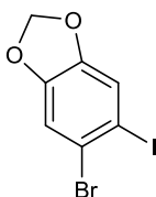
5-bromo-6-iodobenzo[d][1,3]dioxole Chemical Formula: C 7 H 4 BrIO 2 Molecular Weight: 326,9155
