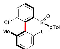
(S)-2-chloro-2'-iodo-6'-methyl-6-((S)-p-tolylsulfinyl)-1,1'-biphenyl Chemical Formula: C 20 H 16 ClIOS Molecular Weight: 466,7615
