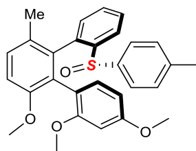
(1' a S,2' a R)-2,4,6'-trimethoxy-3'-methyl-2''-((S)-p-tolylsulfinyl)-1,1':2',1''-terphenyl Chemical Formula: C 29 H 28 O 4 S Molecular Weight: 472.5990
