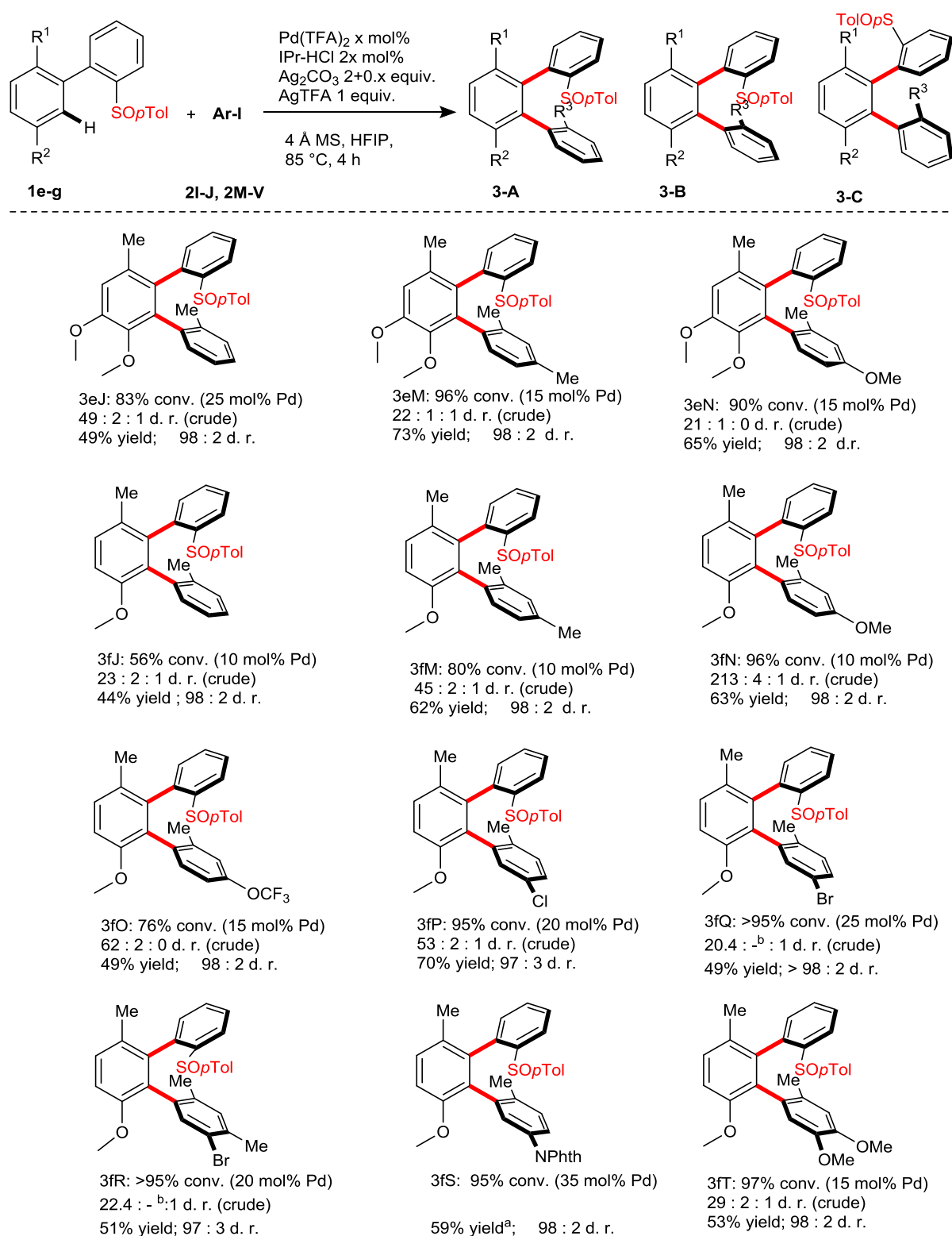
Figure VII-24 : Scope of the terphenyls with two chirality axes; (4 diastereomers could be potentially obtained and 3 of them were identified on crude 1 H NMR)
