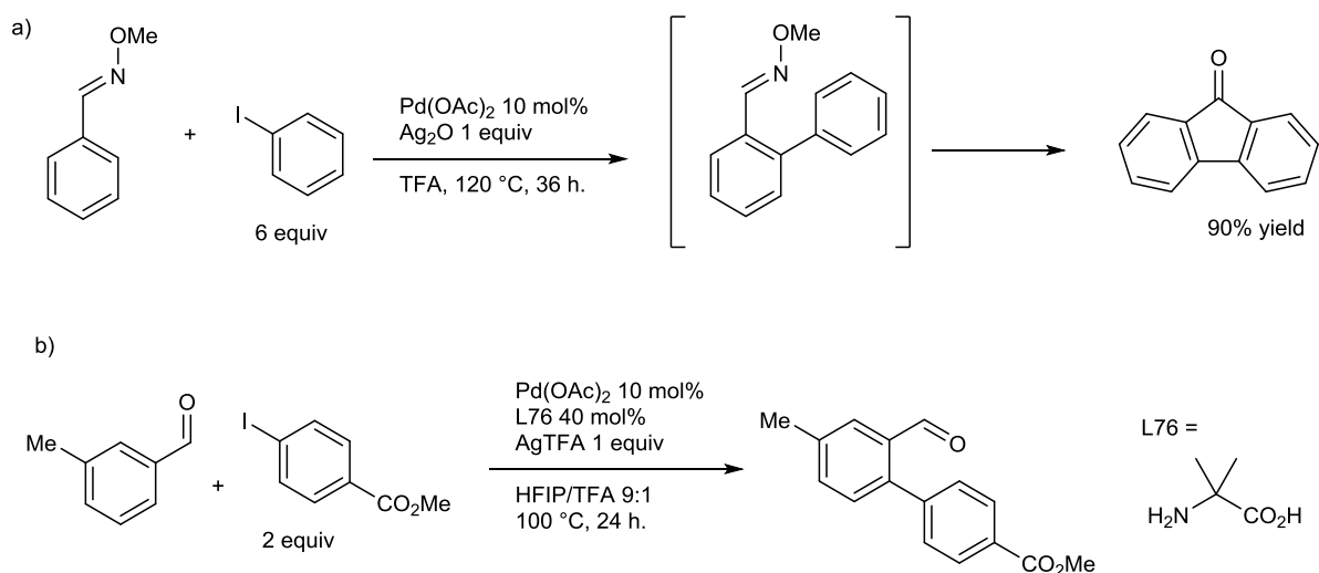
Figure VII-9 : arylation of benzaldehyde derivatives
