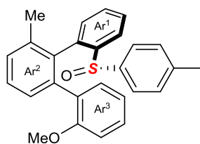
( R )-2-methoxy-3'-methyl-2''-(( S )- p -tolylsulfinyl)-1,1':2',1''-terphenyl Chemical Formula: C 27 H 24 O 2 S Molecular Weight: 412,5470
