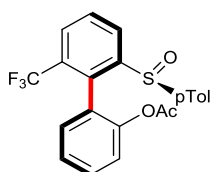
2'-(( S )- p -tolylsulfinyl)-6'-(trifluoromethyl)-[1,1'-biphenyl]-2-yl acetate Chemical Formula: C 22 H 17 F 3 O 3 S Molecular Weight: 418,4302
