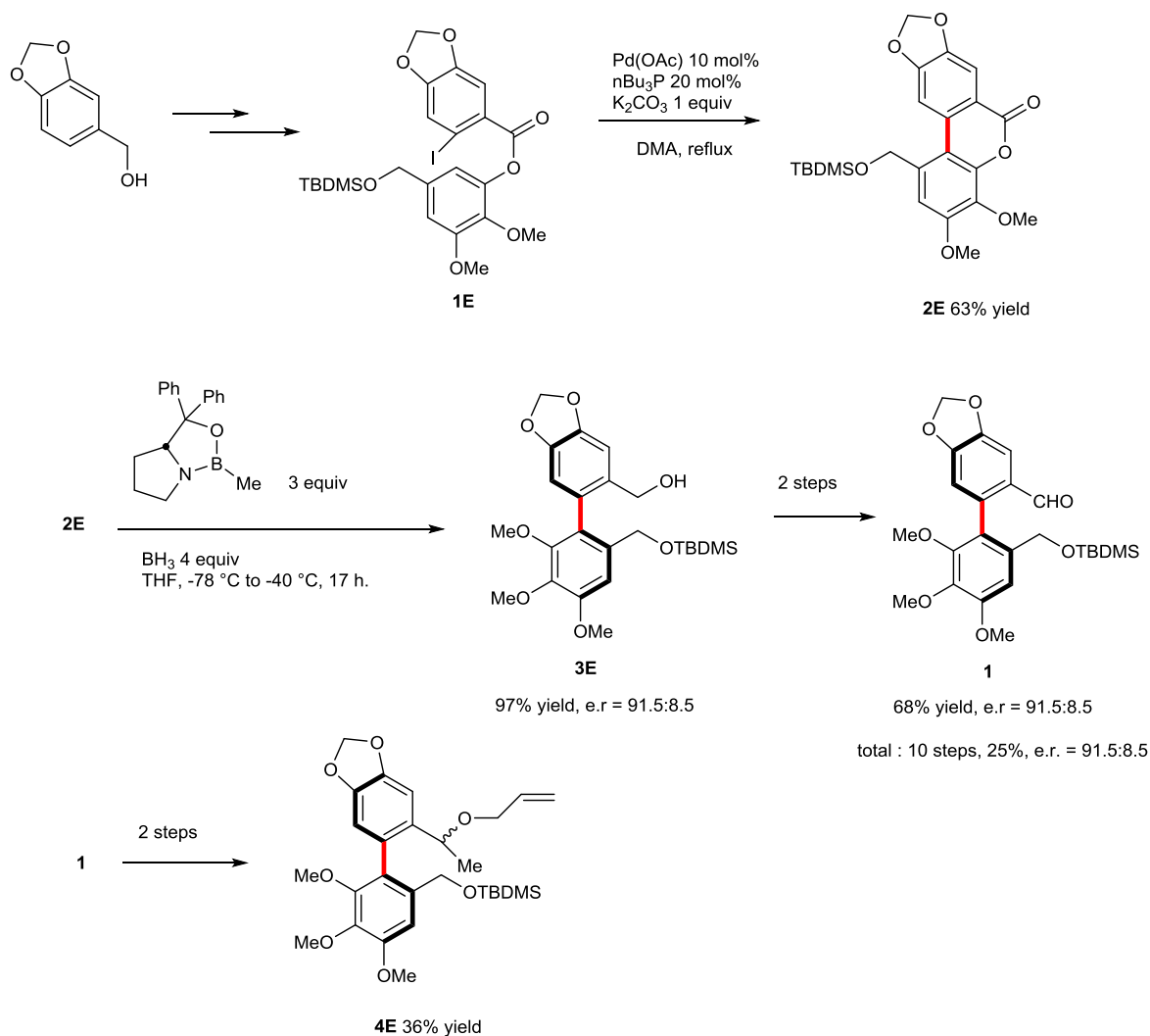
Figure VI-9 : formal synthesis using the lactone concept developed by G. Bringmann
