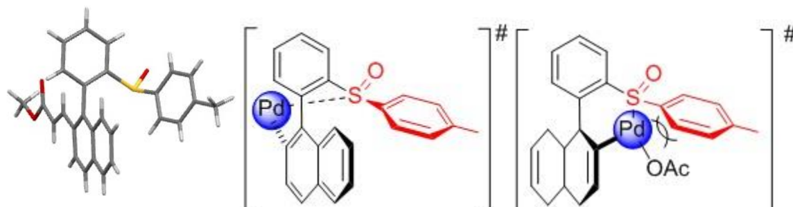
Figure IV-12 : X-Ray structure of ( SaR )- 2c and proposed favoured and unfavoured metallacyclic intermediates
