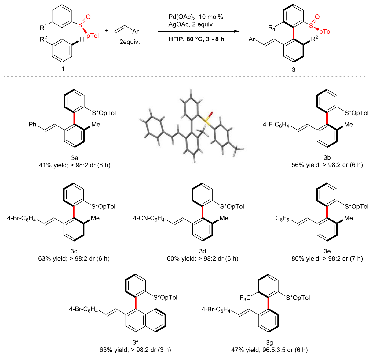
Figure IV-13 : scope of biphenylsulfoxide partners with styrenes. a Isolated yield; dr determined by 1 H NMR.
