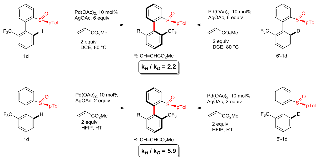
Figure IV-18 : KIEs study in DCE and in HFIP.
