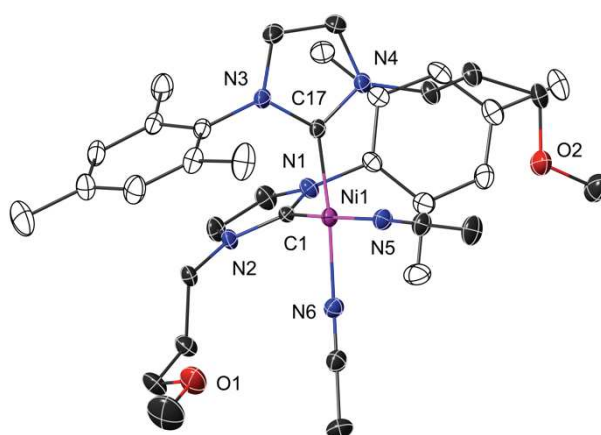
Figure 3. Structure of the Ni(II) complexes 15 with H atoms and \text{PF}_6^- anions omitted for clarity. Thermal ellipsoids at the 40% probability level. Selected bond lengths ( \text{\AA} ) and angles (deg): Ni1–C1 1.884(2), Ni1–C17 1.884(2), Ni1–N5 1.898(2), Ni1–N6 1.906(2), C1–N1 1.364(3), C1–N2 1.349(3), C17–N3 1.359(3), C17–N4 1.348(3), C1–Ni1–C17 89.8(9) , C1–Ni1–N6 92.8(8) , C17–Ni1–N5 91.0(8) , N5–Ni1–N6 87.4(8) , C1–Ni1–N5 172.4(9) , C17–Ni1–N6 172.7(9) , N1–C1–N2 105.2(2) , N3–C17–N4 105.5(2) .
