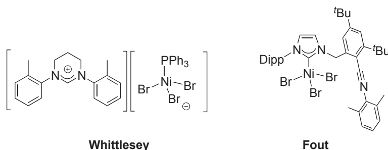
Figure 9. Ni(II) complexes containing a [\text{NiBr}_3]^- moiety (see text)
