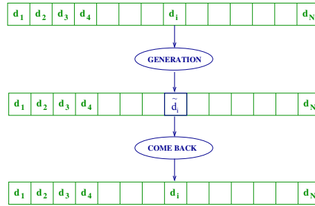
FIGURE 1.10 – Optimization of the generation process. In this figure, the state space is built with a decision vector for which the generation process consist of changing only one decision ( d_i ) in the current solution. If this modification is not accepted, this component of the solution recovers its former value. The only information to be stored is the integer i and the real number d_i .
