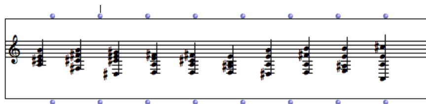
Fig. 30. Chord sequence corresponding to the first bars of Choral 7.
