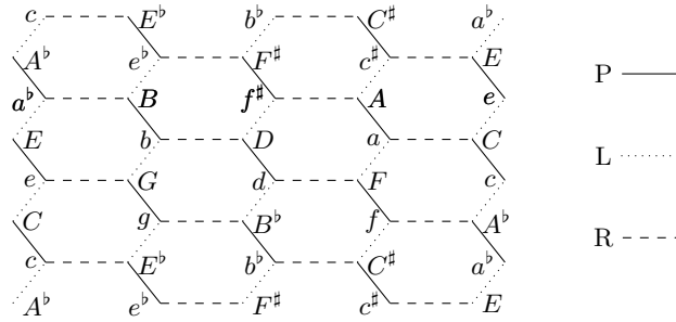
Fig. 8. Douthett and Steinbach's Graph
