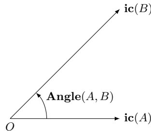
Fig. 21. The measure \mathbf{Angle}(A, B) .
