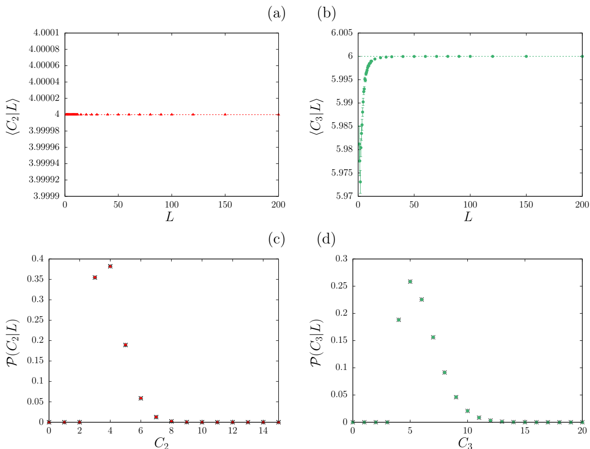
Figure 4.8: (a-b). The first-order moments of the number of faces in d -dimensional Poisson tessellations as a function of the linear size L of the domain. The cases are as follows: (a) the average number of faces \langle C_2|L \rangle for d = 2 , (b) the average number of faces \langle C_3|L \rangle for d = 3 . For each case, symbols correspond to the Monte Carlo simulation results: red triangles denote d = 2 and green circles d = 3 . Simulation results have been obtained with \rho = 1 . We have generated M = 5 \times 10^4 realizations for d = 2 and M = 5 \times 10^3 realizations for d = 3 . (c-d). The probability densities of the number of faces, for different values of the linear size L of the domain. The cases are as follows: (c) the probability density of the number of faces \mathcal{P}(C_2|L) for d = 2 , (d) the probability density of the number of faces \mathcal{P}(C_3|L) for d = 3 . For each case, symbols correspond to the Monte Carlo simulation results: for d = 2 , black crosses denote L = 10 and red triangles L = 200 , for d = 3 black crosses denote L = 10 and green circles L = 200 . Simulation results have been obtained with \rho = 1 . We have generated M = 5 \times 10^4 realizations for d = 2 and M = 5 \times 10^3 realizations for d = 3 .
