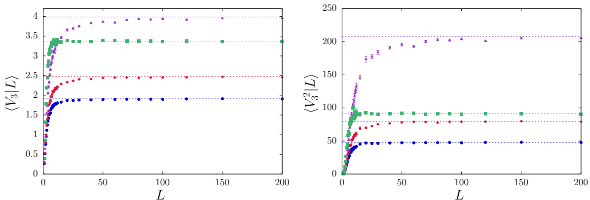
Figure 4.26: Average volume \langle V_3 | L \rangle (left) and second moment of the volume \langle V_3^2 | L \rangle (right) of the Poisson tessellation cells as a function of the box side L , with various anisotropy laws H(\mathbf{n}) , for d = 3 . The tessellation density is \rho = 1 for all the angular laws H(\mathbf{n}) . Symbols denote Monte Carlo simulation results: blue circles correspond to isotropic distribution, red diamonds to quadratic distribution, green squares to box distribution and purple triangles to histogram distribution. Solid lines correspond to the respective limits for infinite Poisson tessellations, as given in Eqs. (2.21) and (2.24), respectively.
