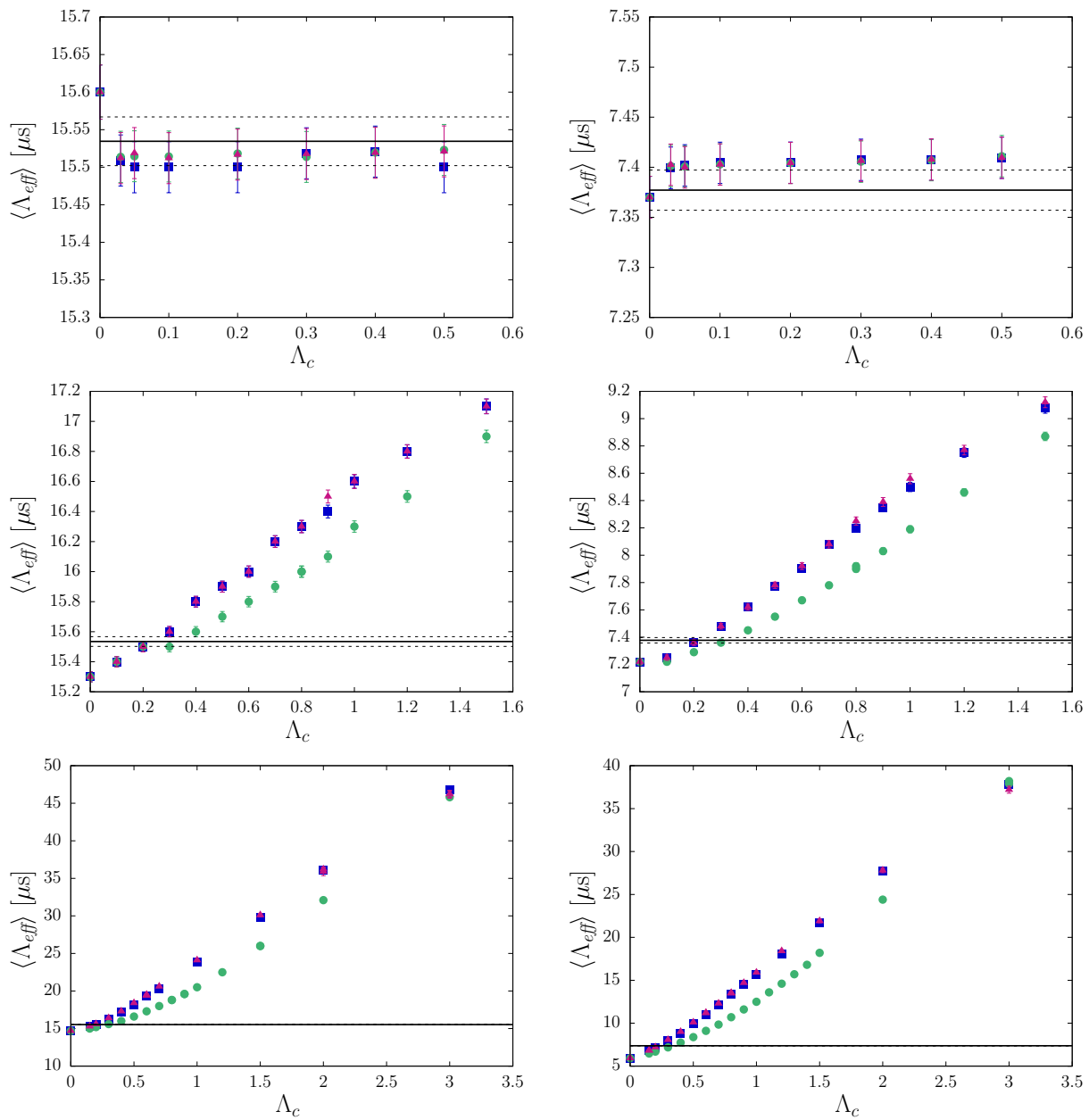
Figure 6.5: Evolution of the ensemble-averaged effective neutron generation time \langle \Lambda_{eff} \rangle as a function of the average correlation length \Lambda_c , for n = 1 (top), n = 7 (middle) and n = 17 (bottom). Left: UOX assembly. Right: MOX assembly. Blue squares denote the results for Poisson tessellations, red triangles for Box tessellations, and green circles for Voronoi tessellations. The limit case at \Lambda_c = 0 corresponds to the atomic mix model. The black solid line denotes \Lambda_{eff,0} , the result for the UOX assembly with intact fuel pins, which has been added for reference (dashed lines represent the 1\sigma statistical uncertainty).
