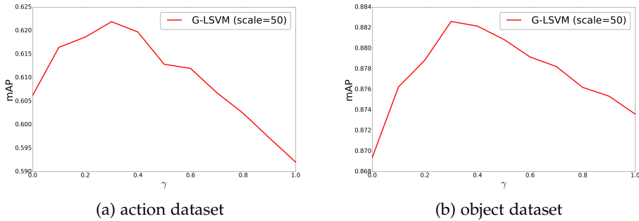
Figure 4.6: For scale = 50%, the effect of parameter \gamma .
