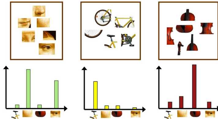
Figure 2.1: Bag of Visual Words (BoVW) scheme. (Credit: cs143 course of Brown University )
