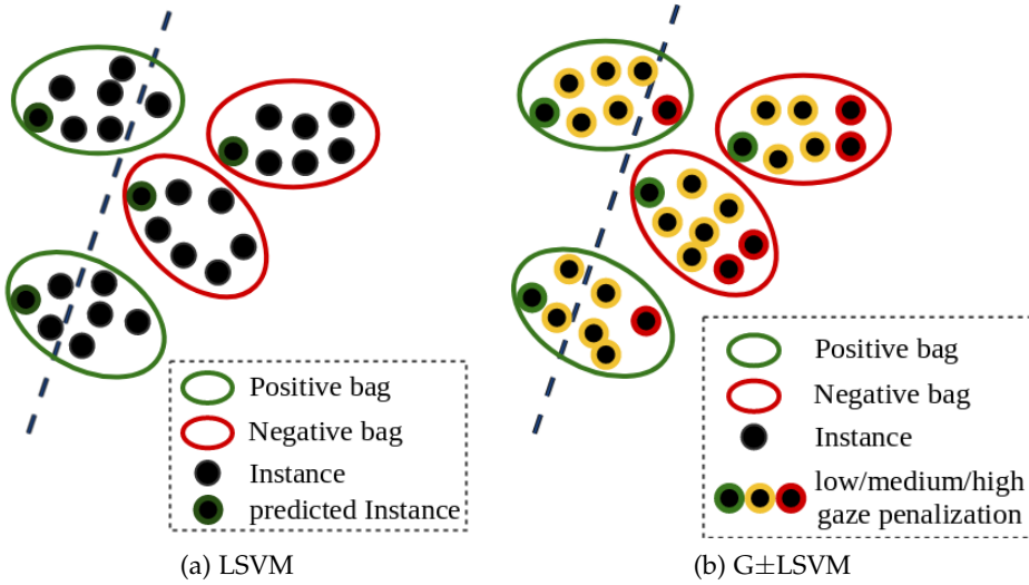
Figure 5.1: G±LSVM generalizes LSVM by penalizing background of positive image and foreground of negative image.
