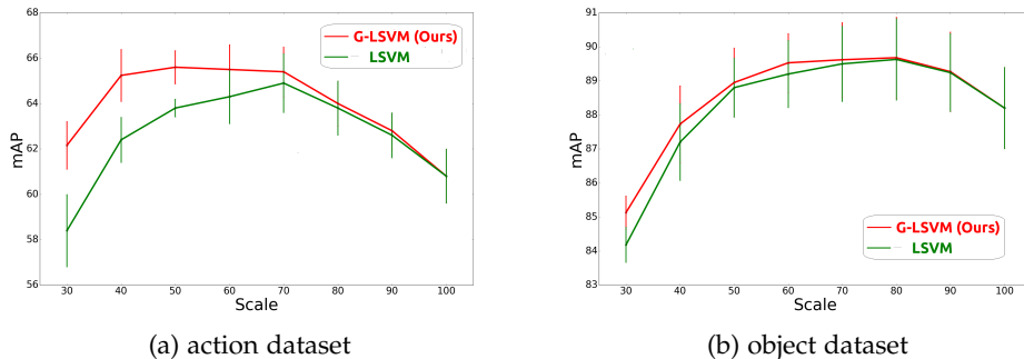
Figure 4.5: mAP(%) at different scales.
