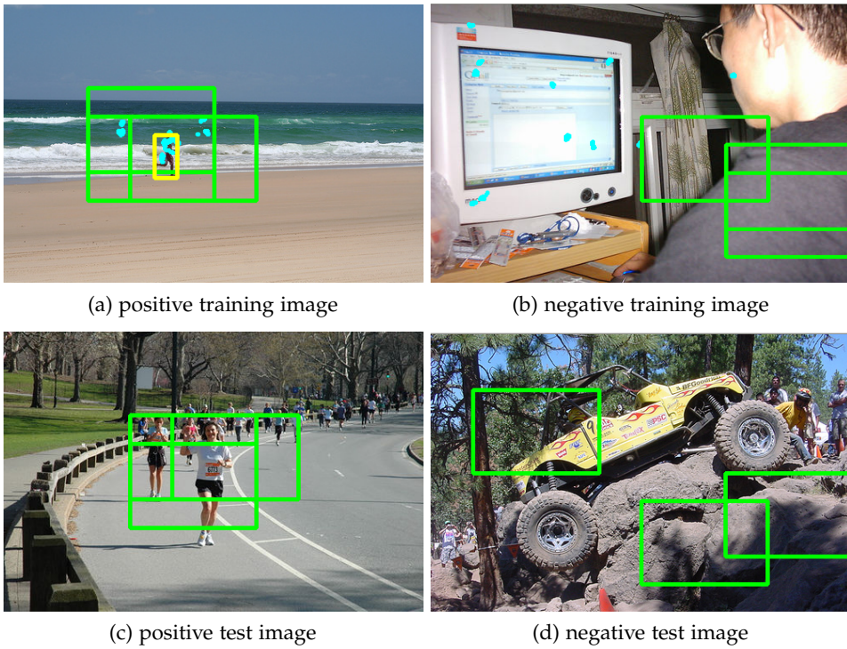
Figure 5.7: Localization results achieved by running model . (a)(b): training results, (c)(d): test results.
