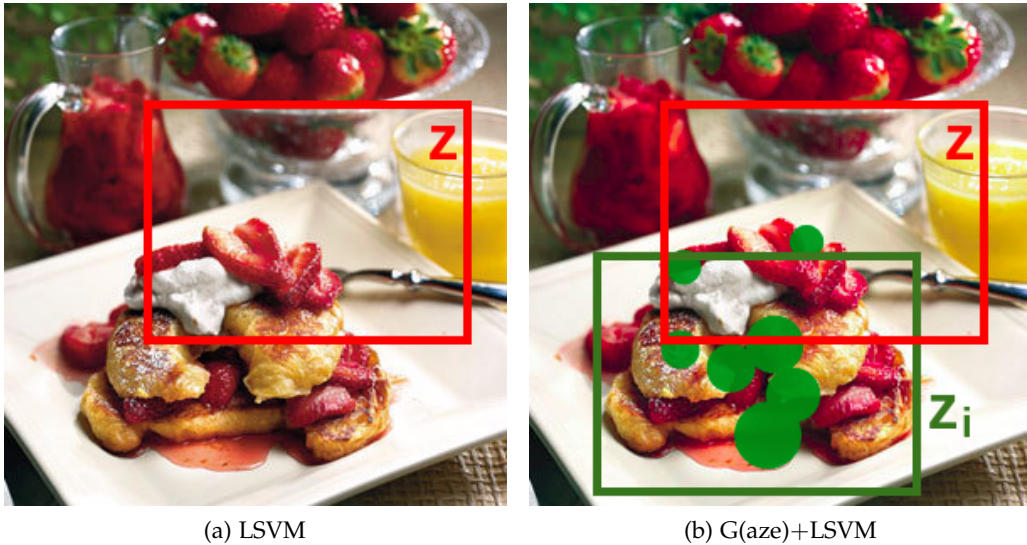
Figure 4.1: Gazes bias the selection of latent regions for LSVM. The interpretation is in the section 4.1.
