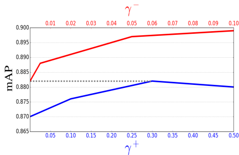
(c) POET dataset
