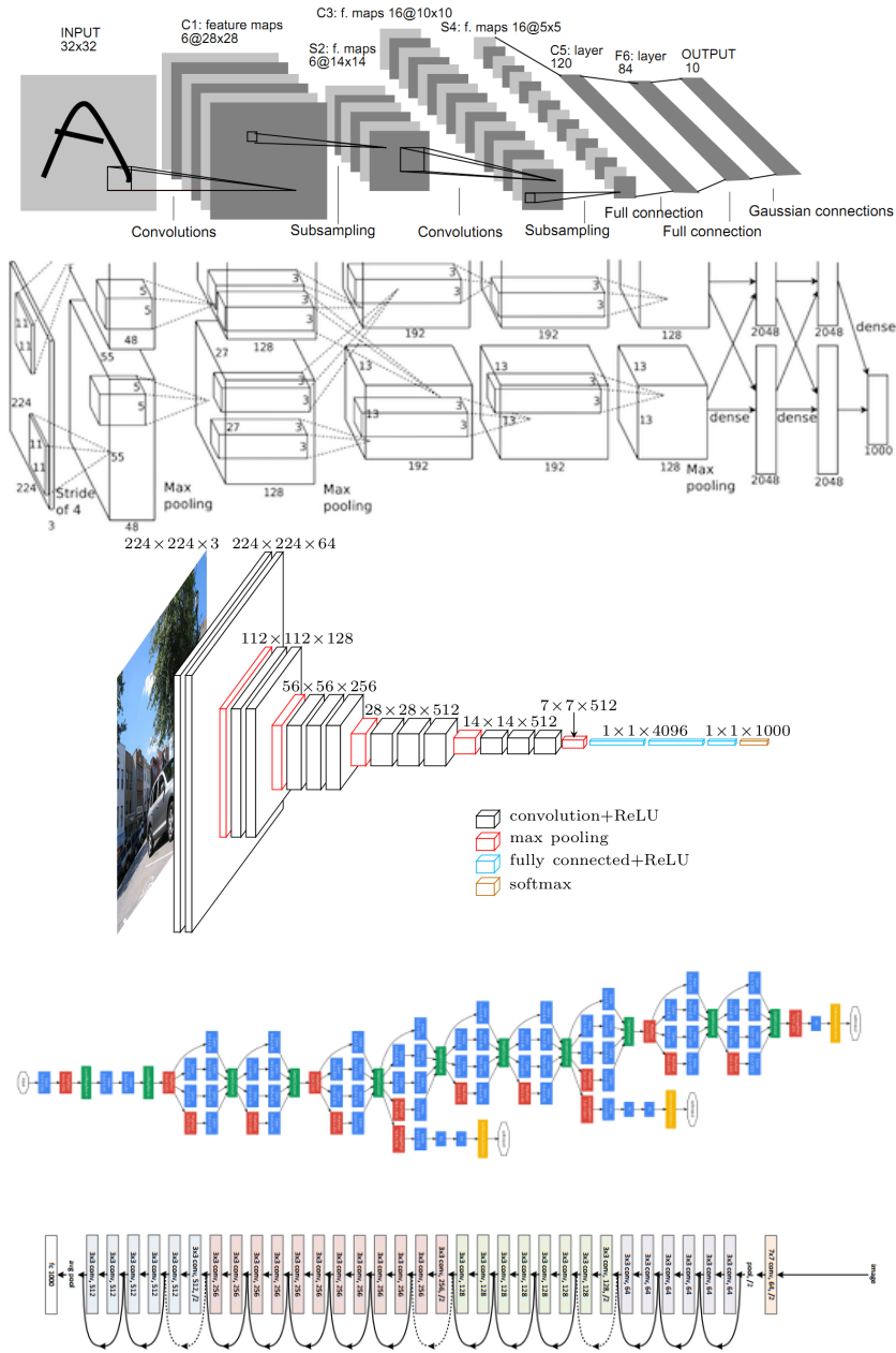
Figure 2.2: A list of classic deep convolutional neural networks. From top to bottom: LeNet-5 (LeCun et al. 1989), AlexNet (Krizhevsky, Sutskever, and Hinton 2012), VGG (Simonyan and Zisserman 2015), GoogleLeNet (Szegedy et al. 2015), Residual Neural Network (ResNet) (He et al. 2016).
