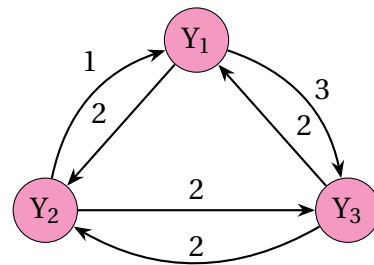
FIGURE 5.8 – Graphe \vec{G}_T
