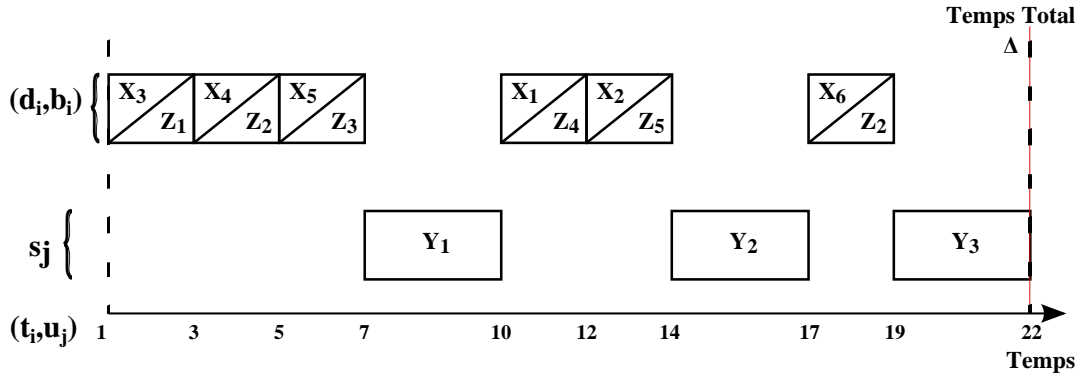
FIGURE 5.9 – I_3 -PSDPP - Solution de l'algorithme KAD
