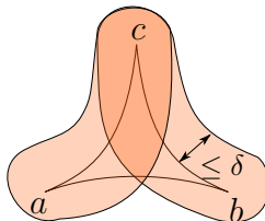
Figure 1.1 – Triangle \delta -fin.
