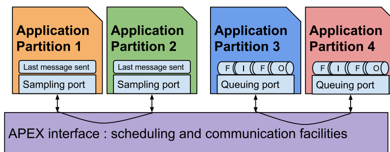
FIGURE 2.29 – La Communication inter Partition
