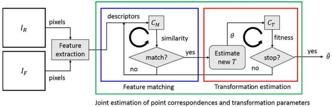
Figure 2.9: Schematic illustration of the feature-based image registration approach.
