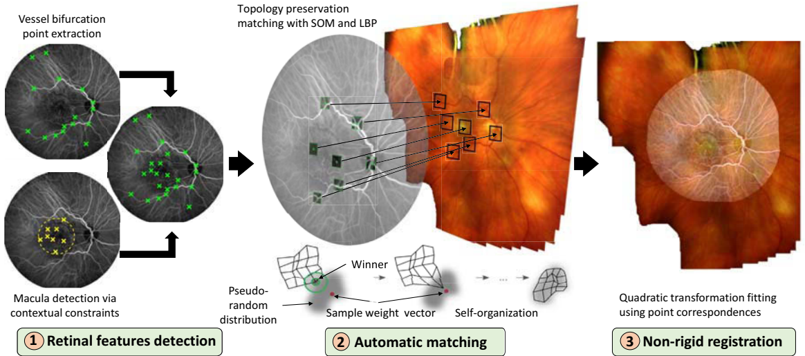
Figure 7.2: Method overview.
