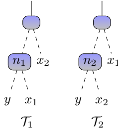
Figure 2.13 – Proof of Claim 1.
