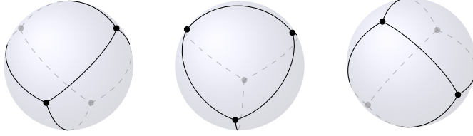
Figure 1.6 – The regular tetrahedron on the sphere.
