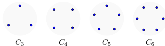
Figure 1.3 – Order types in convex position.
