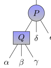
Figure 2.3 – A PQ-tree.
