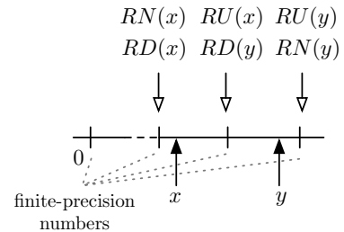
Figure 2.1: Illustration of three rounding modes of real numbers x and y .
