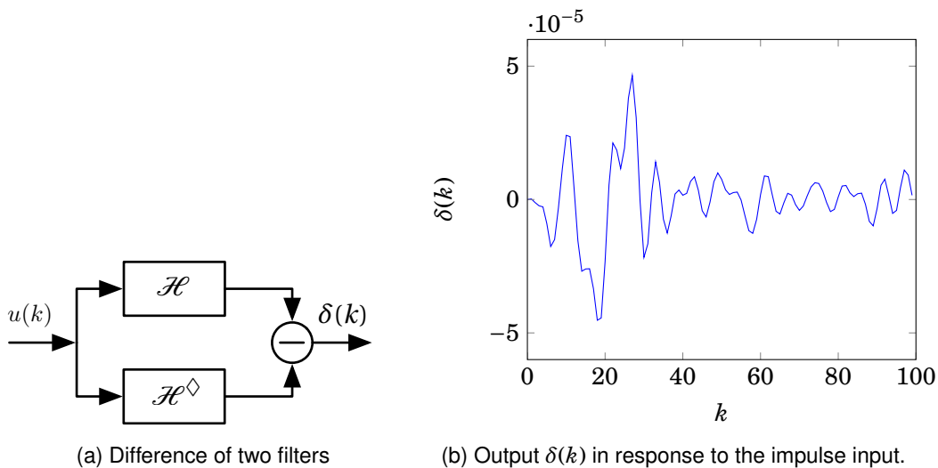
Figure 2.7: Demonstration of the classic error-model.
