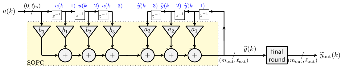
Figure 9.3: Abstract architecture for the direct form realization of an LTI filter
