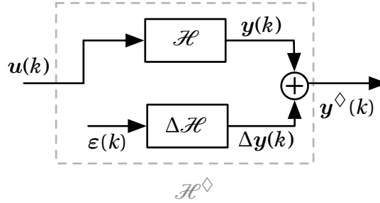
Figure 8.5: Implemented filter
