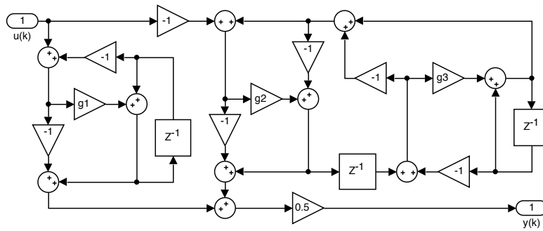
Figure 8.6: Implemented digital filter.
