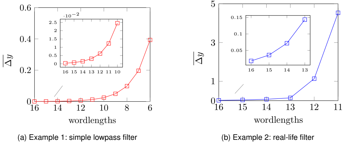
Figure 7.2: Evolution of the worst-case error in dependency with the wordlength constraints.
