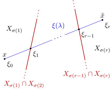
FIGURE 2.4 – Representation of the line segment connecting x and \tilde{x} .
