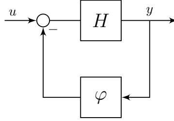
FIGURE 3.1 – Block diagram of the closed-loop system considered in Example 3.5
