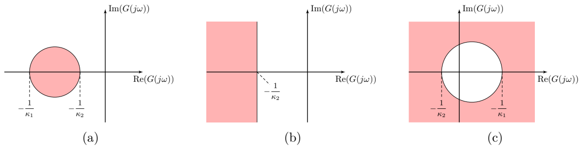
FIGURE A.3 – Graphical representation of the circle criterion when (a) \kappa_1 > 0 , (b) \kappa_1 = 0 and (c) \kappa_1 < 0 . The area in red represents the critical region.
