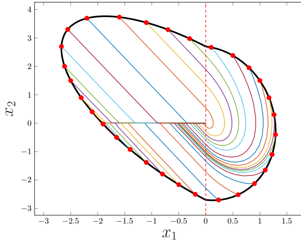
FIGURE 2.5 – A level curve of the piecewise-quadratic Lyapunov function obtained in Example 3.13, along with some trajectories of the PWA system.
