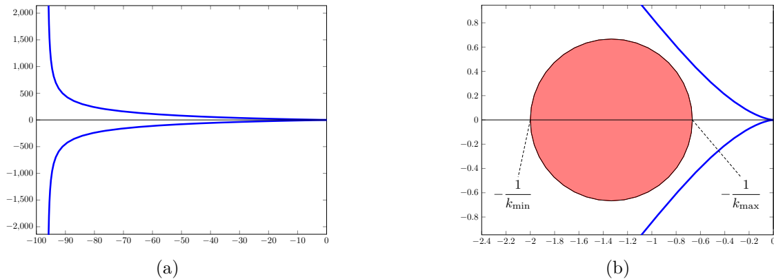
FIGURE 4.12 – Nyquist plot of k_b H , with k_0 = 23.4 , and application of the circle criterion (a) and zoom in (b) for the system in Example 4.36.
