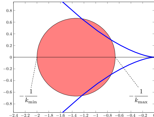
FIGURE 4.13 – Zoom over the Nyquist plot of k_b H , with k_0 = 70.2 , and application of the circle criterion for the system in Example 4.36.
