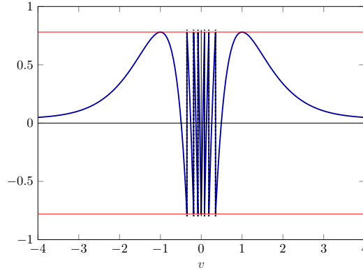
FIGURE 5.7 – Derivative of the approximation error \epsilon due to the PWA approximation computed in Example 5.11. The red lines indicate the bound \mathcal{L}_\epsilon = 0.7805
