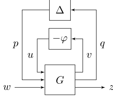
FIGURE 5.1 – Representation of the uncertain Lur'e system defined in (5.1).
