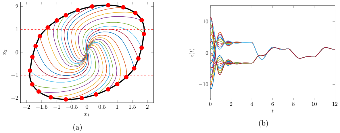
FIGURE 5.12 – Simulation of the system in Example 5.13 in the case of (a) different initial conditions with zero input and (b) different initial conditions with nonzero inputs in (5.17).
