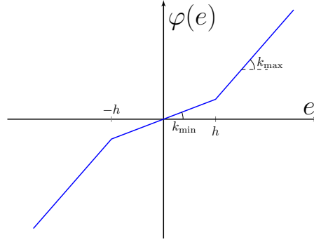
FIGURE 4.10 – Piecewise-affine nonlinearity \varphi in Example 4.36.
