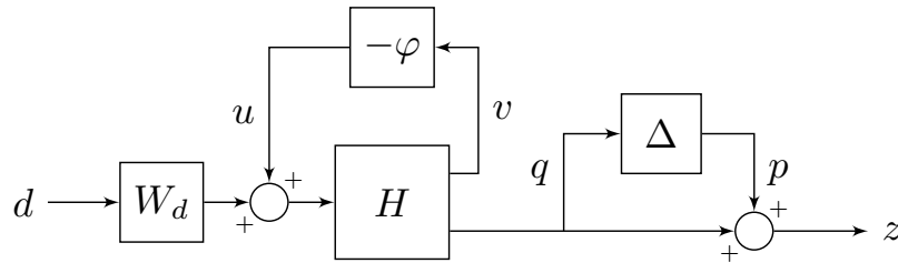
FIGURE 5.13 – Uncertain Lur'e system analyzed in Example 5.13.
