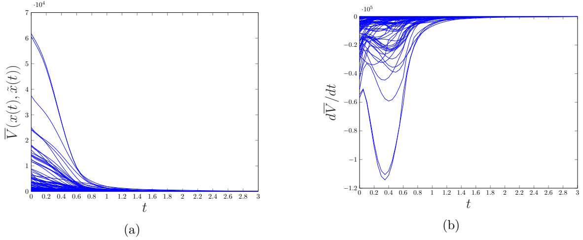
FIGURE 3.4 – Plots of (a) the incremental Lyapunov function and (b) its derivative in Example 3.13.
