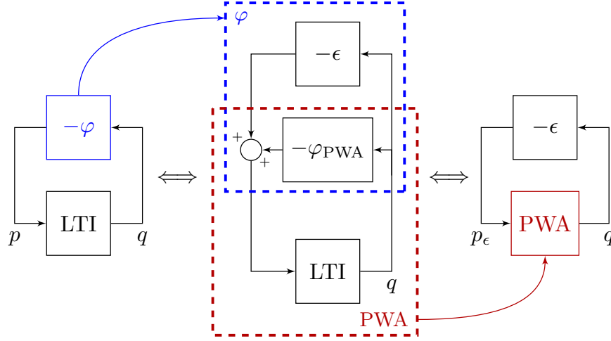
FIGURE 5.2 – Block diagram illustrating the approach proposed in this chapter (the performance channels w and z , as well as the uncertainty \Delta , are omitted for clarity).
