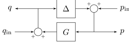
FIGURE 4.3 – Feedback interconnection (G, \Delta) .
