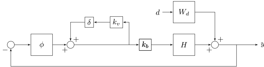
FIGURE 4.11 – Block diagram of the closed-loop system in Example 4.36.
