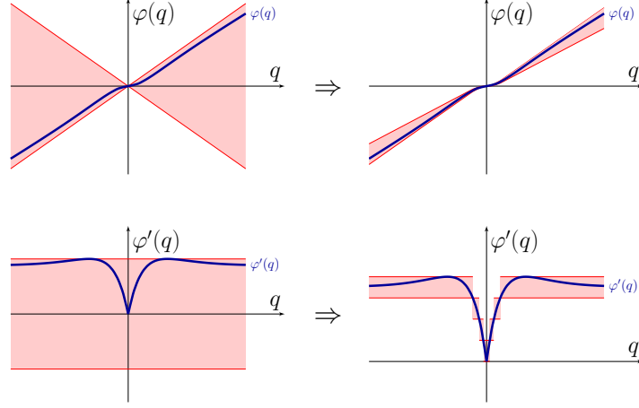
FIGURE 5.3 – Comparison between the sectors describing the nonlinearity \varphi for the incremental circle criterion (left) and the piecewise-affine approach (right).
