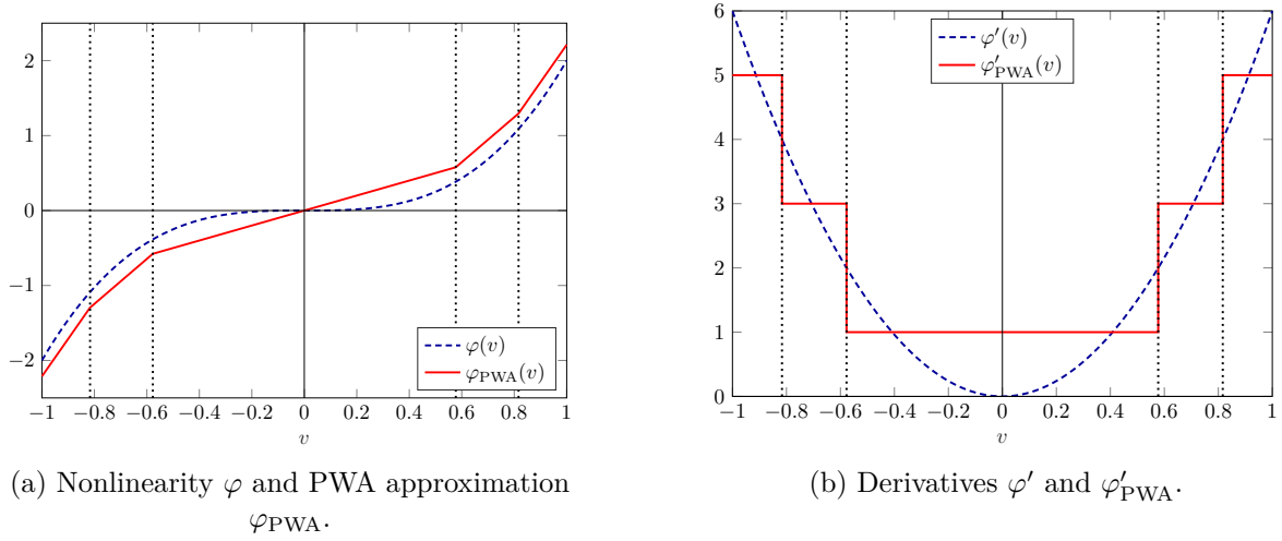
FIGURE 5.9 – Nonlinearity \varphi and piecewise-affine approximation \varphi_{\text{PWA}} computed in Example 5.12.
