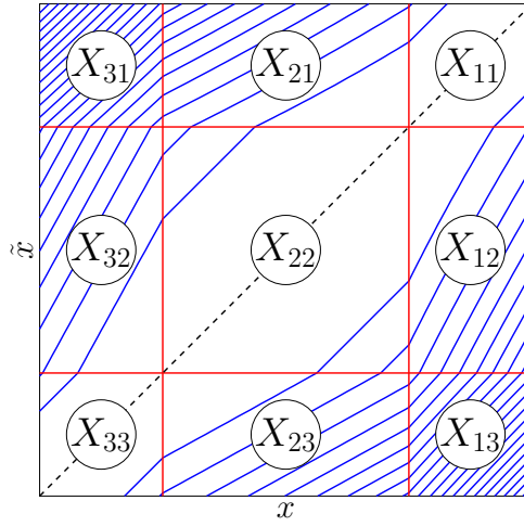
FIGURE 3.2 – Contour plot of the incremental Lyapunov function for the augmented system in Example 3.5 illustrating its piecewise-quadratic structure
