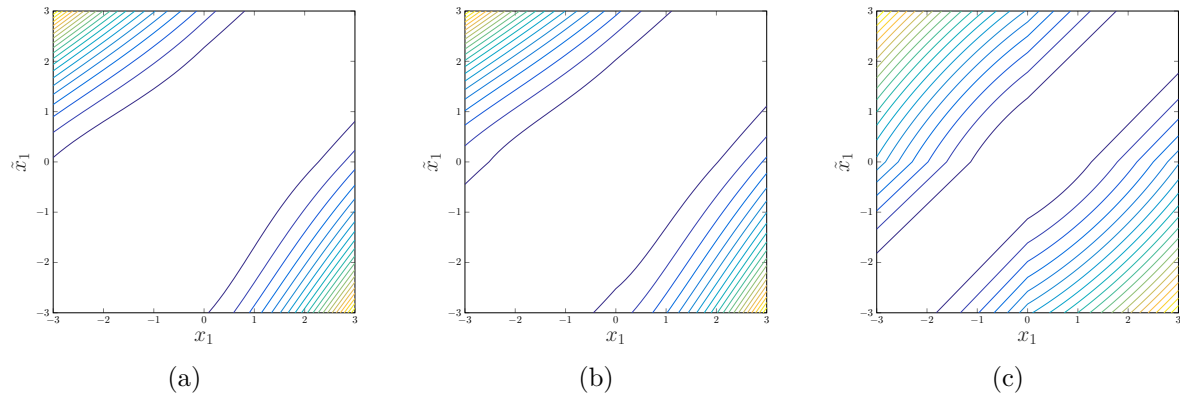
FIGURE 3.6 – Level curves of the intersections of \bar{V} with the plane x_1\text{-}\tilde{x}_1 for: (a) x_2 = \tilde{x}_2 = 0 . (b) x_2 = \tilde{x}_2 = 3 . (c) x_2 = \tilde{x}_2 = 30 .
