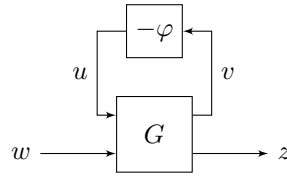
FIGURE A.1 – Lur'e system described by (A.1).
