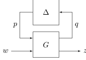
FIGURE A.5 – G - \Delta structure.
