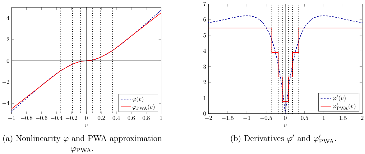
FIGURE 5.6 – Nonlinearity \varphi and piecewise-affine approximation \varphi_{\text{PWA}} computed in Example 5.11.
