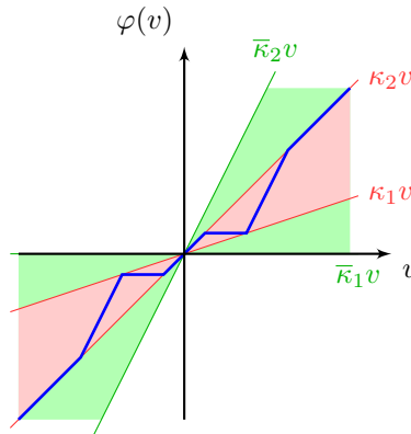
FIGURE A.4 – Sector \text{Sect}(\kappa_1, \kappa_2) and incremental sector \text{Sect}_\Delta(\bar{\kappa}_1, \bar{\kappa}_2) containing a given piecewise-affine nonlinearity.
