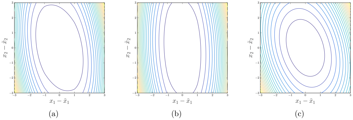
FIGURE 3.5 – Level curves of the intersections of \bar{V} with the plane (x_1 - \tilde{x}_1) - (x_2 - \tilde{x}_2) for: (a) x_1 + \tilde{x}_1 = -1 , x_2 + \tilde{x}_2 = -3 . (b) x_1 + \tilde{x}_1 = 1 , x_2 + \tilde{x}_2 = 1 . (c) x_1 + \tilde{x}_1 = -3 , x_2 + \tilde{x}_2 = -3 .
