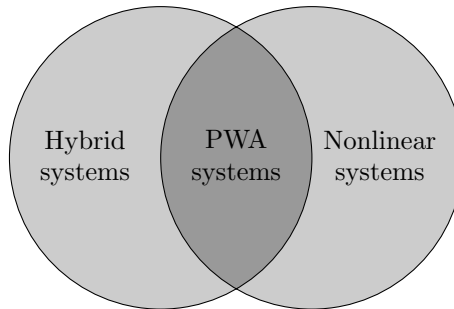
FIGURE 2.2 – Piecewise-affine systems are special cases of hybrid and nonlinear systems
