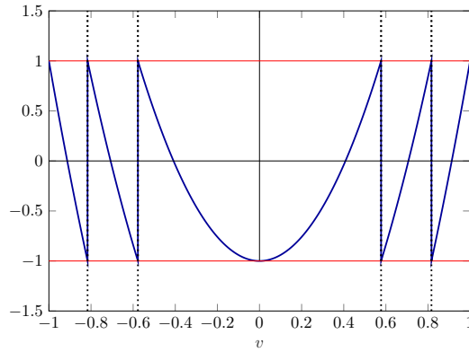
FIGURE 5.10 – Derivative of the approximation error \epsilon due to the PWA approximation computed in Example 5.12. The red lines indicate the bound L_\epsilon = 1 .
