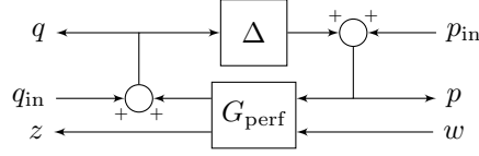
FIGURE 4.4 – Feedback interconnection (G_{\text{perf}}, \Delta) .
