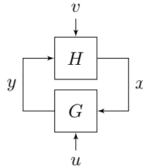
FIGURE 4.6 – Feedback interconnection (4.17).
