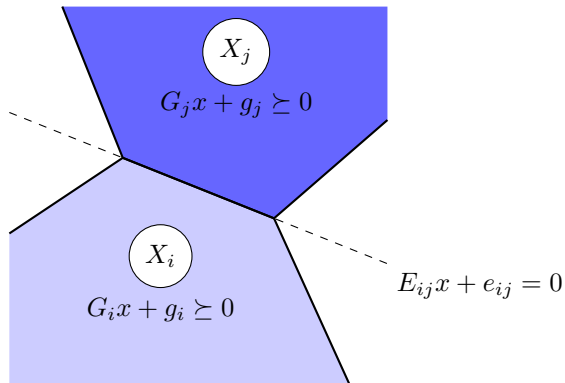
FIGURE 2.1 – Polytopic partition of the state space
