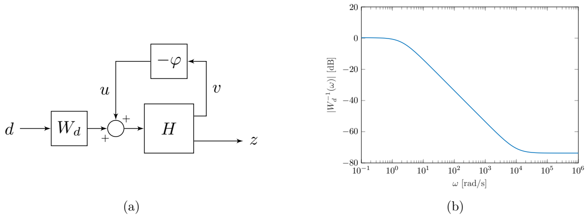
FIGURE 5.11 – (a) Lur'e system analyzed in Example 5.13 and (b) Bode plot of W_d^{-1}(j\omega) showing its low-pass behavior.
