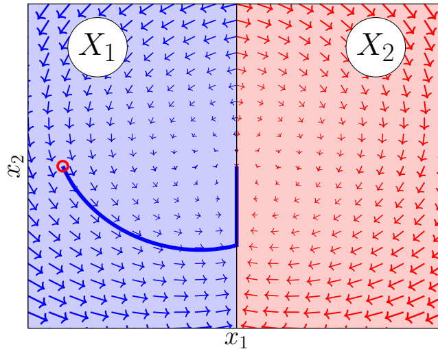
FIGURE 2.3 – Sliding mode trajectory.
