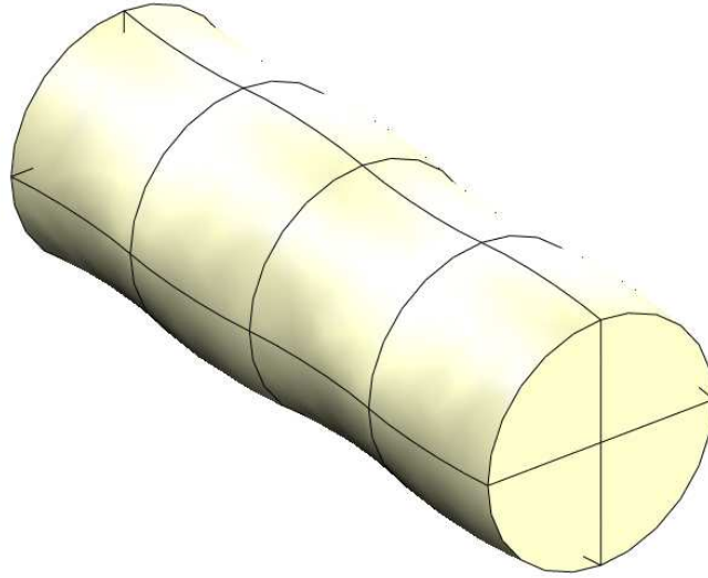
Figure 2.6 – 3D shape with a lower dissipated energy than the cylinder. Credits : A. Henrot and Y. Privat [83]
