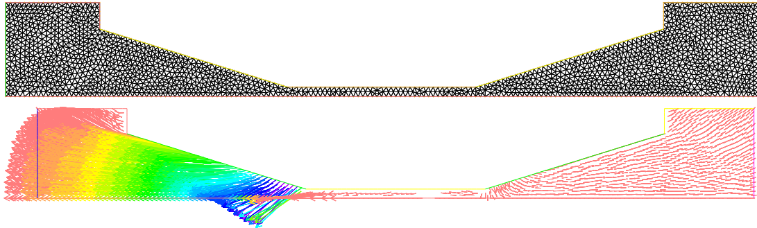
Figure 3.14 – Top : initial mesh. Bottom : displacement field associated to the first iteration
