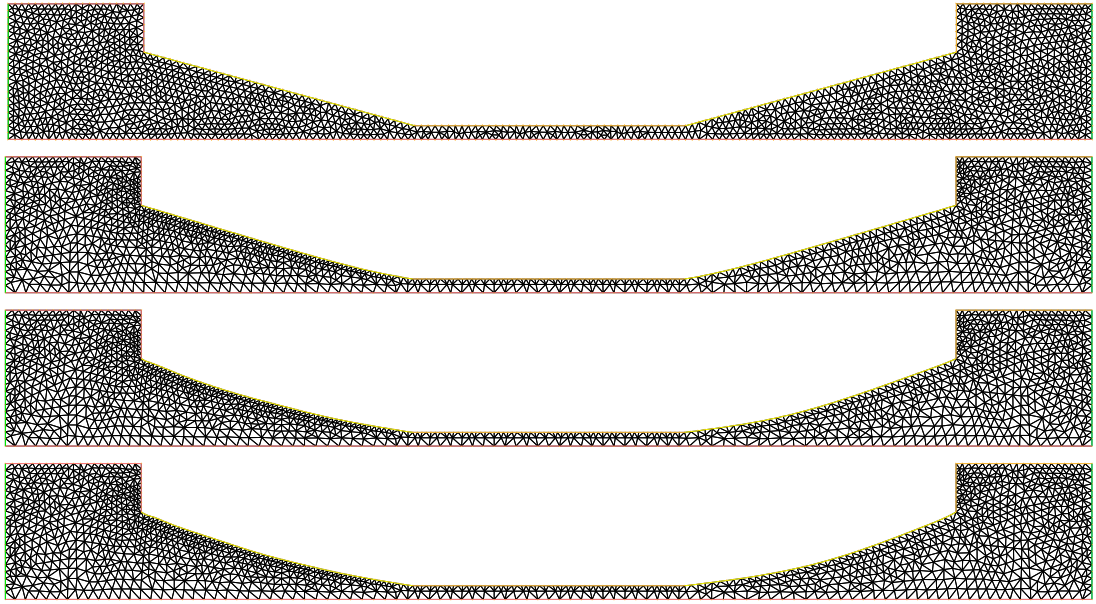
Figure 3.5 – From top to bottom : mesh at iterations 0, 45 and 85 for Test-case 1.
