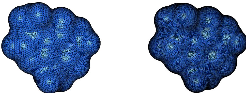
Figure 10: The mesh (right) of caffeine before remeshing with r_p = 1\text{\AA} and the mesh (left) after remeshing with the MMGS tool.
