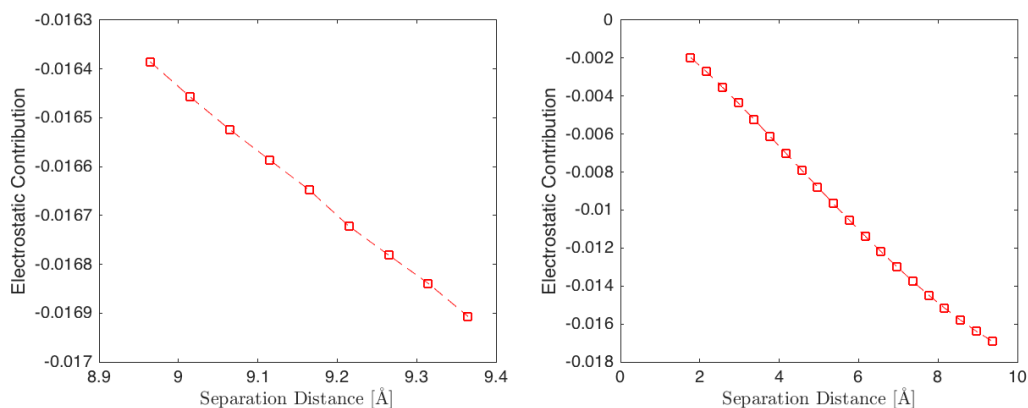
Figure 20: Electrostatic contribution of hydrogen-fluoride with respect to the separation distance between the atomic centers with parameters \ell_{\max} = 11 , N_{\text{leb}} = 1202 , N = 20 , N_{\text{igl}} = 40 , \varepsilon_s = 8.93 , r_p = 1.5\text{\AA} , r_0 = 0\text{\AA} . On the left, the separation distance varies between 8.96\text{\AA} and 9.36\text{\AA} where the topology of the SES changes as showed in Figure 19. On the right, the separation distance varies in a larger range.
