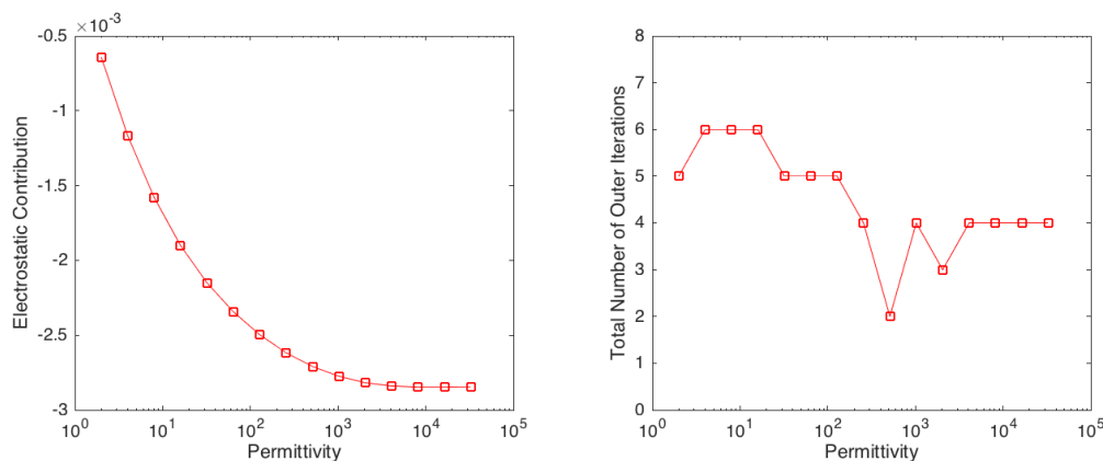
Figure 15: The left figure shows the electrostatic contribution to the solvation energy of hydrogen-fluoride when the solvent dielectric constant \epsilon_s increases; the right figure plots the total number of outer iterations to reach the stopping criterion \text{To1} with respect to \epsilon_s . The following parameters are used: \ell_{\max} = 11 , N_{\text{leb}} = 1202 , N = 20 , N_{\text{lgl}} = 50 , r_p = 1.5\text{\AA} , r_0 = 1\text{\AA} .
