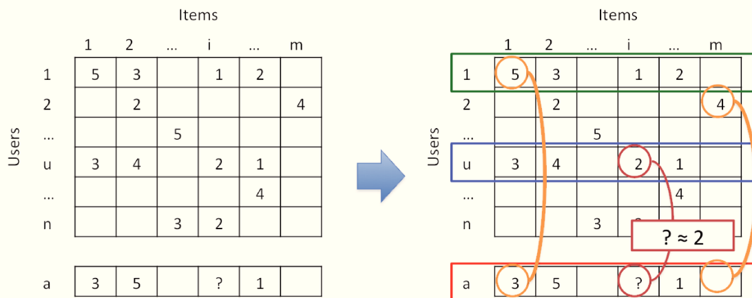
Figure 2.1: Collaborative Filtering matching process
