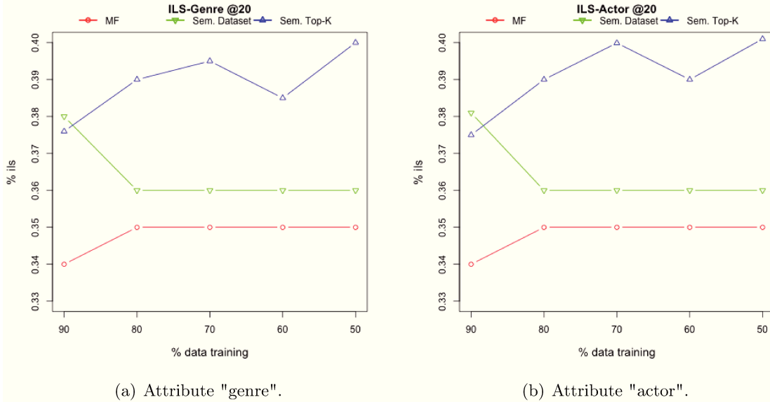
Figure 4.7: ILS metric comparisons.
