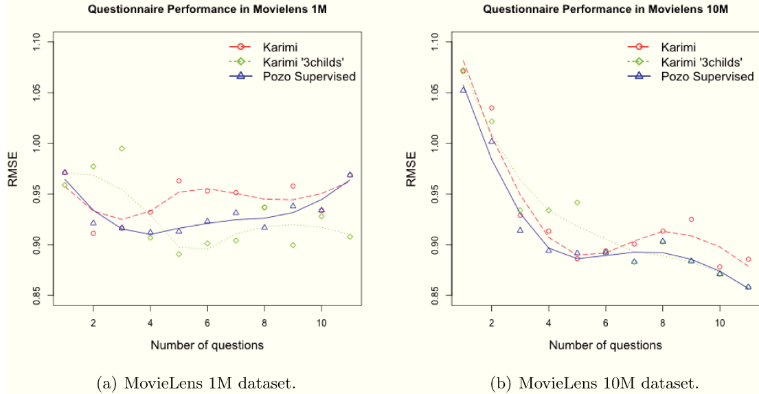
Figure 6.6: Questionnaire performance in RMSE.
