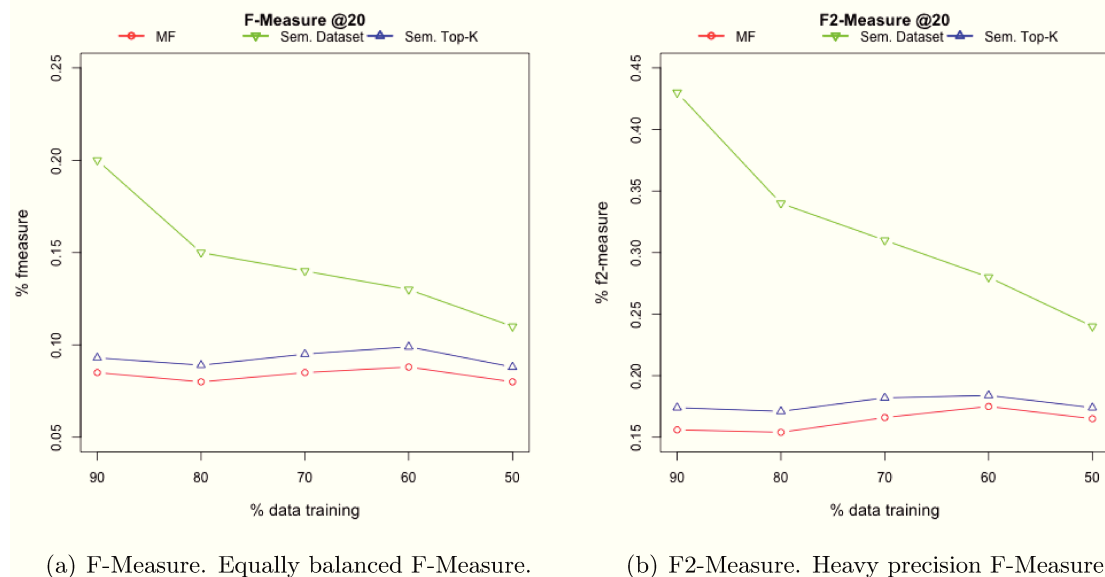
Figure 4.6: F-Measures for top 20 items.
