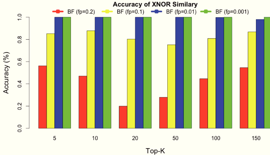
Figure 5.11: Accuracy of the Bloom Filter Similarity Model against the Vector Similarity Model. This similarity uses the XNOR operation.
