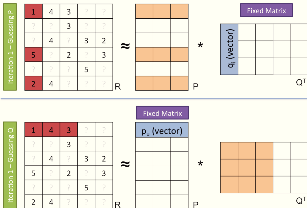
Figure 3.1: Alternating Least Squares technique. Methodology and scalability.
