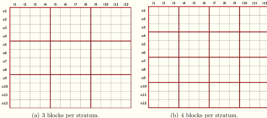
Figure 3.3: Diving the matrix R into independent blocks per stratum
