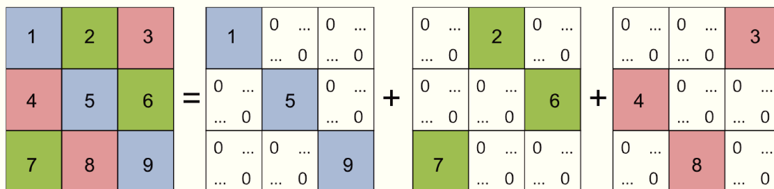
Figure 3.2: Stratification and Block decomposition. Blocks 1,5,9 do not share rows neither columns, thus, they form a stratum to run in parallel. Once computed, another stratum (2,6,7 or 3,4,8) can run. Single iteration.
