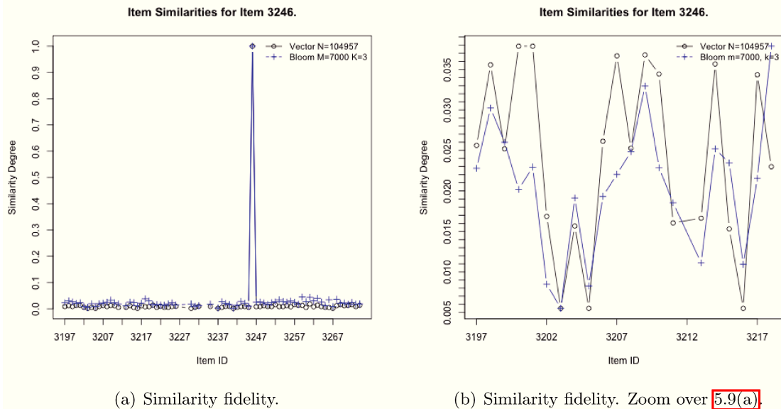
Figure 5.9: Bloom Filter ( m=7000 , k=3 ). Trade-Off for a Bloom Similarity Model.
