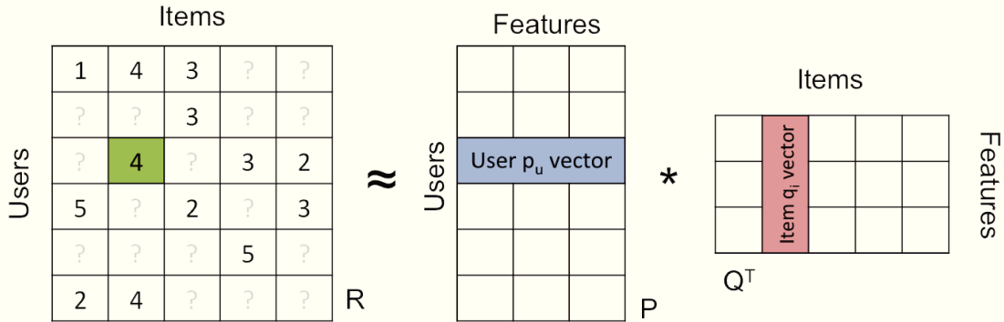
Figure 2.2: Matrix factorization of R (users, items, ratings) into P (users, features) and Q (items, features).
