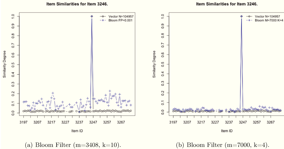
Figure 5.8: Trade-Offs for a Bloom Similarity Model.
