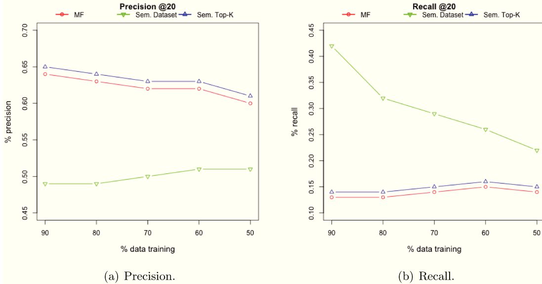
Figure 4.5: Precision and Recall metrics comparisons regarding a top-20 items.
