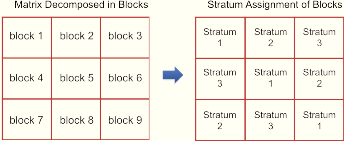
Figure 3.4: Block Stratum Assignment technique.
