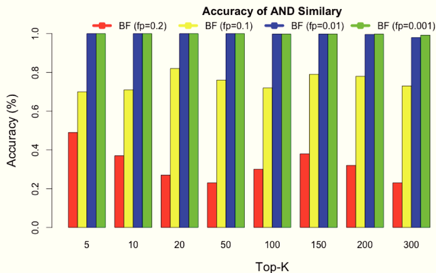
Figure 5.10: Accuracy of the Bloom Filter Similarity Model against the Vector Similarity Model. Bloom Filters with fewer false positive values achieve better accuracy in tops comparisons.
