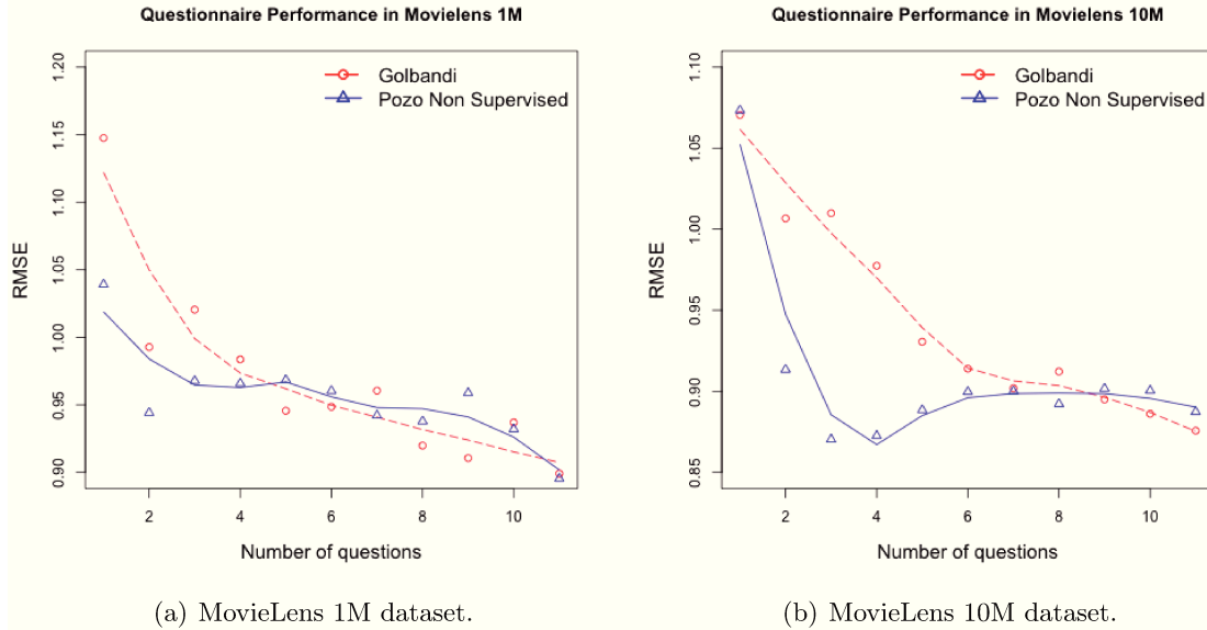
Figure 6.5: Questionnaire performance in RMSE.
