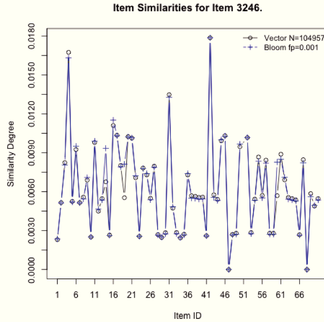
Figure 5.7: Degree of Similarity of the item 3246 with several items. Bloom Filter ( n=237 , fp=0.001 ) has been reconstructed into a vector of size N .
