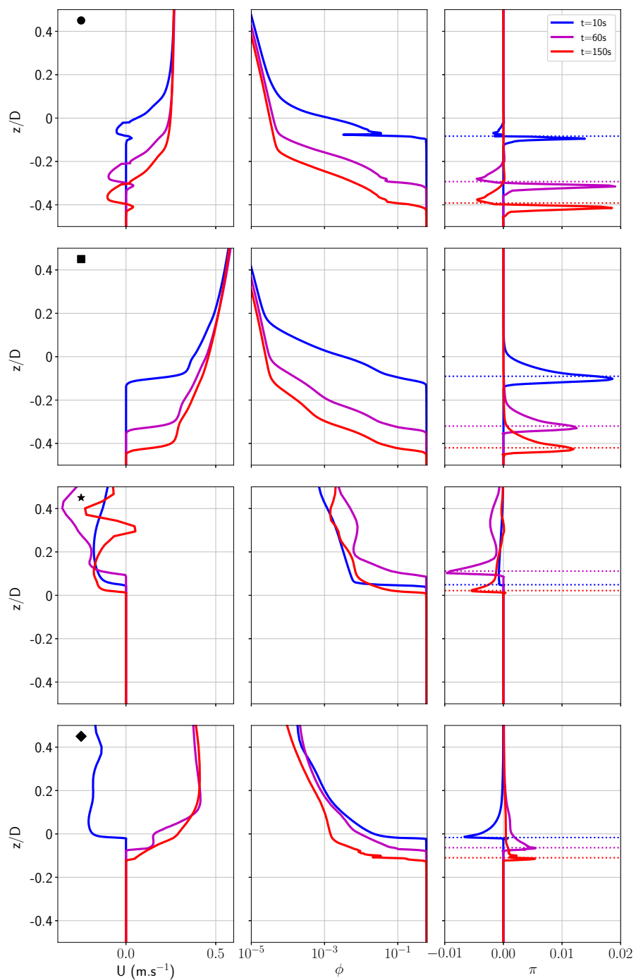
FIGURE 5.21: Vertical profiles of mixture velocity ( U ), sediments concentration ( \phi ) and dimensionless sediments flux ( \pi ) at different locations around the cylinder and at t=10s (blue), t=60s (magenta) and t=150s (red). The location of each profile is shown in subfigure 5.20. The horizontal dotted line in the dimensionless sediments flux panels represent the vertical elevation of the sediments concentration \phi=0.08 .
