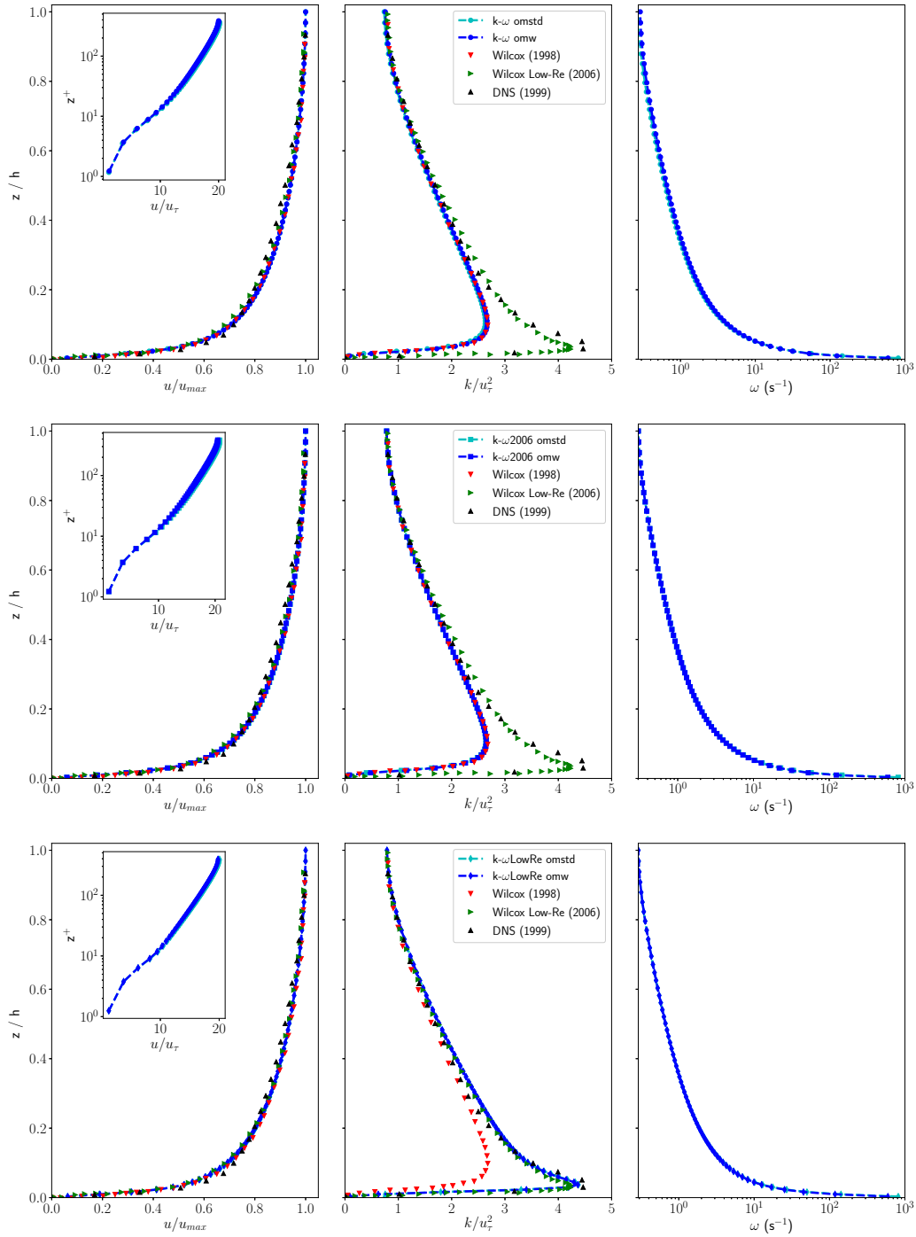
FIGURE 4.4: Comparison between SedFoam and Moser et al. (1999); Wilcox (1998, 2008) for velocity, TKE and specific dissipation rate profiles using the k- \omega (top panel), k- \omega 2006 (middle panel), and k- \omega low-Reynolds (bottom panel) turbulence models and different wall functions. Here, z^+ \approx 1 .
