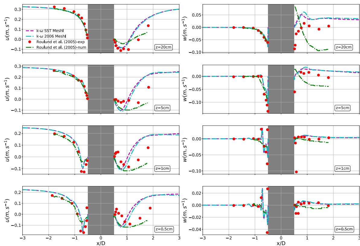
FIGURE 5.3: Horizontal and vertical velocities, u (left panel) and w (right panel), in the plane of symmetry at different distances from the bed for the two turbulence models k\text{-}\omega 2006 and SST using MeshI.
