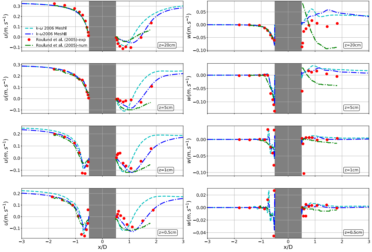
FIGURE 5.4: Horizontal and vertical velocities, u (left panel) and w (right panel), in the plane of symmetry at different distances from the bed for the k-\omega 2006 turbulence model with MeshI and MeshII.
