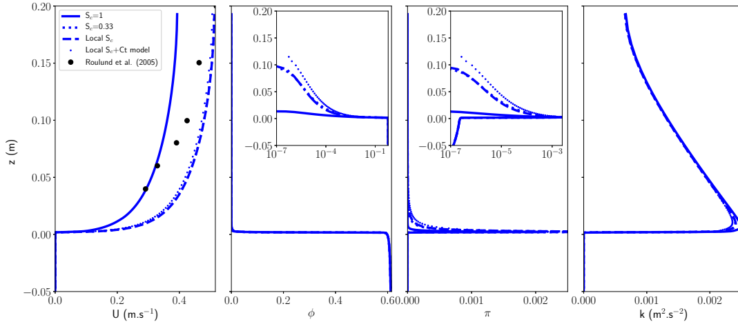
FIGURE 4.10: Velocity, sediment concentration \phi , sediment flux and TKE profiles using the k - \omega 2006 turbulence model for a two-phase flow simulation including sediment. Here, \theta=0.19 . Experiment (black dots) correspond to the velocity profile measured by Roulund et al. (2005).
