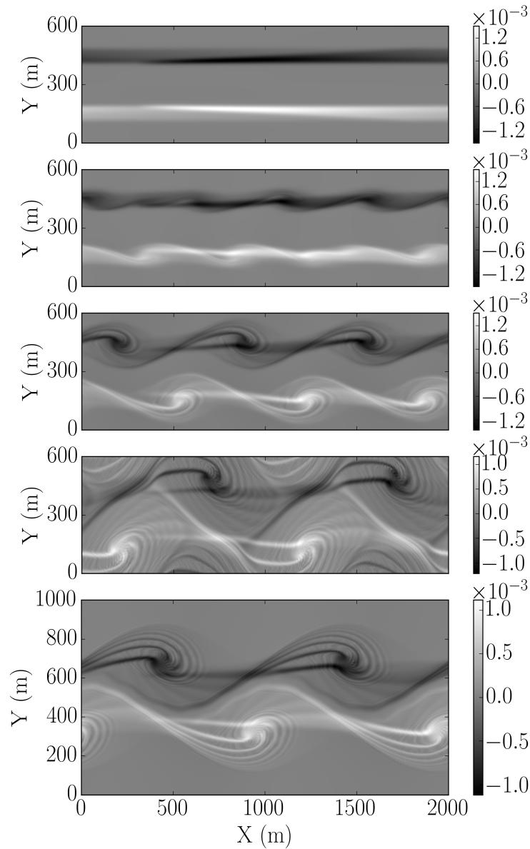
FIGURE 2.3: 2D vorticity fields after 14 days of dynamics for H15, (a) H20 (b), H30 (c), H50 (d) and H50w (e). Increasing the water layer thickness leads to a generation of two types of oceanic instabilities, distinct and interacting ones. This instabilities generation is controlled by the wake stability parameter S .
