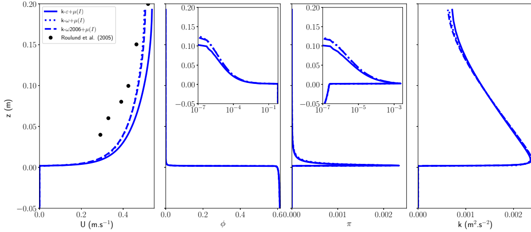
FIGURE 4.9: Velocity, sediment concentration \phi , sediment flux and TKE profiles using the k- \varepsilon , the k- \omega and the k- \omega 2006 turbulence model for a two-phase flow simulation including sediment. Here, \theta=0.19 . Experiment (black dots) correspond to the velocity profile measured by Roulund et al. (2005).
