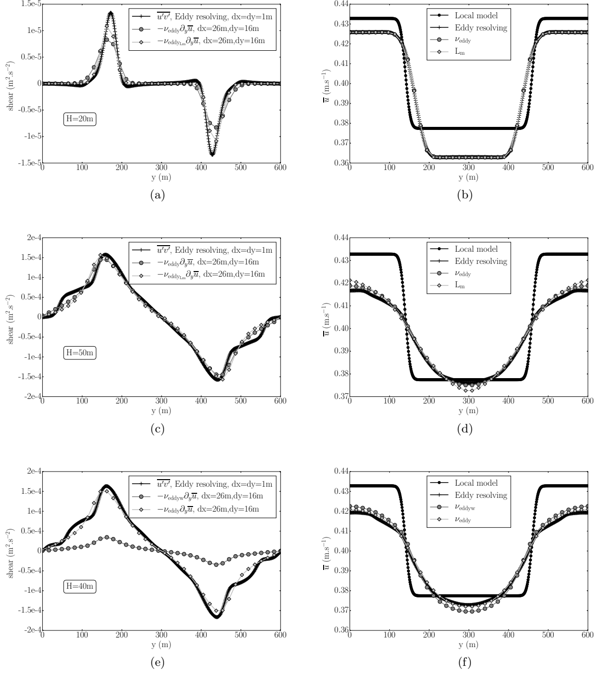
FIGURE 2.9: Confined runs y-direction transect at x=1300\text{m} of the shear (a,c,e) and mean velocity field \bar{u} (b,d,f) for different water layer thicknesses. Eddy resolving computations (cross) and the three parametrizations are represented. For the 40m water layer thickness case (e,f), the circles symbols show the results obtained with an eddy viscosity computed from the non-confined configuration, when the diamonds curve is obtained with a eddy viscosity computed from the confined configuration. The results are satisfactory on the mean velocity field \bar{u} , but they are incorrects on the shear.
