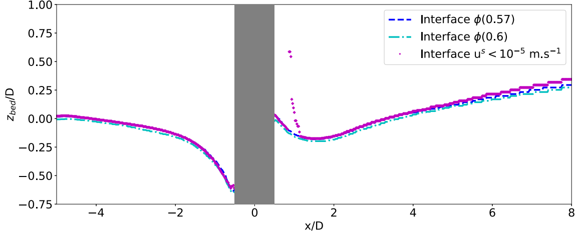
FIGURE 5.11: Bed elevation along the x-axis after t=600s of dynamics using different interface determination criterion : blue ( \phi=0.57 ), cyan ( \phi=0.6 ), magenta ( \sqrt{u^{s2}} < 10^{-5} ).
