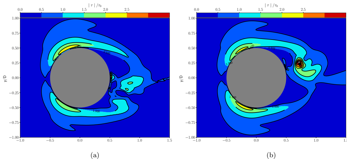
FIGURE 5.9: t=60\text{s} . Bed Shear Stress amplification magnitude in the Rigid-Bed case with MeshA (a), and MeshB (b).
