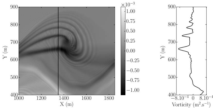
FIGURE 2.6: Zoom (a) and transect along the y-direction (b) of an eddy presented in figure 2.3, for the H50w case. The spaghetti-type structure of the vorticity field induced by atmospheric wake forcing and periodic boundary conditions but also the decaying vorticity intensity of the rotated filaments are clearly identifiable in the transect plot.
