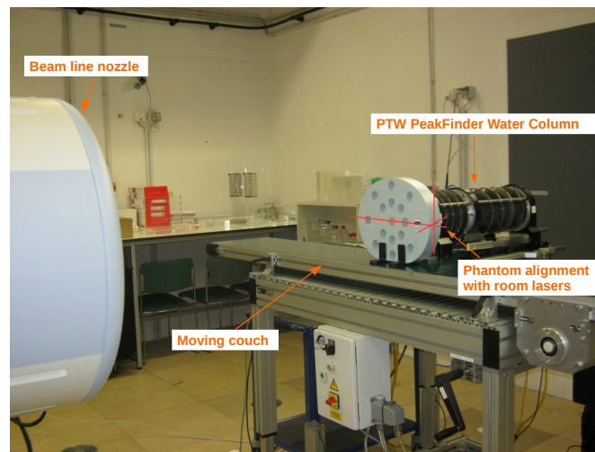
Figure C.1: Experimental setup to determine the Bragg Peak position
