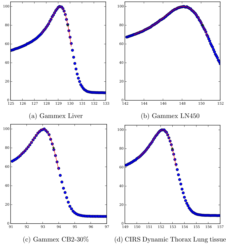
Figure C.2: Measured depth-dose distributions (dots), fifth degree polynomial fit in the 70% proximal to distal region (red line) and range position (green star) at the 80% distal edge.
