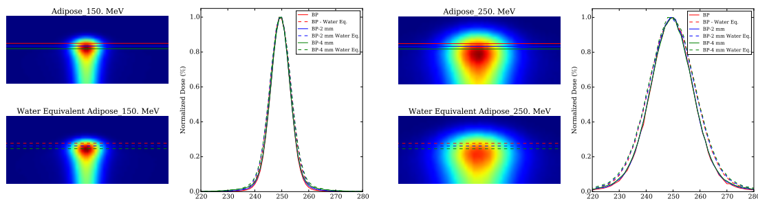
Figure D.1: Transverse dose profiles at the Bragg Peak (BP) position (red), at the BP-2 mm (blue) and at the BP-4 mm (green) for the adipose tissue (solid line) and the water equivalent adipose tissue (dashed line) at 150 MeV (left) and 250 MeV (right).
