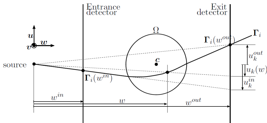
Figure 6.1: Schematic top view of the proton CT scanner used in this study. u and v define the orientation of the detectors, whereas \omega defines the source-to-isocenter direction. \Gamma_i(\omega^{in}) , \Gamma_i(\omega^{out}) and \Gamma_i represent the entrance position, the exit position and the most likely path, respectively. Figure extracted from [Quiñones, 2016].
