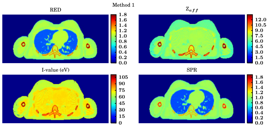
Figure 4.6: From top to bottom and from left to right: the RED and Z_{eff} images are the DECT outputs used by the first calibrated relation to estimate the SPR from DECT data. The I -value image is obtained from the empirical relationship between Z_{eff} and \ln I_m , and the SPR image using Bethe's equation without correction terms. Images relative to the situation without noise in the projections.
