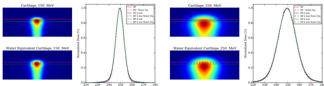
Figure D.2: Transverse dose profiles at the Bragg Peak (BP) position (red), at the BP-2 mm (blue) and at the BP-4 mm (green) for the cartilage tissue (solid line) and the water equivalent cartilage tissue (dashed line) at 150 MeV (left) and 250 MeV (right).
