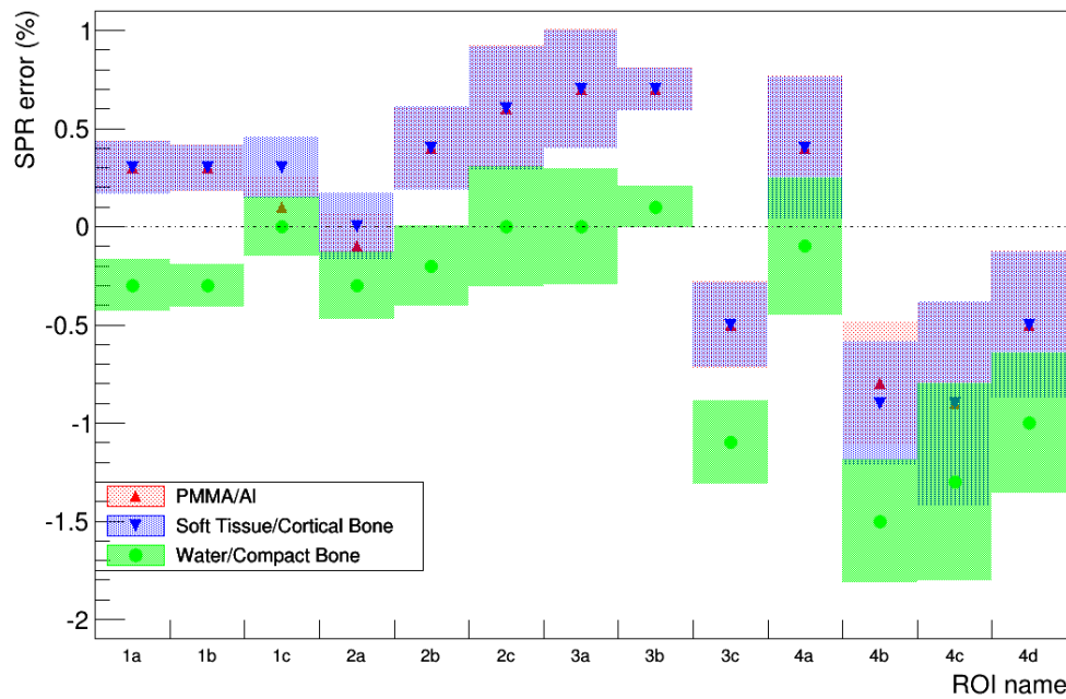
Figure 5.8: Relative SPR errors for each of the thirteen ROIs (see Figure 4.11 for the placement of the ROIs on the four ICRP slices) obtained with each decomposition basis: PMMA and aluminum, soft tissue and cortical bone, and water and compact bone.
