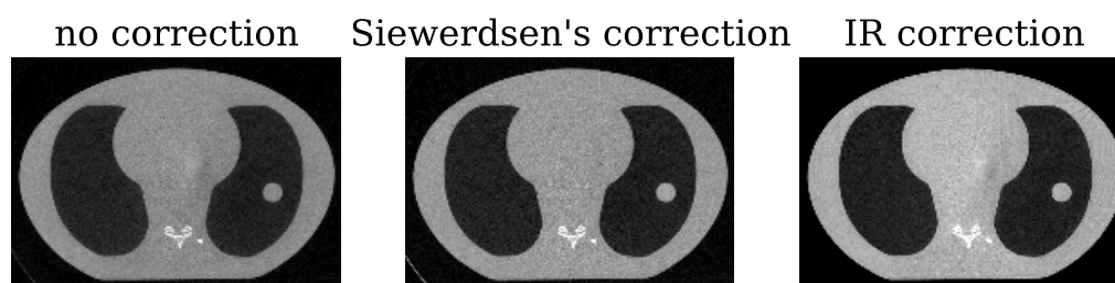
Figure 3.13: Comparison of reconstructed CT images without scatter correction (left), scatter corrected using Siewerdsen's method (middle) and with the IR scatter correction implemented at the time of the experiment (right). Colorbar from [0, 0.3] \text{ cm}^{-1} .
