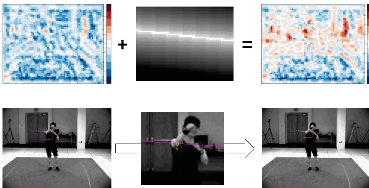
Fig. 6.3 Top : Epipolar energy map ( center ) is added to the initial feature response map ( left ), where final energy map for part estimation is seen on the right. Bottom left : Estimated position for the part, without the geometric constraint. Bottom center : Close up display of displacement of the part position towards the magenta epipolar line, where old position is marked with a green cross and new position is marked with a yellow circle. Bottom right : Part position is estimated jointly, this time considering the geometric consistency.
