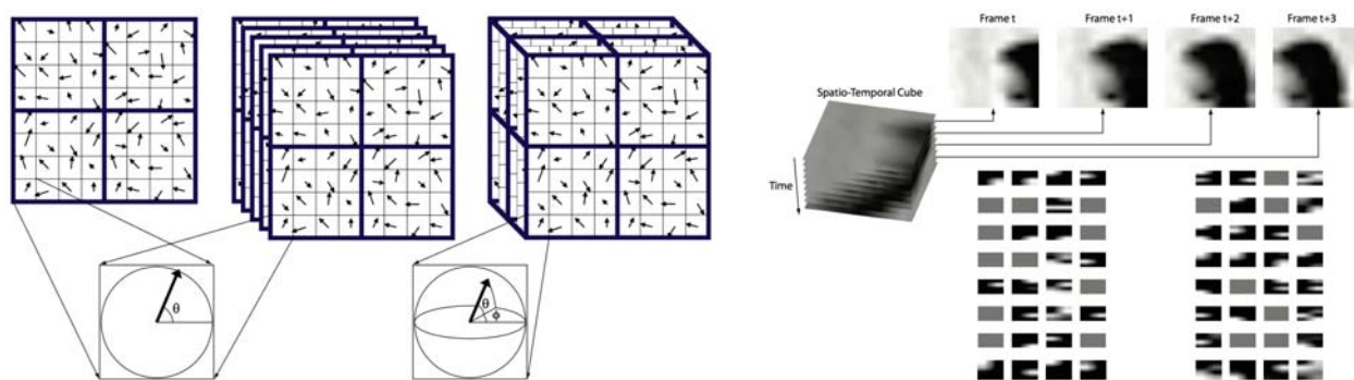
Fig. 2.3 Left : SIFT3D feature descriptor, illustrated as an extension of SIFT. Right : Computation of SIFT3D and descriptors before and after the reorientation. (Reprinted from [245])
