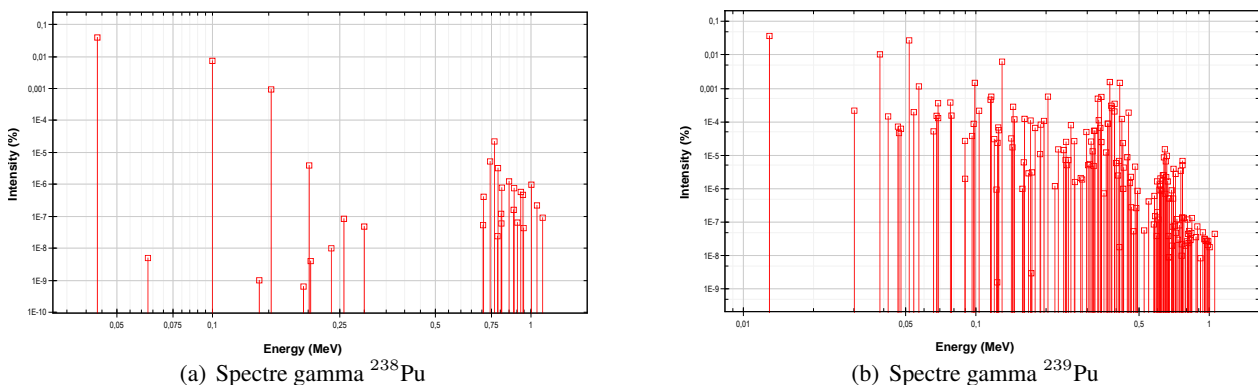
FIGURE 1.41 – Spectre \gamma du plutonium [7].
