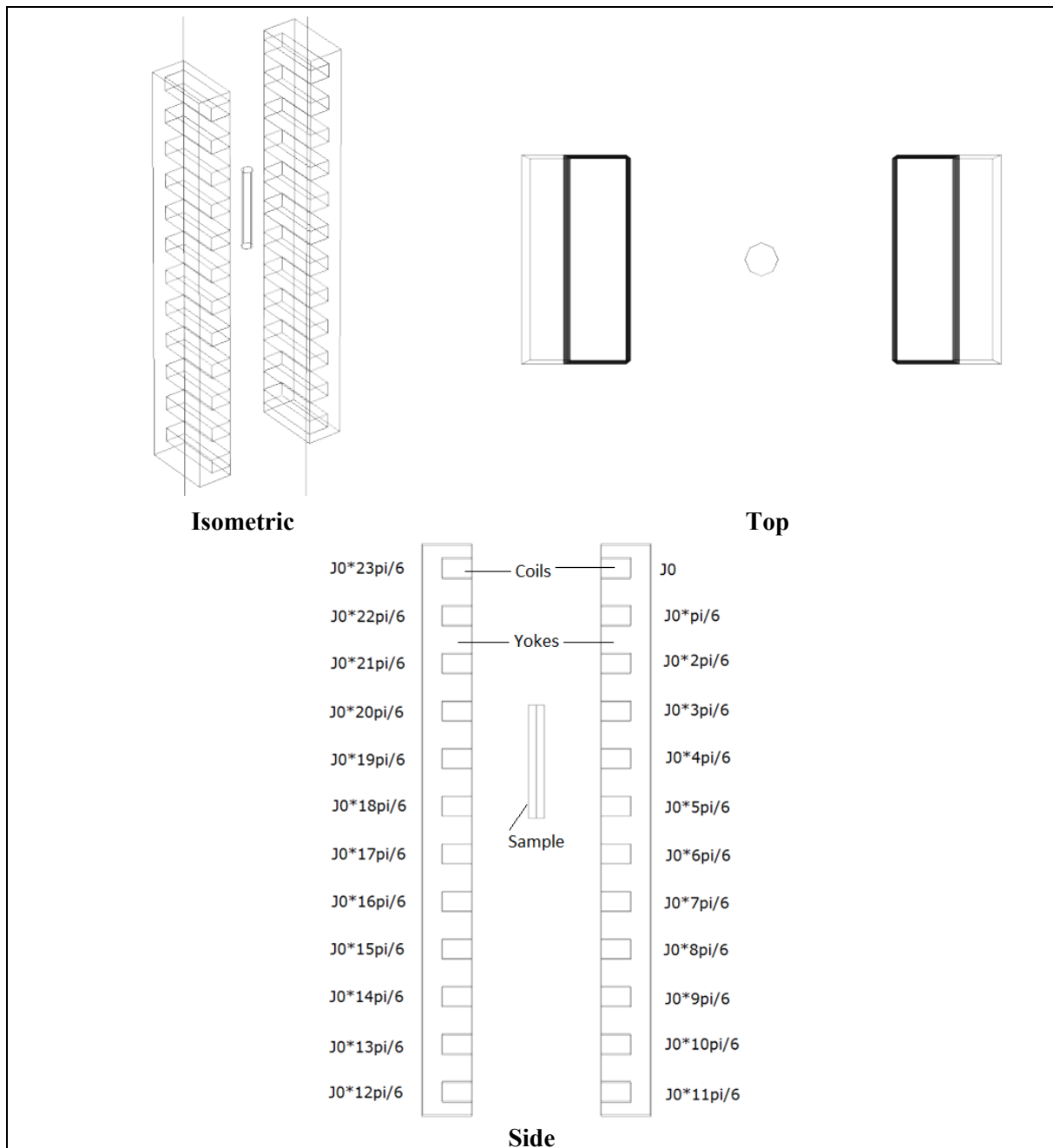
Figure 4.19 The geometry of the electromagnetic simulations on TMF including the phases of alimantation
