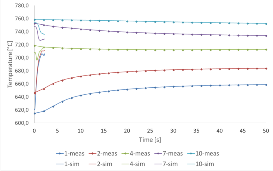
Figure 4.32 First gradient shift result – 40 mT
