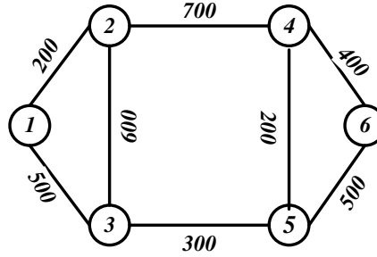
Figure 3.6: Six-node network [16]
