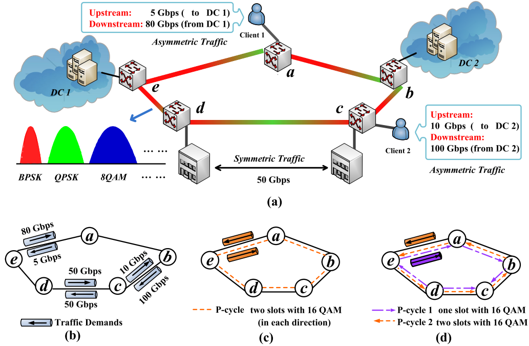
Figure 3.2: (a) Symmetric and asymmetric services in EONs. (b) The traffic demands. (c) Undirected p -cycle protection. (d) Directed p -cycle protection.
