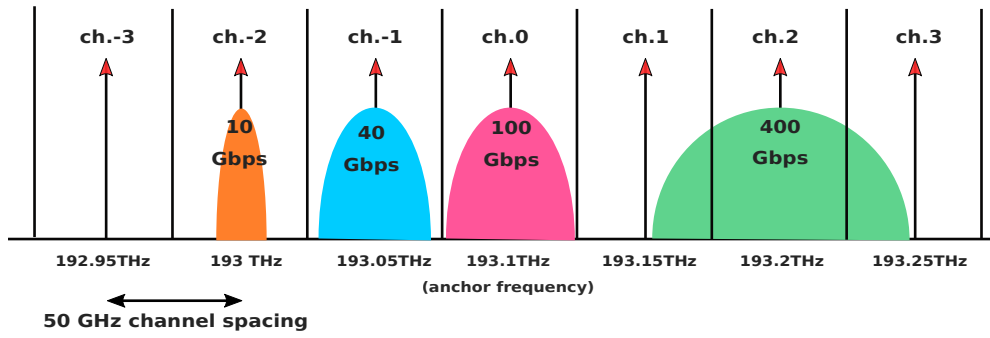
Figure 1.3: ITU-T fixed-grid [117].
