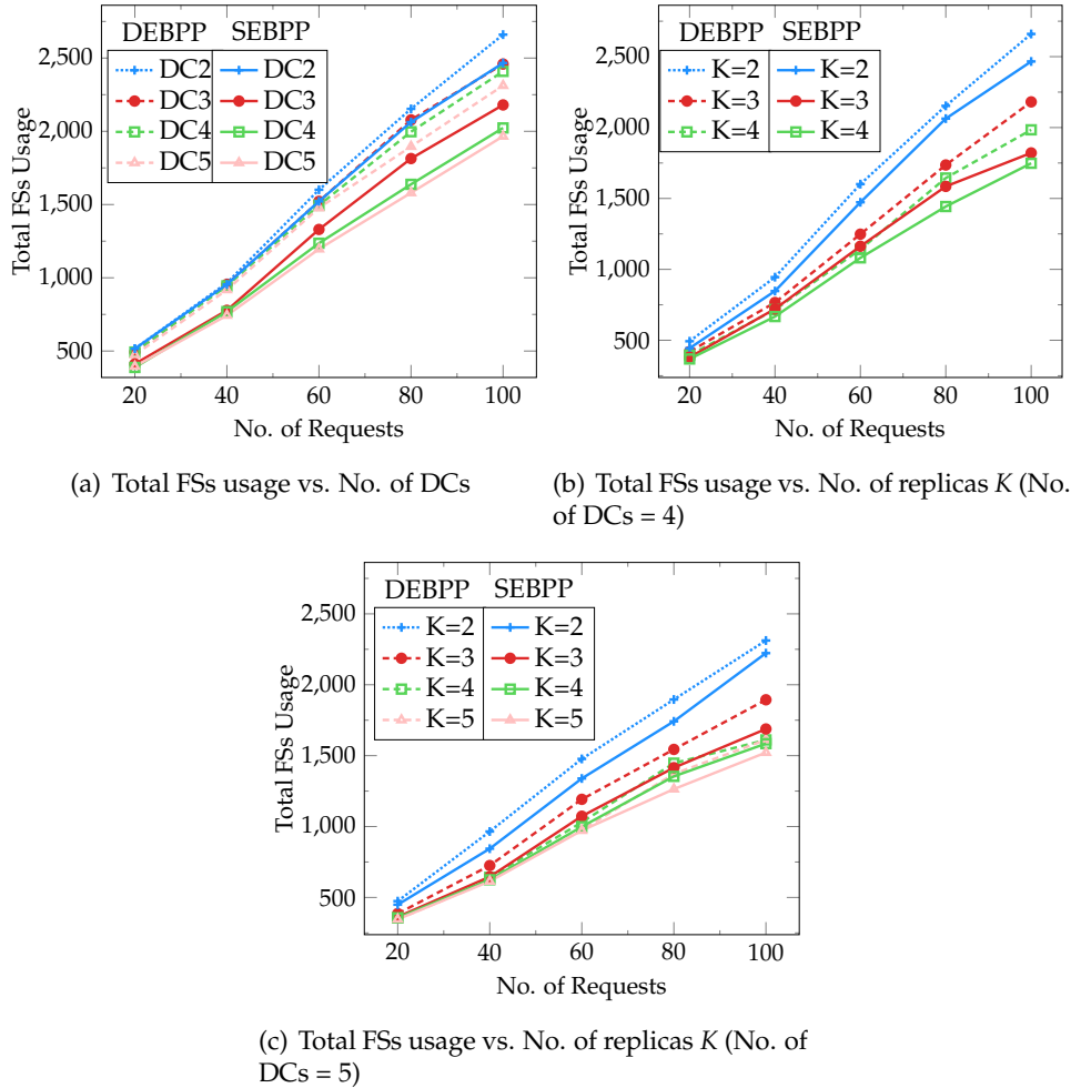
Figure 5.6: Total FSs usage of DEBPP and SEBPP for different No. of DCs and No. of replicas in NSFNET network.
