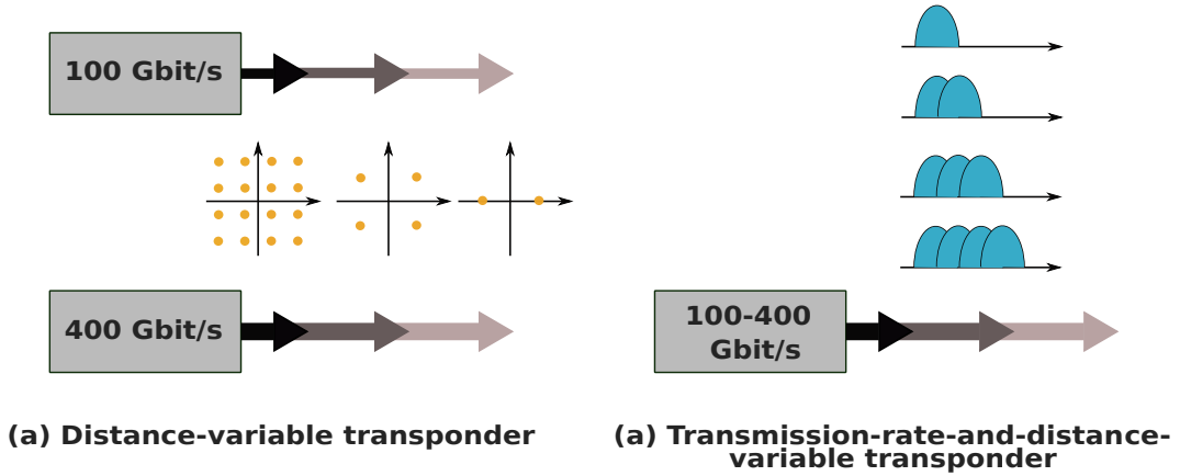
Figure 1.8: BVT [92].
