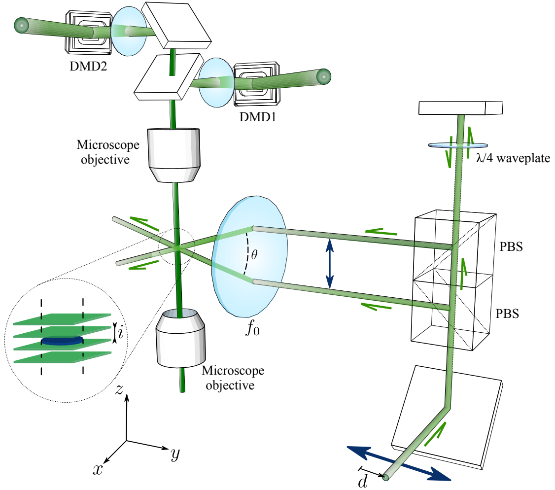
Figure 2.3 – Schematic view of the whole final trapping setup.
