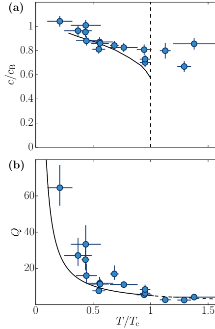
Figure 8.4 – Speed of sound and quality factor. (a) Measured speed of sound c normalized to c_B . The vertical dashed line shows the position of the critical point. The solid line shows the result from the two-fluid hydrodynamic model applied to the 2D Bose gas [75]. A fit to the data points below T_c by this hydrodynamic model with a free multiplicative factor shows that the measurements are globally 3% above the theoretical prediction. This could correspond to a 6% systematic error in the calibration of n_{2D} used to determine c_B \propto n_{2D}^{1/2} . Our estimated uncertainty on n_{2D} is on the order of 11% (see section 8.4.3) and our measurements are thus compatible with the predicted value of the speed of second sound c_{HD}^{(2)} . (b) Quality factor Q = 2\omega/\Gamma of the lowest-energy mode. The solid line is the prediction for Landau damping [265] (continued as a dashed line for T > T_c ). For both graphs, the error bars represent the statistical uncertainty extracted from the fitting procedures used to determine c , \Gamma and T/T_c .
