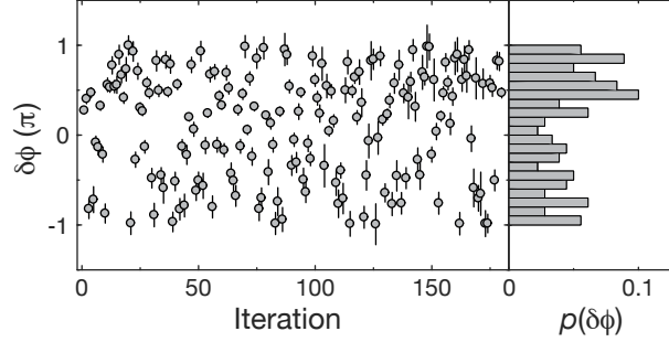
Figure 6.7 – Relative phase between the two ring-shaped condensates. The relative phases \delta\phi were evaluated using the data displayed in Fig. 6.3(a) for N = 1 and restricting the analysis to images with \nu = 0 . The results are shown in the left panel. The corresponding histogram displaying the binned probabilities p(\delta\phi) is depicted in the right panel.
