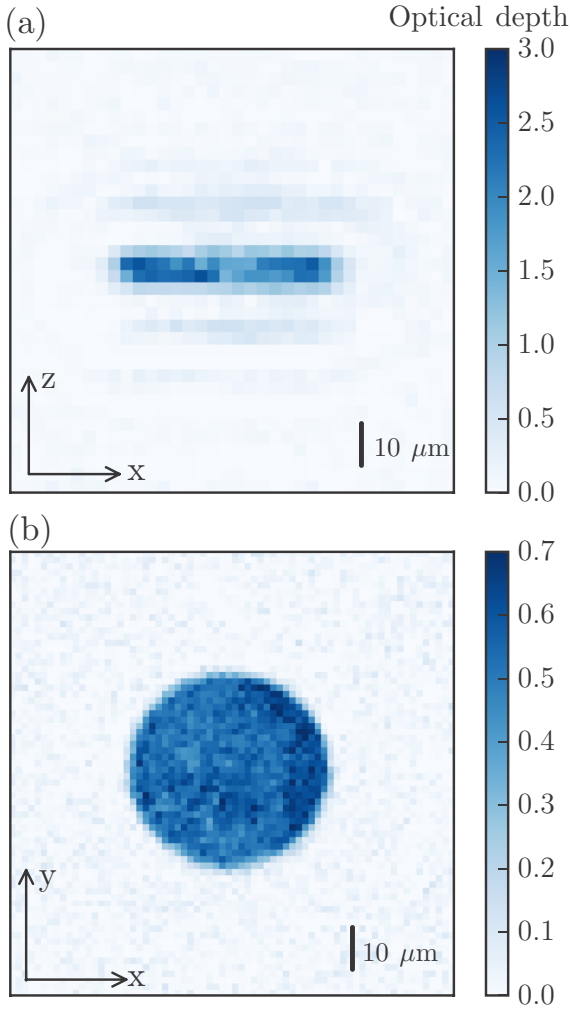
FIG. 4. In situ absorption images of the trapped cloud before compression with \omega_z/2\pi = 2.1 kHz and T = 800 nK. The cloud diameter is 40\ \mu\text{m} . To avoid saturation of the absorption signal, we transfer, using a microwave field, only a small fraction of the 10^5 atoms from the F = 1 state to the F = 2 state before imaging atoms in F = 2 . (a) Side view (transferred fraction: 100%, average of five pictures). The weak signals above and below the main cloud are fringes due to the propagation of light through our dense sample. We have checked that their position is independent of the lattice spacing of the accordion lattice. (b) Top view (transferred fraction: 2.4%, average of 35 pictures).
