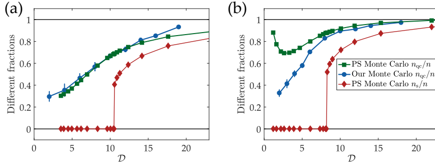
Figure 1.6 – Computed superfluid and quasi-condensed fractions of the gas for \tilde{g} = 0.1 in (a) and \tilde{g} = 0.01 in (b). The green squares correspond to the quasi-condensate fraction computed by Prokof'ev and Svitsunov, and the blue disks to the results of our simulations. The red diamonds correspond to the superfluid fraction computed by Prokof'ev and Svitsunov.
