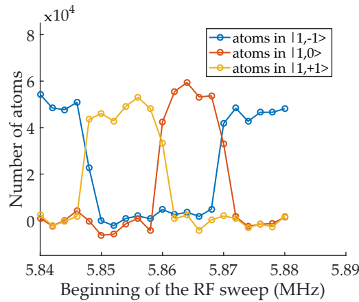
Figure 2.10 – Number of atoms in the different Zeeman states after the RF sweep for different starting frequencies
