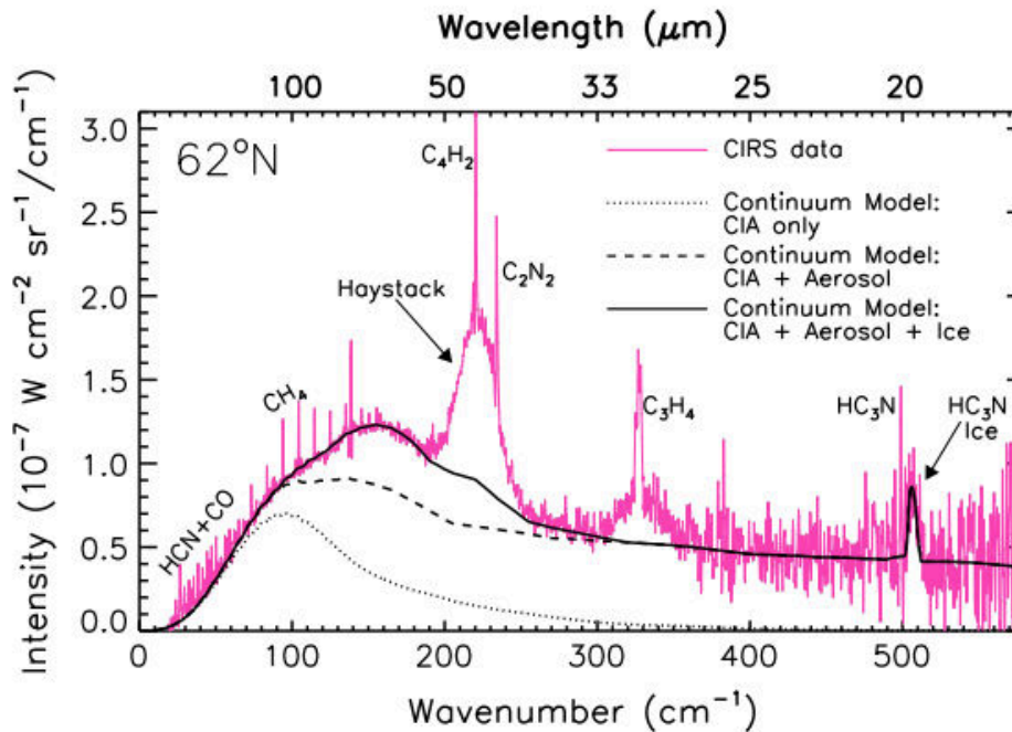
FIGURE 1.21: CIRS limb spectrum (pink) at a 0.48 \text{ cm}^{-1} spectral resolution, at a limb tangent height of \sim 125 \text{ km} (Anderson et al., 2014). The broad haystack feature at 220 \text{ cm}^{-1} is attributed to an ice cloud absorption, potentially nitrile-rich.
