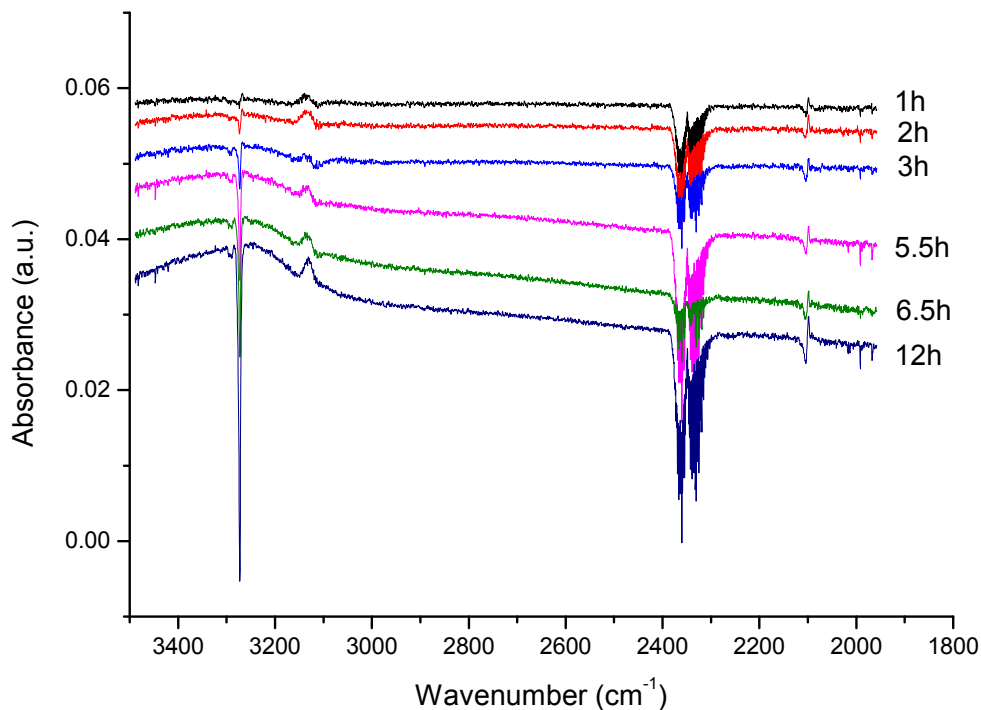
FIGURE 5.19: 12h of accumulated irradiation. The C 4 H 2 consumption at 3272 cm -1 is clearly visible. HCN is marked by a consumption of both the CN and CH bands.
