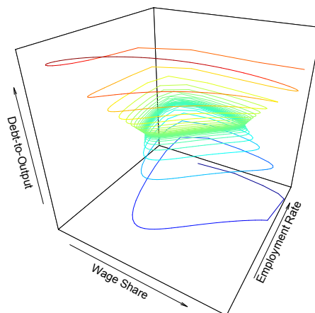
FIGURE 4.7: Simulation of a trajectory towards the bad equilibrium with the calibration of Appendix C.2 and \eta = 500 . The initial condition of the system is (\omega, \lambda, d) = (0.80558764045, 0.9719722, 1.4995533) , which corresponds to the darkest blue point.
