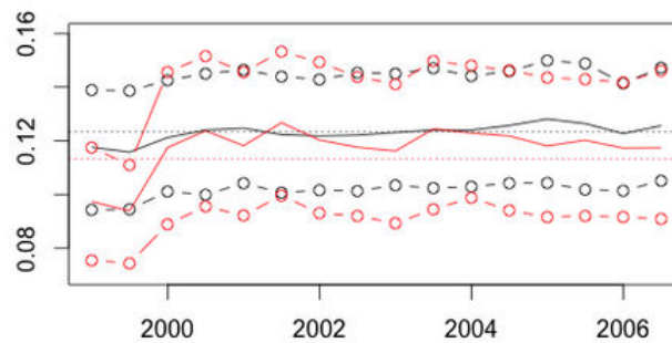
FIGURE 2.6: The Evolution of \hat{\alpha}_e from 1999:Q1 to 2006:Q3 in Bi-annual Frequency.
