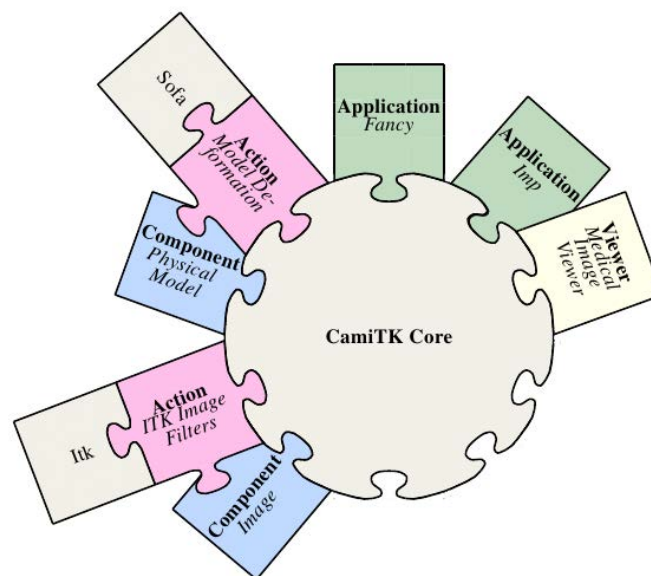
Figure 4.13 - CamiTK architecture with several collaborating modules Source: http://camitk.imag.fr
