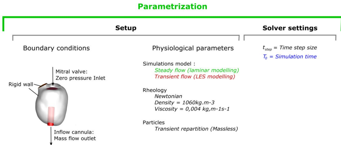
Figure 5.4 - CFD simulation settings parametrization
