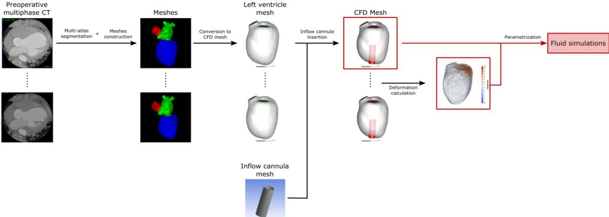
Figure 5.22 - Flowchart for the elaboration of heart beating simulation with a LVAD inflow cannula
