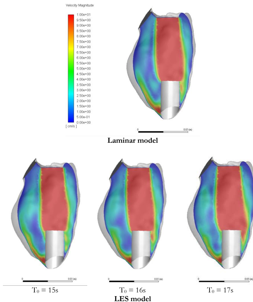
Figure 5.7 - Comparison of the velocity magnitude from the laminar to the LES model
