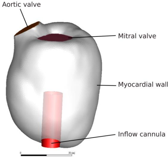
Figure 5.3 - Left ventricular CFD geometry with a LVAD inflow cannula
