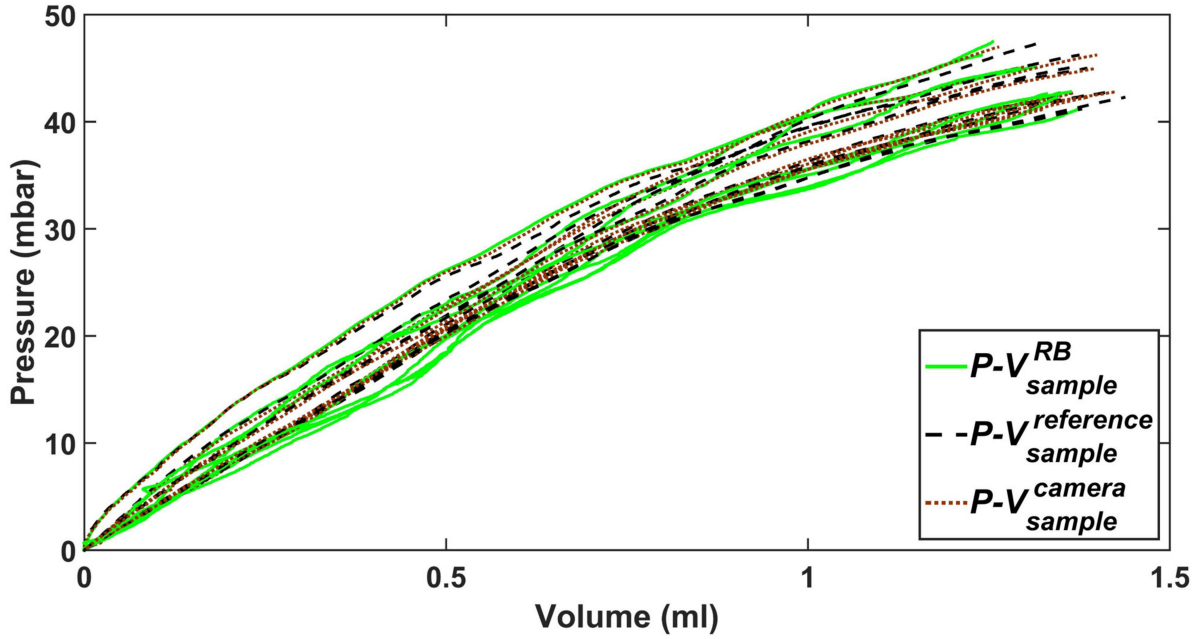
Figure 2.6: Comparison of 9 diagrams of pressure P versus measured aspirated volume using rate-based V_{sample}^{RB} , reference V_{sample}^{reference} and camera V_{sample}^{camera} methods for the test group VT-1.
