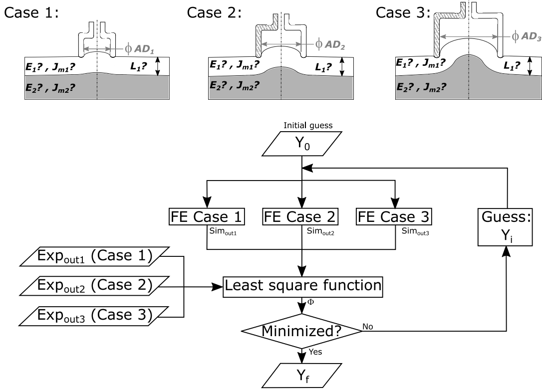
Figure 4.2: Schematic representation of the optimization process for the inverse characterization of the materials parameters and the superficial layer thickness, using aspiration tests with three aperture diameters AD_j . Y are the set of the unknown parameters (here the thickness of the superficial layer L_1 and the Gent constitutive parameters of the two materials E_1, J_{m1}, E_2 and J_{m2} ).
