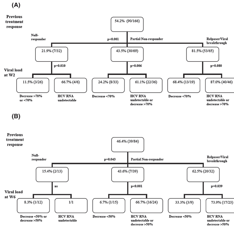
Figure 2 Decision tree giving the proportion of patients achieving SVR12 according to previous treatment response and viral load at week 2/week 6. In each box, the probability of achieving SVR12 is given. Figures slightly differ from the total number of cases since only patients with information on previous treatment response are included. A. Telaprevir-treated patients. B. Boceprevir-treated patients.
