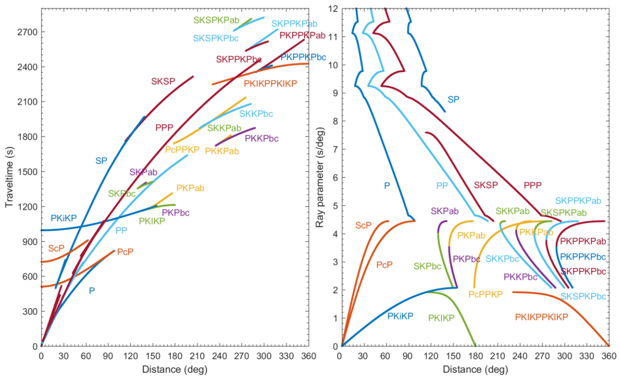
Figure 3.4. Theoretical curves of traveltimes and ray parameters for typical seismic body phases, predicted by the Taup program base on the IASP91 model.
