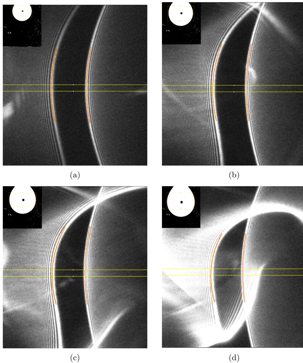
Figure 5.4: Images of pendant drops and their scattering pattern near rainbow angle. The region between two yellow line is the equatorial region selected. The yellow and red curve along the rainbow pattern are respectively the outline extracted and curve fitted for the main peak of rainbow.
