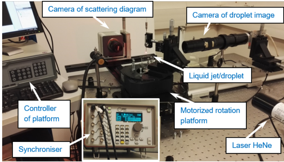
Figure 5.1: Experimental setup
