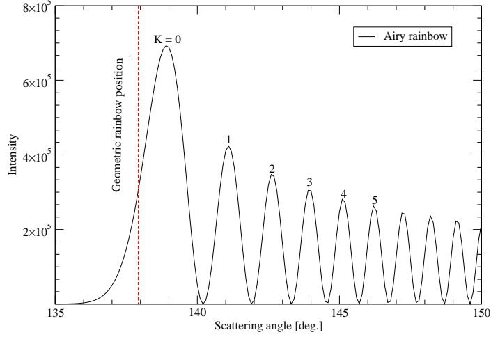
Figure 2.6: Intensity distribution calculated by Airy theory for a sphere of refractive index m = 1.333 and radius a = 50 \mu\text{m}
