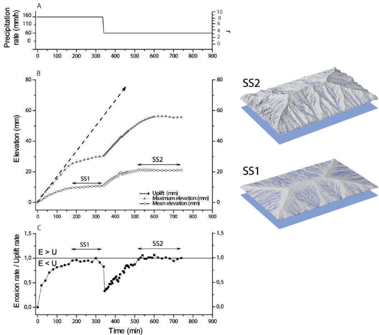
Figure 1 : Evolution of a typical experiment (Experiment MOD2) forced by an instant drop ( T_p=0 ) in precipitation rate. (A) Precipitation applied and corresponding water-to-rock-ratio ( r ). (B) Evolution of the mean and maximum elevation. The dotted line indicated the amount of applied uplift, that is, elevation of the model if no erosion occurred. Periods of constant mean and maximum elevations indicate steady-state (erosion rate=uplift rate) (C) Evolution of mean erosion rate ( E ) of the landscape calculated from mass balance. Erosion rates are normalized to the uplift rate ( U ). Periods of normalized uplift rates of 1 correspond to steady-state. Two examples of steady-state landscapes (SS1 and SS2) are shown on the right (3D view of DEMs; size 60 \times 40 cm).
