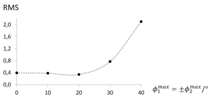
Figure 3.48. RMS value as a function of \phi_1^{max} = \pm\phi_2^{max} calculated for t -St in PBLG/THF- d_8 by the AP-DPD approach while fixing A_{C_2} = 0.6 and h_1 = 10 . The curve is also drawn as eye-guide.
