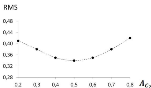
Figure 3.47. RMS value as a function of probability ratio A_{C_2} calculated for t -St in PBLG/THF- d_8 by the AP-DPD approach while fixing \phi_1^{max} = 16.80 and h_1 = 10 . The curve is also drawn as eye-guide.
