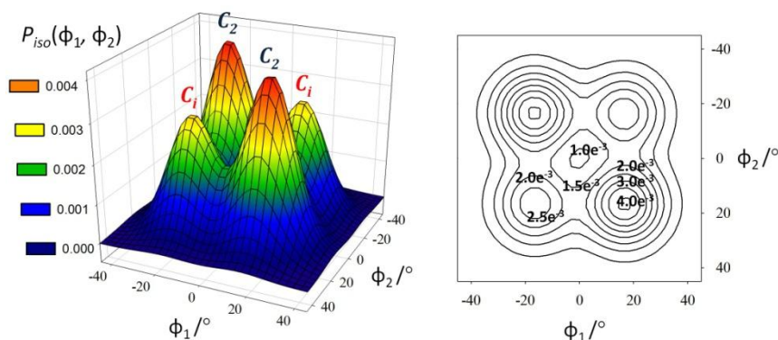
Figure 3.41. Experimental probability distribution P_{iso}(\phi_1, \phi_2) for t -St dissolved in the nematic solvent ZLI1132 at 298 K, obtained by the liquid crystal NMR conformational analysis (both the 3D surface and its contour plot are shown).
