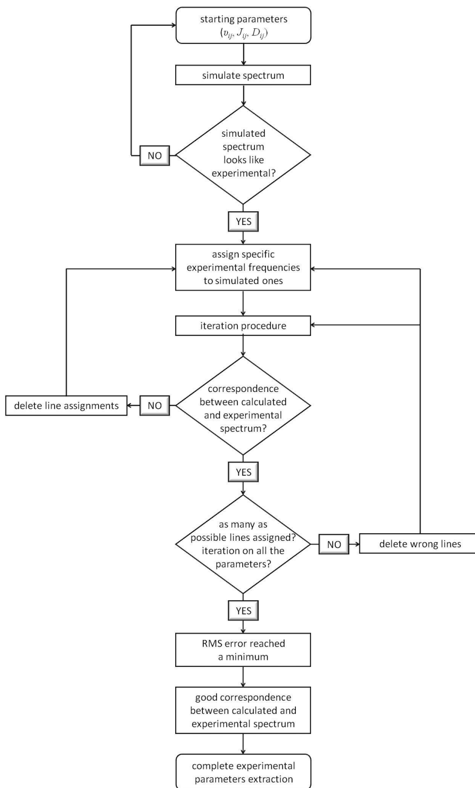
Figure 1.13. Flowchart showing the strategy adopted for analysis of the NMR spectra of oriented molecules.
