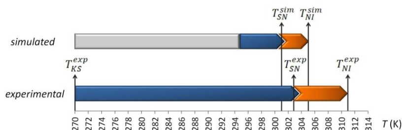
Figure 3.4. Comparison between simulated and experimental transition temperatures for 8CB with 2P as solute. Nematic and smectic ranges are in orange and blue, respectively. Gray area represents the temperature range not considered in MD simulations.
