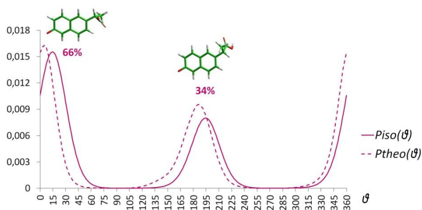
Figure 3.32. Experimental (solid line) and theoretical (dashed line) torsional probability distributions as a function of \vartheta obtained for S -naproxen respectively by the AP-DPD approach and from B3LYP/6-31G** calculations.
