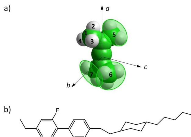
Figure 2.1. (a) “Balls” structure, atomic labeling and molecular frame of the D_{2d} symmetry tetramethylallene (TMA) and (b) topological structure of the liquid crystal I52.
