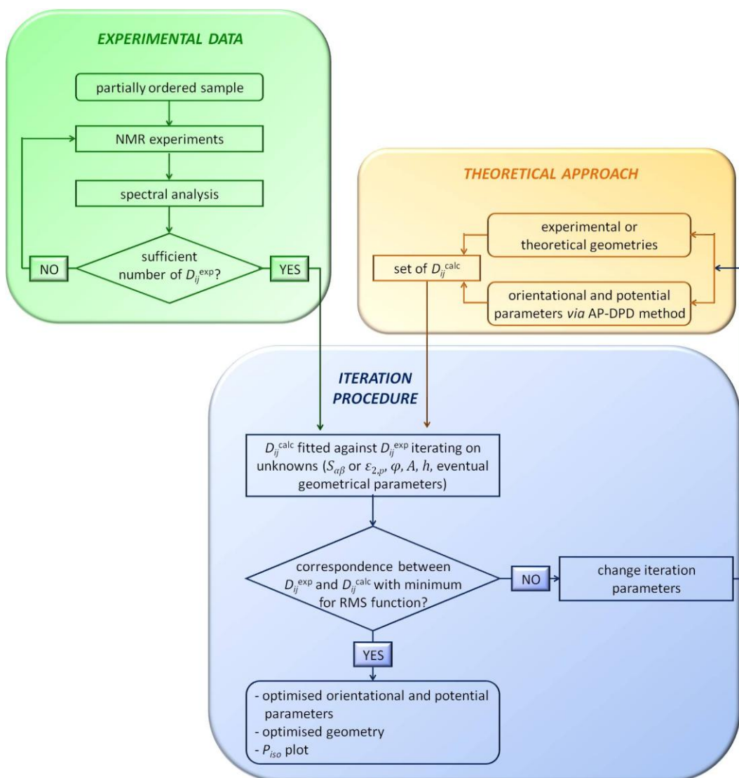
Figure 1.14. Flowchart showing the whole analytical strategy adopted for structural, orientational and conformational studies of partially ordered molecules.
