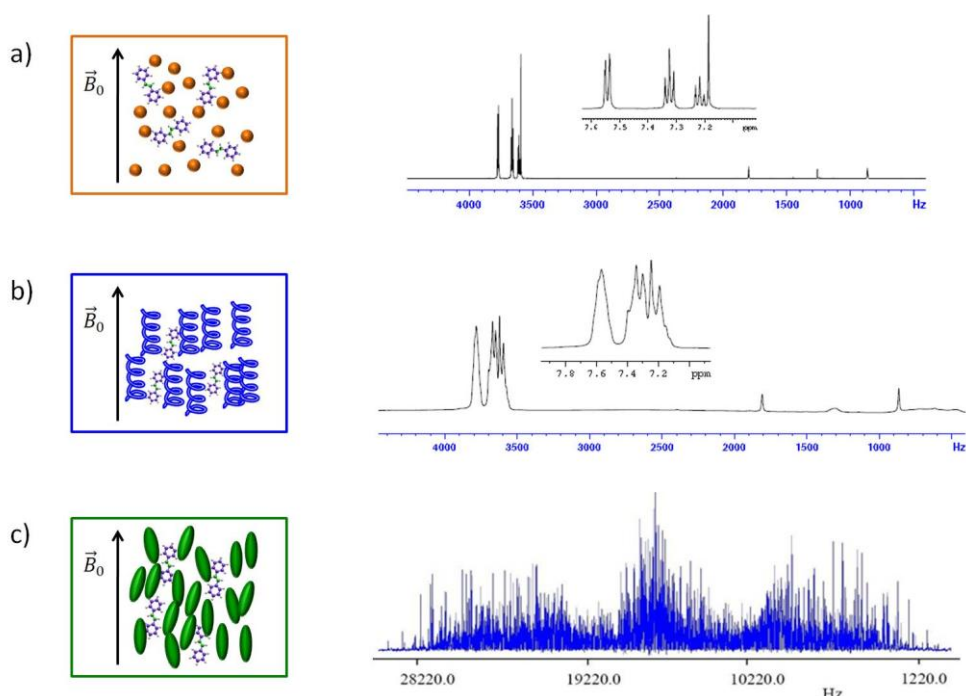
Figure 1.12. SQ ^1\text{H} spectra of trans -stilbene dissolved in (a) THF- d_8 , (b) PBLG/ THF- d_8 mixture and (c) ZLI1132.
