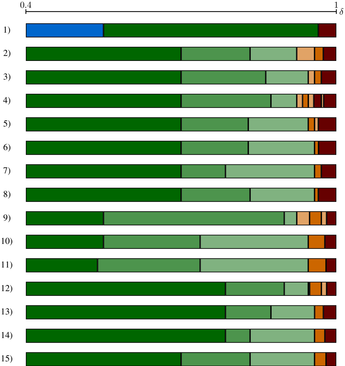
Figure 2.13: Duration of all 15 cases with T = 5 and R = \frac{3}{2} .
