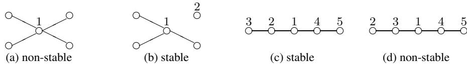
Figure 3.12: Examples with \delta > \left(\frac{1}{2}\right)^{\frac{1}{2}} , where players 1 and 2 have the same items.
