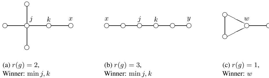
Figure 3.4: Not pairwise stable networks for \delta \leq \frac{1}{2} .
