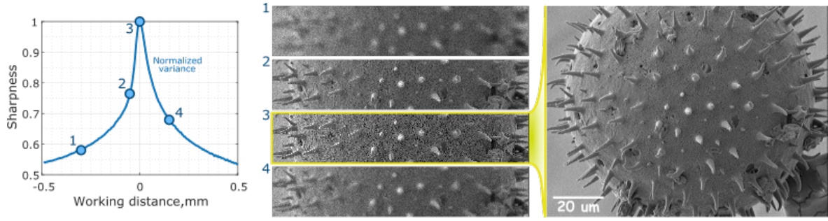
Figure 5.1: Left: sharpness function for a pollen grain of daisy flower ( Bellis Perrenis ). Middle: image ROIs for points in sharpness function. Right: in-focus image that corresponds to point 3 on sharpness function. Magnification: \times 1000 .
