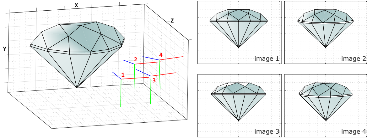
Figure 3.4: Four images of diamond sequence with 3D view. Cameras are represented by local coordinate axes.
