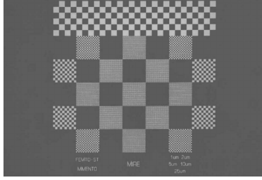
Figure 1.9: Multi-scale calibration target for SEM, square size from 1 \mu\text{m} up to 25 \mu\text{m} .
