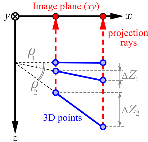
Figure 2.7: Bas-relief ambiguity.
