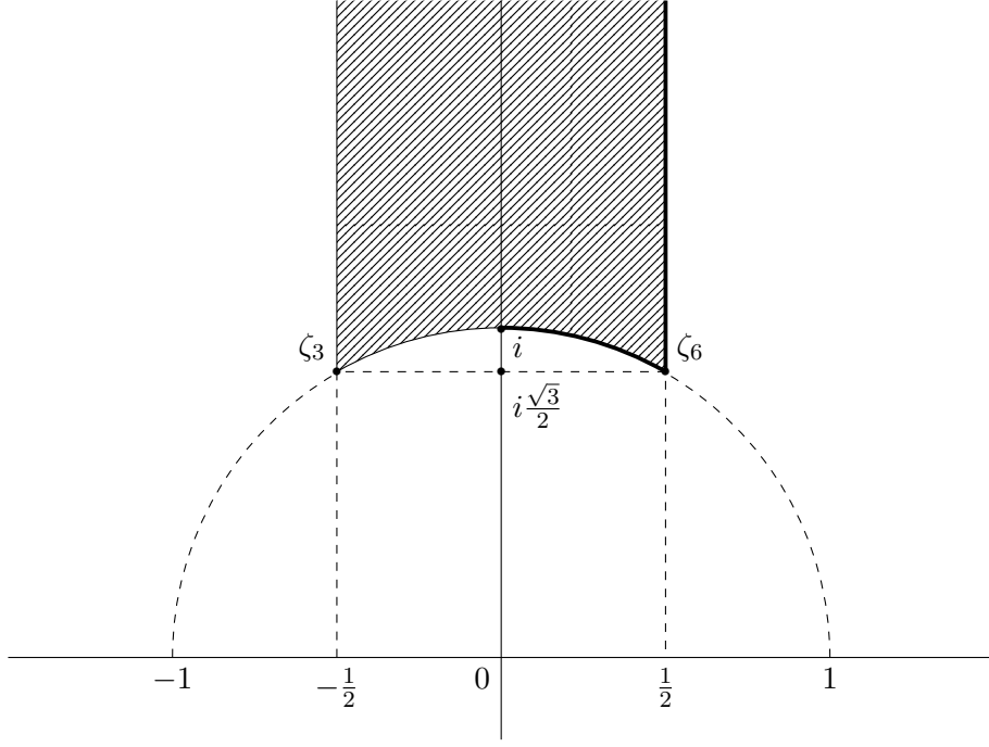
FIGURE B.1 – Domaine fondamental \mathcal{D}
