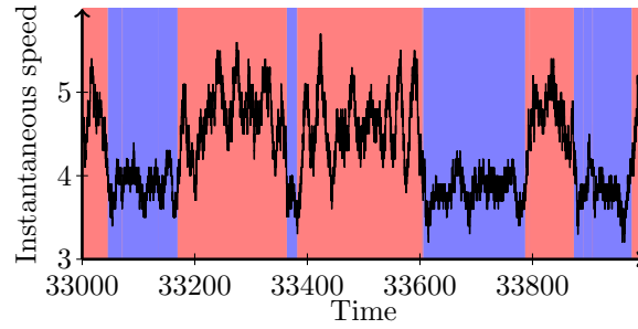
Figure 3.9 – Instantaneous speed of the front of the epidemic across time. The underlying color indicates which pathogen genotype is present at the edge of the front: the wild type (blue) or the mutant (red). This corresponds to a single run of a stochastic simulation of the epidemic spread. Default parameter values: \beta_w = 5 , \alpha_w = 1 , r_w = 4.0 , R_{0,w} = 5.0 , \beta_m = 50 , \alpha_m = 40 , r_m = 10.0 , R_{0,m} = 1.25 , \mu_w = \mu_m = 0.01 , N = 550 , \sigma = 1 , h = 1 . The criterion we used to determine which genotype dominates at the edge is based on their relative abundance in the first three occupied cells. The speed is the shifting speed averaged in a small period of time (5 units). Notice that since the simulations are done in continuous time, there is no discretization step. The unit of time is thus arbitrary, but common to all the simulations: it corresponds to the average life-time of a wild type infection (i.e. \alpha_w = 1 in all our simulations).
