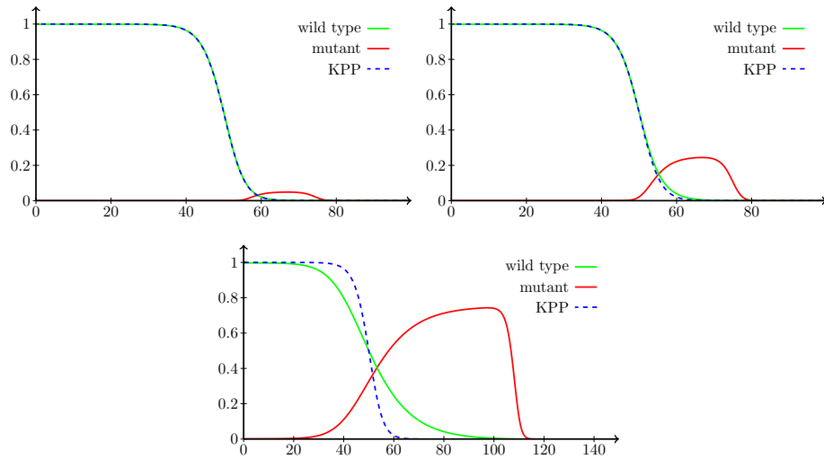
Figure 2.2 – Comparison of the travelling wave solutions of (2.2) and the travelling wave solution of the Fisher-KPP equation of (non-minimal) speed 2\sqrt{r} . These figures are obtained for r = 2 , \mu = 0.001 , and three values of K : K = 0.05, 0.25, 0.75 . We see that the agreement between the density of the wild type ( w , green line) and the corresponding solution of the Fisher-KPP equation ( u , dashed blue line) is good as soon as K \leq 0.25 . The travelling waves solutions of (2.2) are obtained numerically as long-time solutions of (2.2) (based on an explicit Euler scheme), while the travelling waves solutions of the Fisher-KPP equations (for the given speed 2\sqrt{r} that is not the minimal travelling speed for the Fisher-KPP model) is obtained thanks to a phase-plane approach, with a classical ODE numerical solver.
