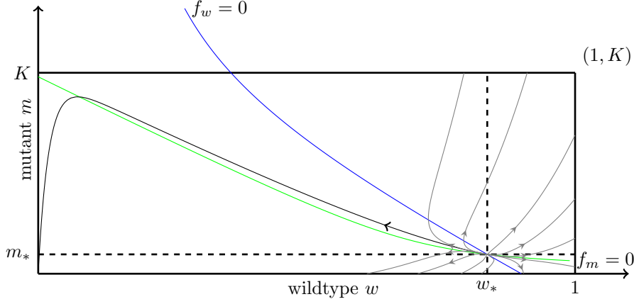
Figure 2.3 – Phase-plane-type representation of a solution of (2.7): we represent (dark line) x \mapsto (w(x), m(x)) \in [0, 1] \times [0, K] . Note that the usual phase-plane for (2.7) is of dimension 4. The blue line represents the set of (w, m) such that f^w(w, m) = 0 (see (2.4)), f^w(w, m) > 0 for (m, w) on the left of the blue curve. The green line represents the set of (w, m) such that f^m(w, m) = 0 (see (2.4)), f^m(w, m) > 0 for (m, w) under the green curve. The gray lines represent several other solutions of (2.3) such (w(-a), m(-a)) = (w^*, m^*) . The dashed dark lines separate this phase plane into four compartments that will be used in the third step of the proof of Lemma 2.4.1. Finally, the solid black line corresponds to the travelling wave.
