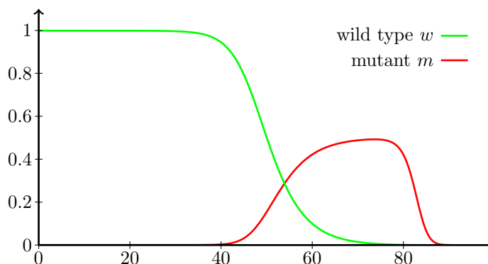
Figure 2.1 – Numerical simulation of (2.2) with r = 2 , K = 0.5 , \mu = 0.01 , with a heaviside initial condition for w and null initial condition for m . The numerical code is based on an implicit Euler scheme. For large times, the solution seems to converge to a travelling wave, that we represent here, propagating towards large x . In the initial phase of the epidemics, the mutant ( m , red line) population is dominant, but this mutant population is then quickly replaced by a population almost exclusively composed of wild types ( w , green line). Although the steady states on the back of the wave seems to be close to (w(x), m(x)) = (1, 0) , we actually know that (w^*, m^*) \in (0, 1) \times (0, K) .
