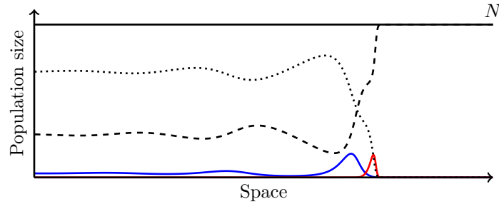
Figure 3.8 – Shape of the stationary solution for a SIR scenario. We use an SIR model in which infected hosts I_w (resp. I_m ) acquire immunity at rate \gamma_w (resp. \gamma_m ) and any recovered host loses immunity at rate \theta . The number of recovered hosts is also shown (black dotted curve). Parameters : \beta_w = 2.0 , \alpha_w = 0.05 , \gamma_w = 0.5 , r_w = 1.45 , \mu_w = 0.01 , R_{0,w} = 3.64 , \beta_m = 10.0 , \alpha_m = 6.0 , \gamma_m = 1.0 , r_m = 3.0 , \mu_m = 0.01 , R_{0,m} = 1.43 , \theta = 0.02 , \sigma = 1.0 .
