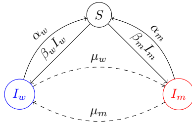
Figure 3.1 – Schematic representation of the pathogen life cycle. Arrows represent the transitions between states. The label indicate the rates at which those transitions occur.
