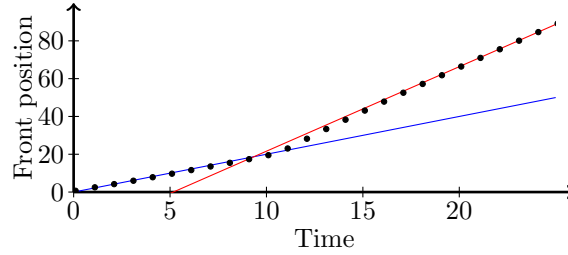
Figure 3.6 – Position of the front with respect to time. The black dots represent the location where the wild type population reaches half its carrying capacity (ie. w = 1/2 ), measured on a numeric computation of Equation (3.1). The initial population that we have considered is composed of only a non-zero population of wild type pathogens located at the origin, while no mutant pathogen are present: (w, m) = (\delta_0, 0) on the box [0, 500] . We used the parameters \sigma = 1 , r_w = 1 , r_m = 5 , K_w = 1 , K_m = 0.25 , \mu_w = 10^{-6} , \mu_m = 0.01 , and the spatial steps \Delta t = 0.01 , \Delta x = 0.01 . The blue and red lines have a respective constant velocity of 2\sqrt{\sigma r_w} and c^* \sim 2\sqrt{\sigma r_m} . We have introduced an important asymmetry between \mu_w and \mu_m to improve the readability of the figure.
