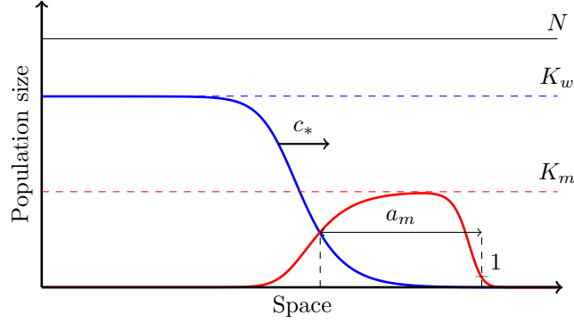
Figure 3.2 – Shape of the stationary front of the spreading epidemic. The epidemic moves at a constant speed c^* . The mutant genotype (in red) is prevalent at the edge of the front and reaches a maximal density of K_m . Behind the front, the wild type genotype (in blue) takes over and reaches a higher density K_w . The size of the area where the mutant is more abundant than the wild type is called the mutant's range, a_m .
