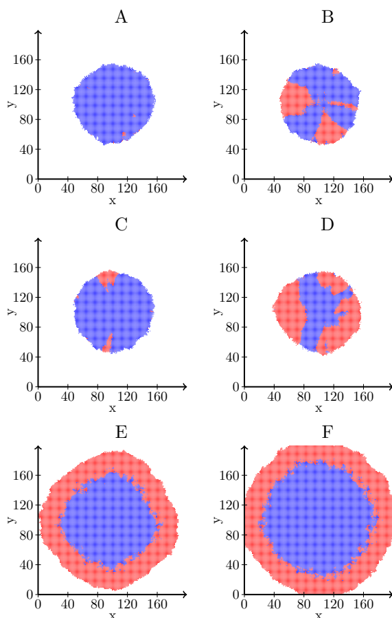
Figure 3.5 – Stochastic simulations of the spread of an epidemic in 2 dimensions ( x and y ). At the beginning of the simulation the pathogen population starts as a disk of radius 6.3 cells. In A, C and E the simulation starts from an initial condition where only the wild type is present. In B, D and F the simulation starts from a mixed pathogen population where the wild type and the mutant are equally frequent. In the first row (A and B) the wild type and the mutant have the same parameter values (neutral selection scenario). In the second row (C and D) the mutant is slightly more virulent than the wild type (weak selection scenario). In the third row the mutant is very different from the wild type (strong selection scenario). The actual parameters we used can be found in the SI (section 12).
