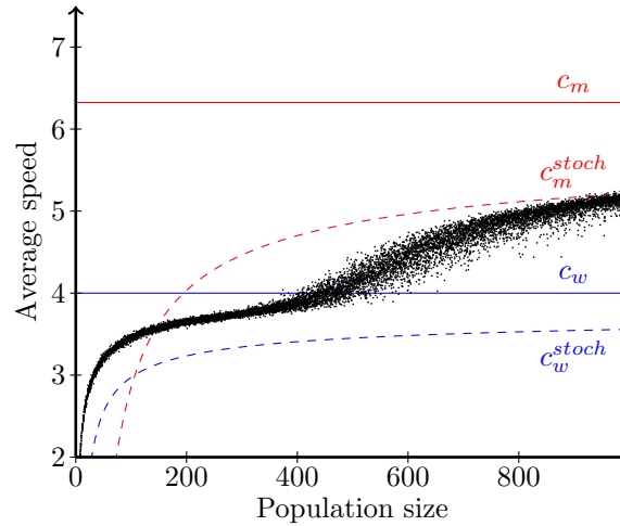
Figure 3.4 – Effect of host population size N on the average speed of the stochastic epidemic. 100 simulations were done for each value of N and each dot represents the average epidemic speed for a single simulation, taken between time t = 200 and t = 1000 .
