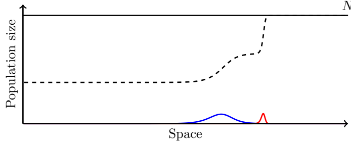
Figure 3.7 – Shape of the stationary solution for a SI scenario with host demography. Hosts are not allowed to reproduce and host death is only induced by the infection. The number of susceptible hosts is also shown (black dashed curve). For clarity, we multiplied the population size of the mutant and wild type strains by 5. Parameters : \beta_w = 10.0 , \alpha_w = 5.0 , r_w = 5.0 , \mu_w = 0.01 , R_{0,w} = 2.0 , \beta_m = 50.0 , \alpha_m = 40.0 , r_m = 10.0 , \mu_m = 0.01 , R_{0,m} = 1.25 , \sigma = 1.0 .
