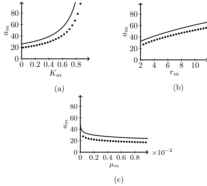
Figure 3.3 – Effects of K_m , r_m and \mu_m on the size of the mutant's range a_m in (a), (b) and (c), respectively. The full lines present the approximation given in (3.4). The dots present the mutant's range obtained from numerical simulations at time t = 500 .
