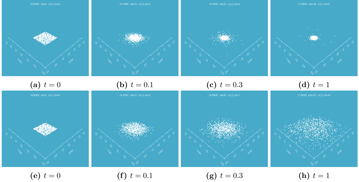
Figure 7.1: (a)-(d): \chi = 50 ; (e)-(h): \chi = 1 . Euler scheme is applied to (1.15), with N = 1000 , d = 2 . Particles are initially distributed uniformly on [-1, 1] \times [-1, 1] . Initial concentration of the chemical is a centered Gaussian density. When \chi is large an agglomeration of particles appear in the center of the domain, whilst when \chi is small the particles diffuse.
