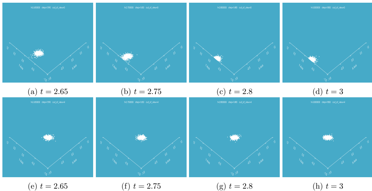
Figure 7.4: The continuation of the evolution in Figure 7.3–(a)–(d): PDPM; (e)–(h): PPPM.
