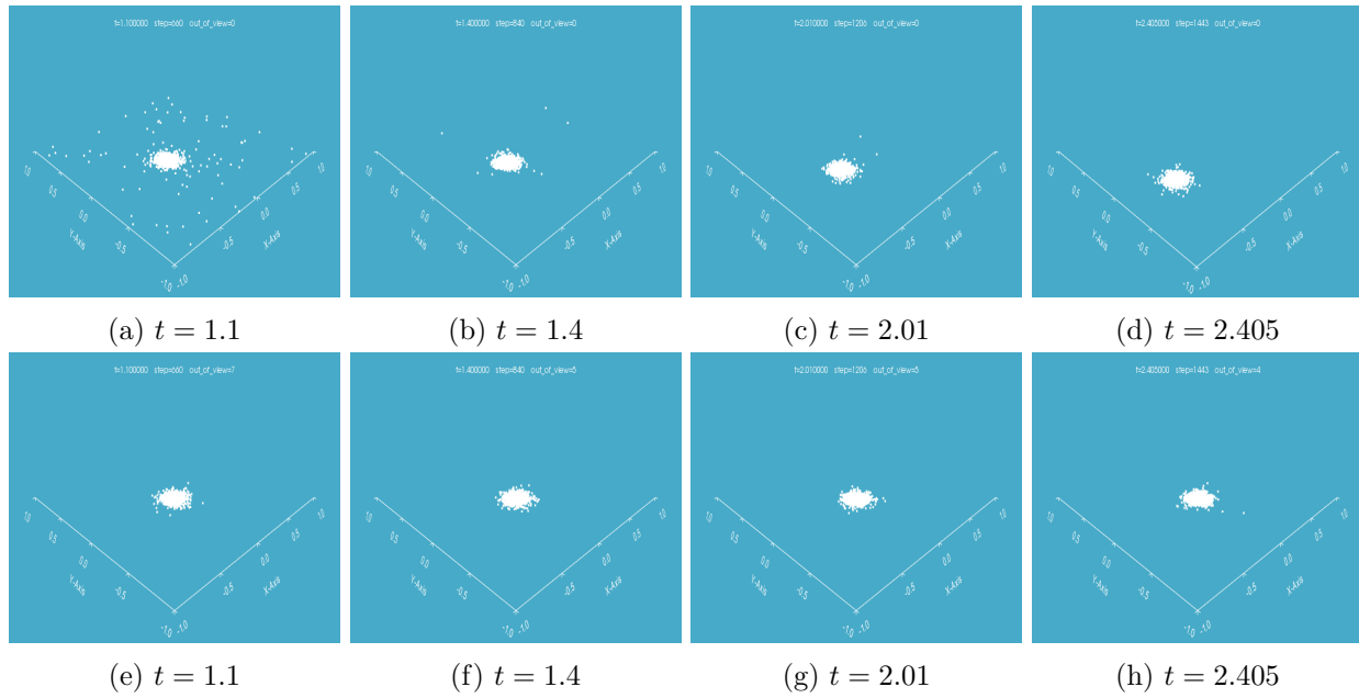
Figure 7.3: The continuation of the evolution in Figure 7.2–(a)–(d): PDPM; (e)–(h): PPPM.
