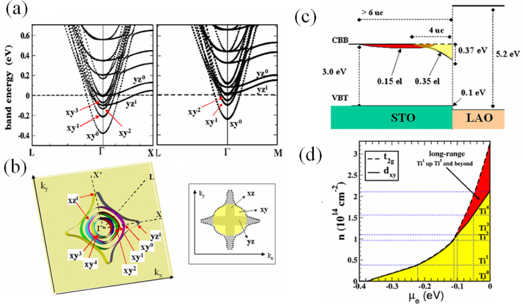
Figure 4.4: (a) Calculated energy bands for high (left) and low (right) carrier density. (b) Fermi surfaces of the 2DEG at the interface of LaAlO 3 /SrTiO 3 . (c) The band alignment of the LaAlO 3 /SrTiO 3 and calculated distribution of the d_{xy} , d_{xz} , d_{yz} orbitals. Electrons in d_{xy} are confined closer to the interface, while the d_{xz} , d_{yz} electron wavefunctions extend up to the sixth STO layer below the interface. (d) Calculated t_{2g} (dashed) and d_{xy} (solid) charge densities per unit area as a function of chemical potential. Extracted from [Delugas 2011].
