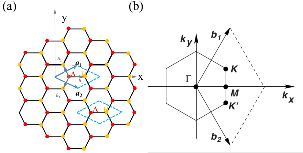
Figure 3.2: (a) Honeycomb lattice of graphene. The vectors \delta_1 , \delta_2 , and \delta_3 connect the nearest-neighbors (NN) carbon atoms, separated by a distance a=0.142 nm. The vectors a_1 and a_2 are basis vectors of the triangular Bravais lattice. (b) Reciprocal lattice of the triangular lattice. The primitive lattice vectors are b_1 and b_2 . The first Brillouin zone (BZ) is characterized by its center \Gamma and the two inequivalent corners K and K'. Extracted from [Castro Neto 2009, Mousavi 2014].
