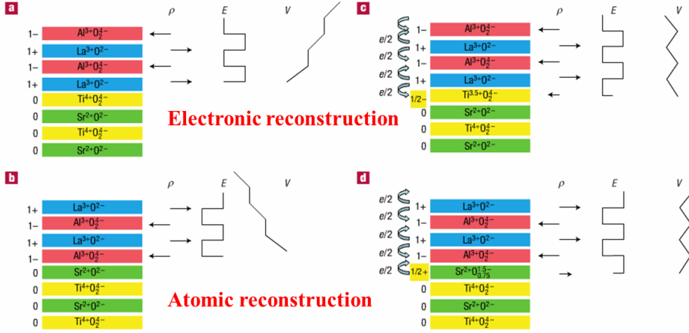
Figure 4.2: The polar catastrophe model at atomically abrupt LAO and STO interfaces along (001) direction. (a,b) are n- and p-type interfaces before reconstruction, respectively. (c,d) are corresponding interfaces after reconstruction. Because the Ti ions have multivalence, the electronic reconstruction is possible in the \text{LaO}/\text{TiO}_2 interface, while the atomic reconstruction is the only option for the \text{AlO}_2/\text{SrO} interface. The electronic reconstruction in the \text{LaO}/\text{TiO}_2 interface induces the 2DEG and the conducting properties whereas the atomic reconstruction brings in an insulating \text{AlO}_2/\text{SrO} interface. Extracted from [Nakagawa 2006].
