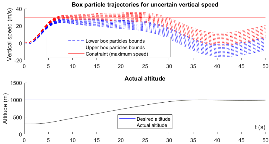
Figure 6.6: Box particle trajectories for the \dot{h} dimension and actual altitude (open loop).
