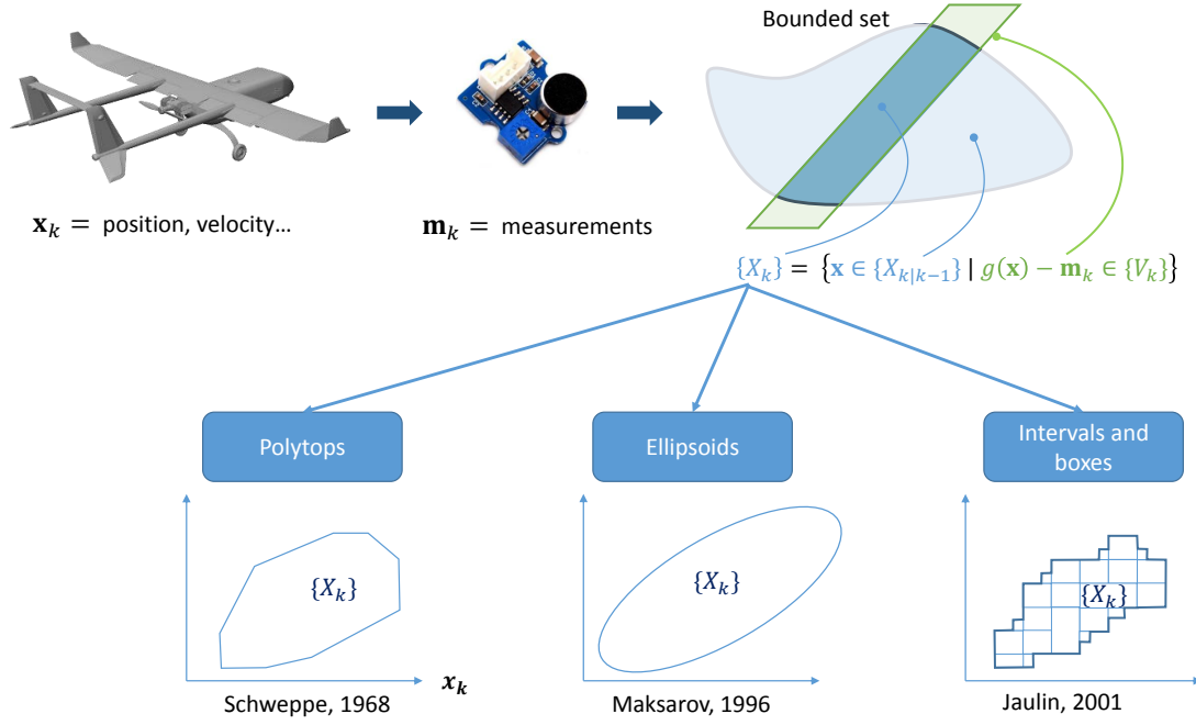
Figure 2.9: Set-based estimation scheme and three different state set approaches: Polytopes, ellipsoids, and paving of intervals, or boxes in the multidimensional case
