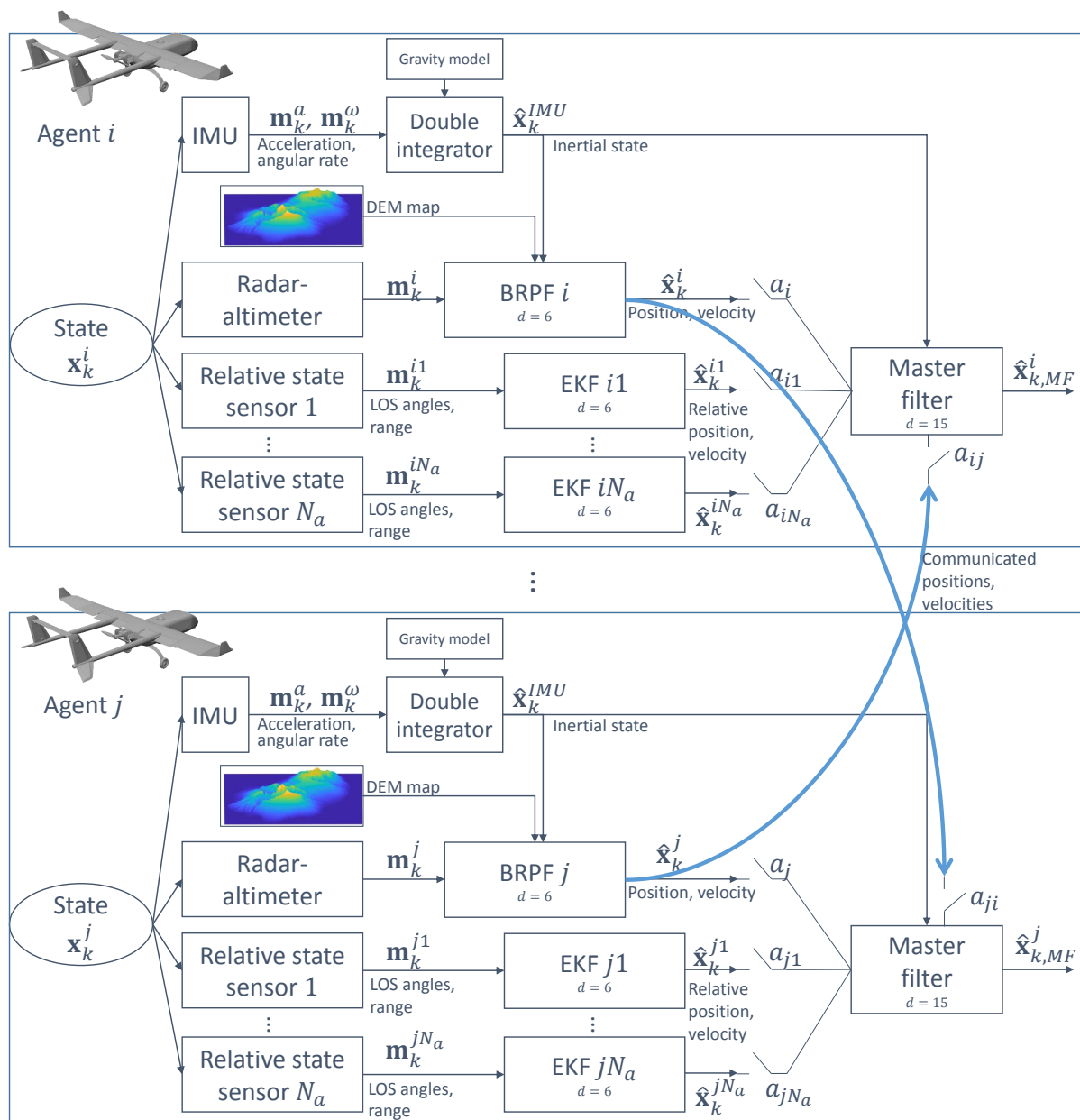
Figure 5.13: BRPF integrated to a distributed federated architecture in the context of IMU hybridisation with TAN, relative measurements, and communicated BRPF estimates. Two agents i and j among the N_a vehicles are represented, with j \neq i . Local absolute measurements \mathbf{m}_k^i are obtained from a radar altimeter, local relative measurements \mathbf{m}_k^{ij} ( j \neq i ) are Line Of Sight (LOS) angles and range, and communicated information are BRPF estimates \hat{\mathbf{x}}_k^i . The BRPF is assumed to run with a 6-dimensional IMU hybridisation model. The N_a - 1 relative EKF filters run with a 6-dimensional relative state model. The Master Filter runs with a 15-dimensional IMU hybridisation model and fuses local filters outputs in a linear way.
