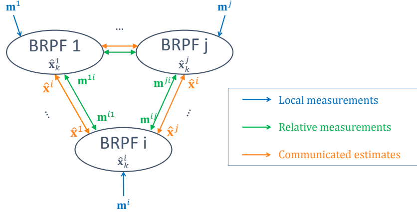
Figure 5.10: Collaborative estimation scheme: each system i uses a BRPF to estimate its own state \mathbf{x}_k^i from its local measurements \mathbf{m}_k^i . In order to improve its estimation quality, it is allowed to exchange its estimate \hat{\mathbf{x}}_k^i with its connected neighbors (e.g. j ) and to get some relative measurements \mathbf{m}_k^{ij} .
