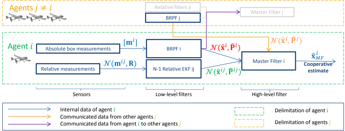
Figure 5.11: Two stages fusion architecture for distributed BRPF: each agent i gets its local measurement box [\mathbf{m}_k^i] . A first estimate \hat{\mathbf{x}}_k^i is done by the BRPF. Simultaneously, an Extended Kalman Filter provides an estimation of the relative states \hat{\mathbf{x}}_k^i using the relative measurements \mathbf{m}_k^{ij} . Then, the Master Filter fuses a unimodal approximation of the own state estimate, the relative estimates, and unimodal approximations of the communicated states in a linear way.
