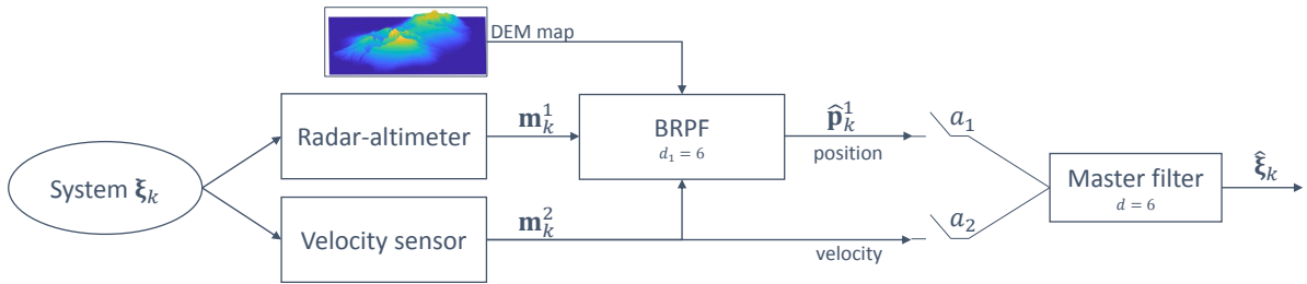
Figure 5.5: Box Regularised Particle Filter integrated to a federated architecture. BRPF tackles the ambiguous and non-linear TAN problem and provides a position estimate to the Gaussian Master Filter (e.g. Kalman Filter). The Master Filter estimates the whole state vector (position, measurement) from the BRPF's position estimation under Gaussian asymptotic hypothesis and the Gaussian velocity measurements. The BRPF and the Master Filter use the same 6-dimensional dynamical model.
