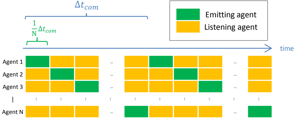
Figure 5.14: Communication protocol
