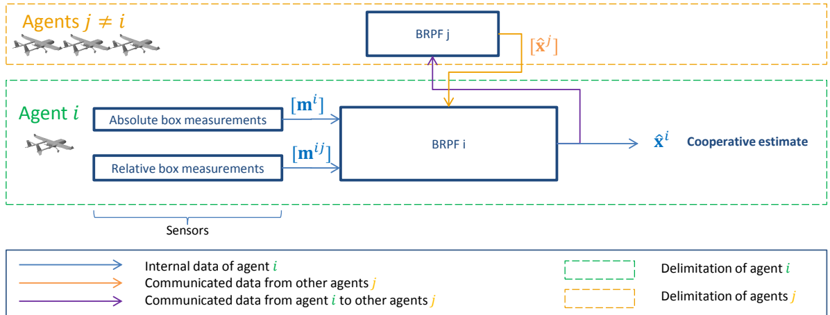
Figure 5.12: One stage fusion architecture for distributed BRPF: each agent i gets its local measurement box [\mathbf{m}_k^i] , the relative measurement boxes [\mathbf{m}_k^{ij}] with respect to other agents j \neq i , and the communicated estimation box [\hat{\mathbf{x}}_k^j] . By combining these sets, viewed as a whole measurement box, [\mathbf{m}_k^i] \times [\mathbf{m}_k^{ij}] \times [\hat{\mathbf{x}}_k^j] , the filter can improve its estimate quality. However, such a single state BRPF appears less accurate than a BRPF integrated to a federated architecture.
